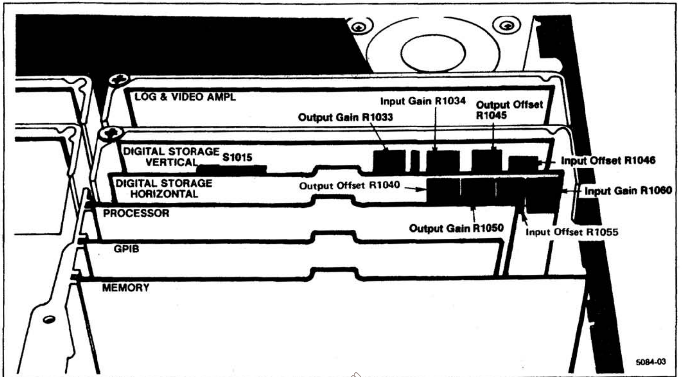
Figure 5-7. Digital storage adjustment locations.
