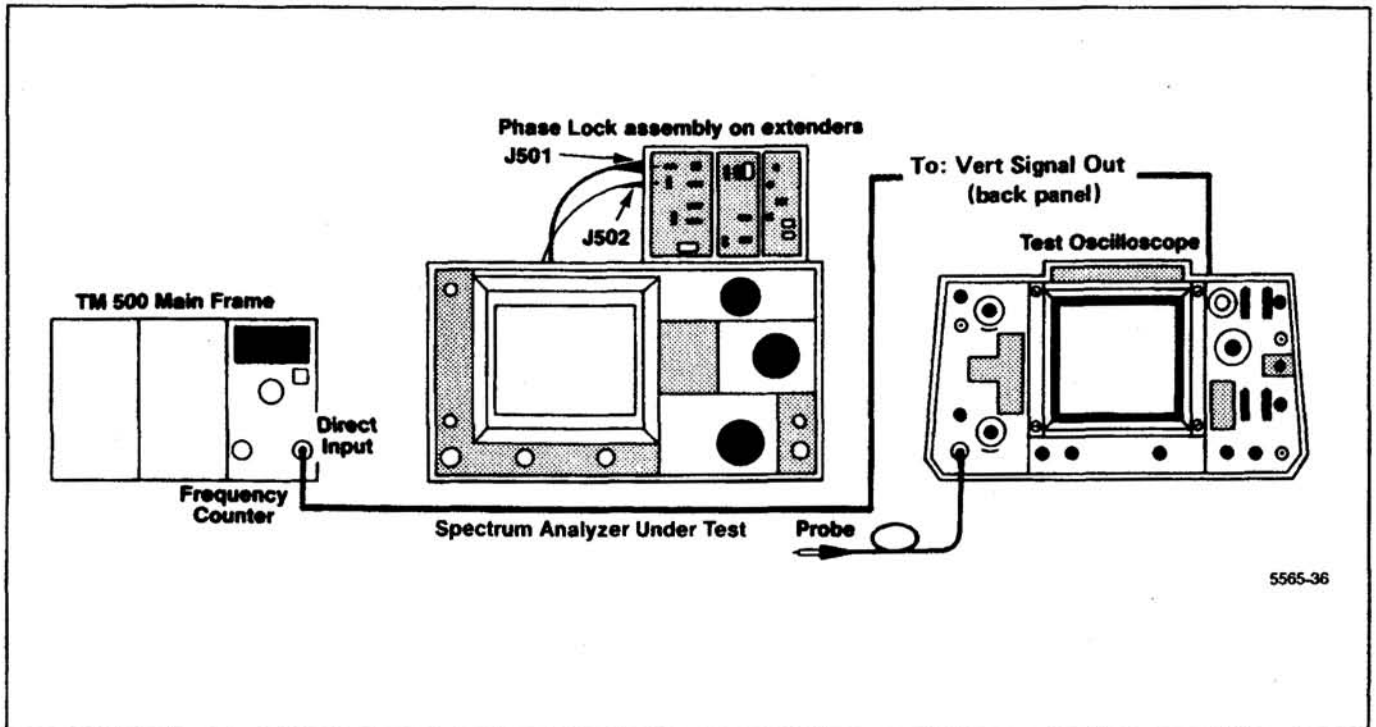
Figure 5-25. Test equipment setup for adjusting the Phase Lock assembly.
