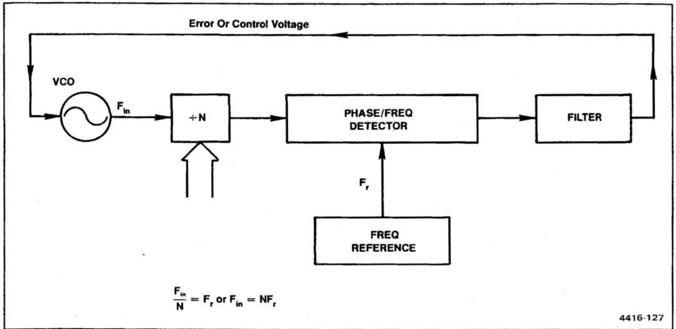
Figure 7-28. Block diagram of a basic synthesizer.
