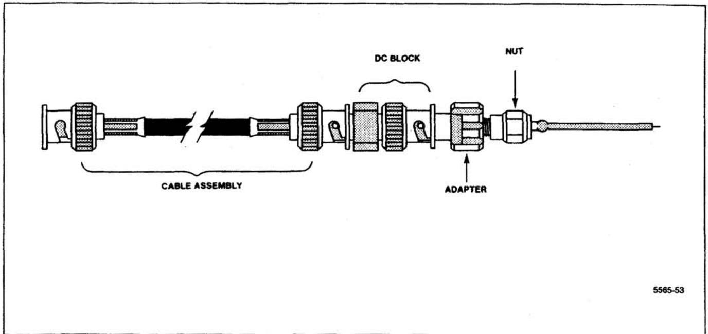
Figure 6-22. Coaxial test probe construction details.
