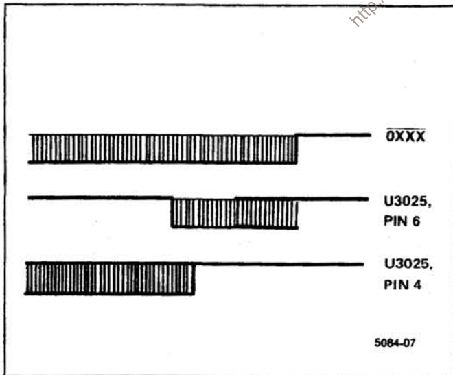
Figure 6-34. RAM select output in relation to 0XXX.
