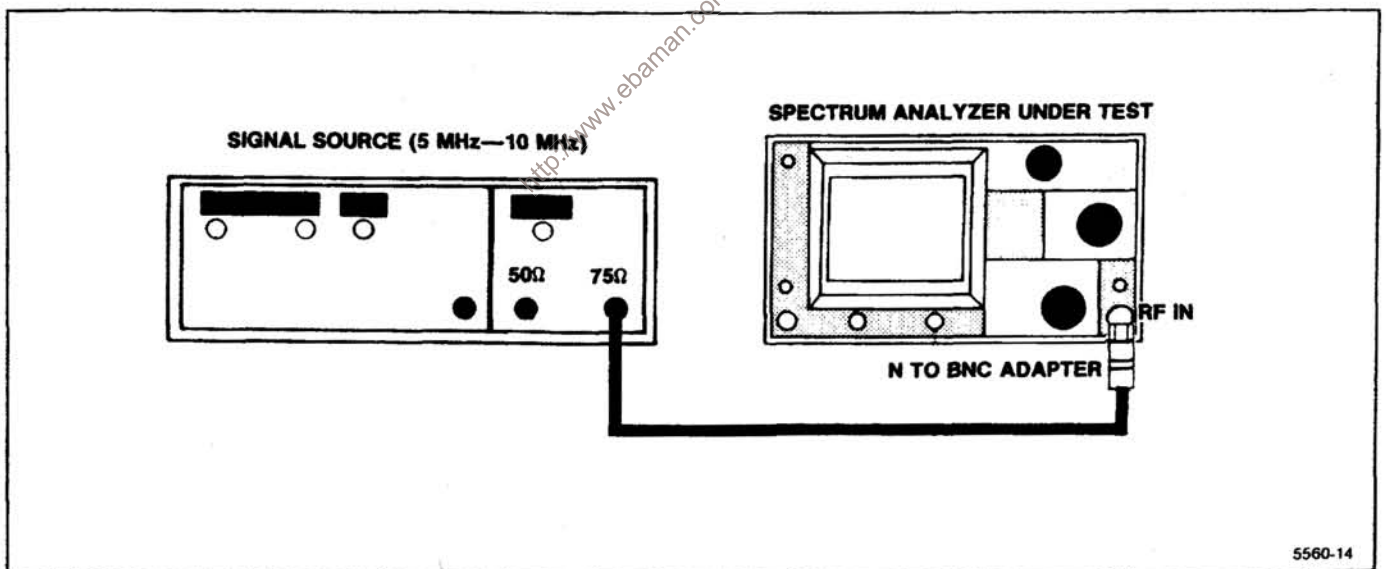
Figure 4-25. Equipment setup for checking Option 07 frequency response from 5 MHz to 10 MHz.
