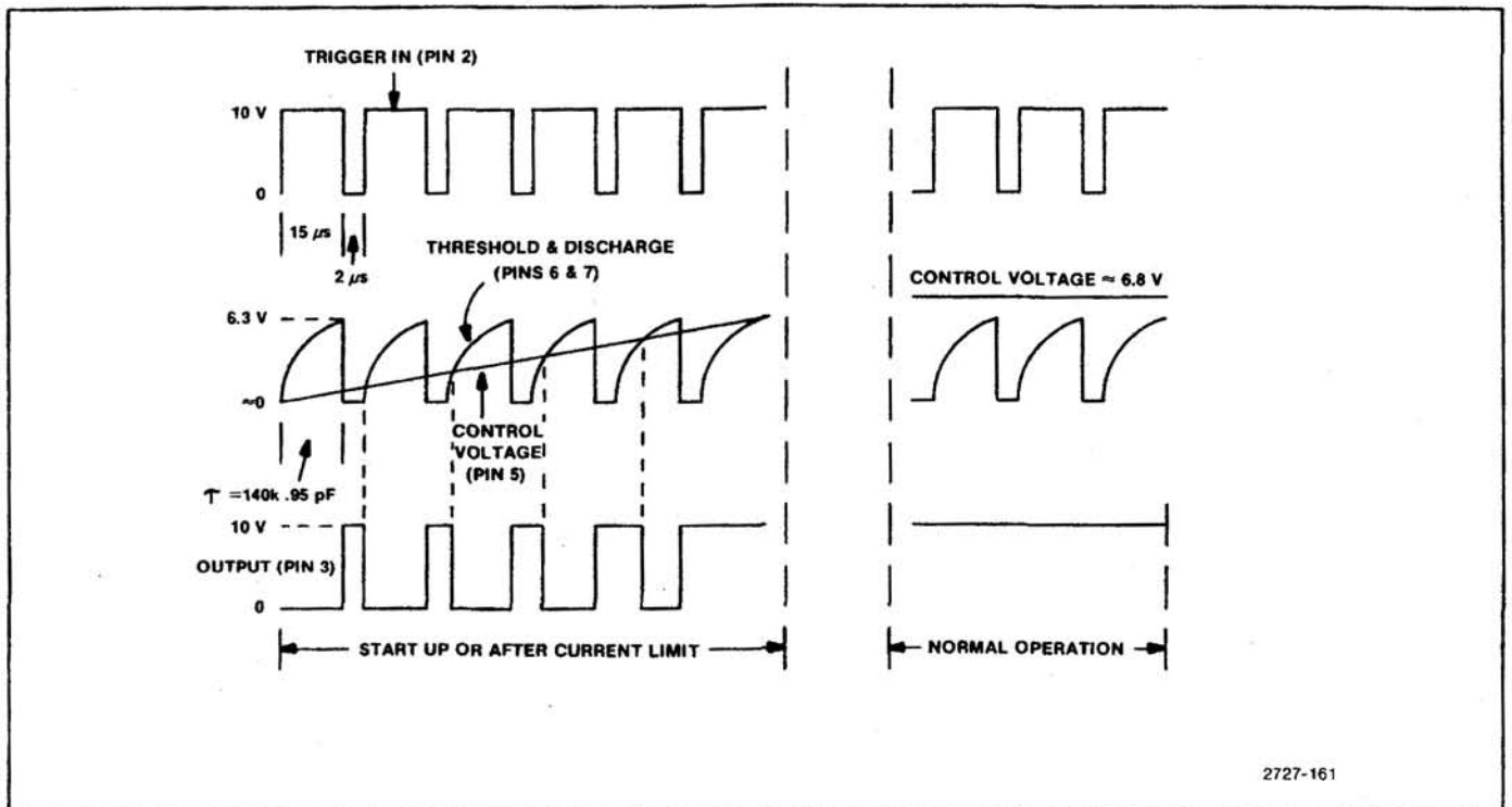
Figure 7-35. Timing waveforms for soft-start circuit.
