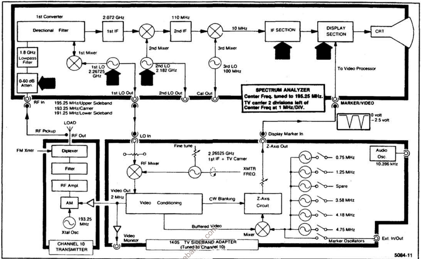
Figure 7-13. Functional diagram showing the Spectrum Analyzer and 1405 TV Sideband Adapter System.
