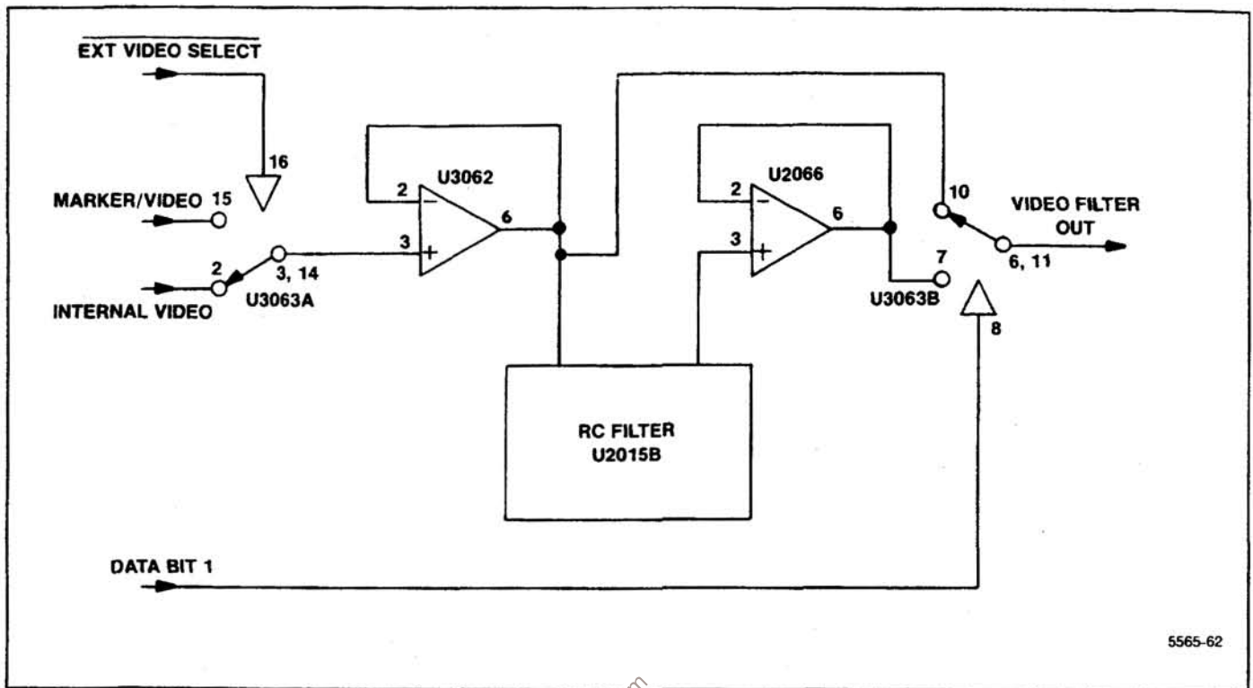
Figure 7-14. Simplified diagram of a video filter.
