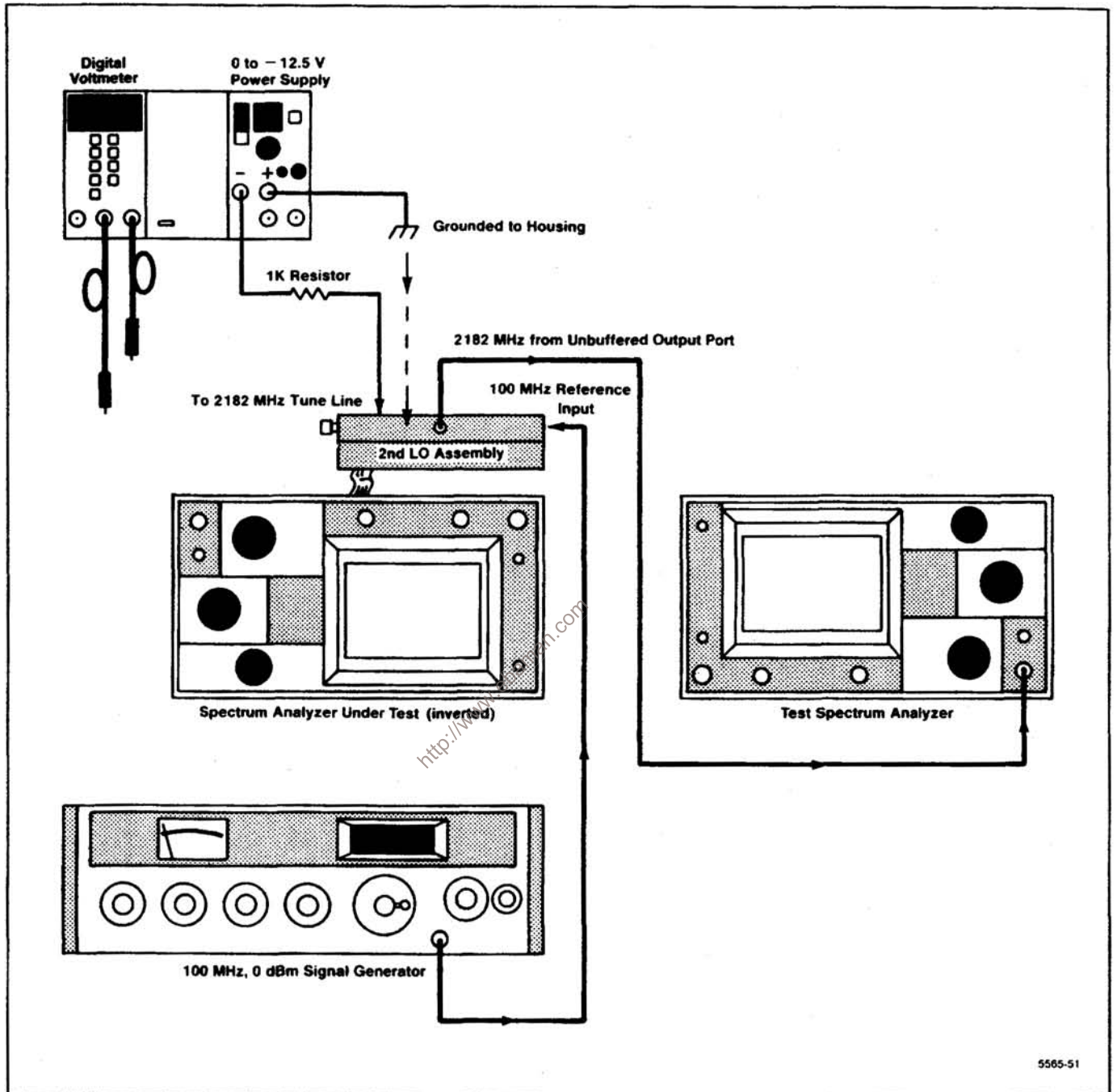
Figure 6-19. 2182 MHz Phase Locked 2nd LO adjustment setup.
