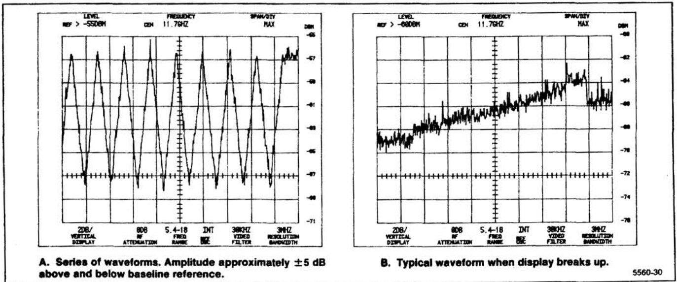
Figure 6-31. Typical baseline compensation adjustment displays.
