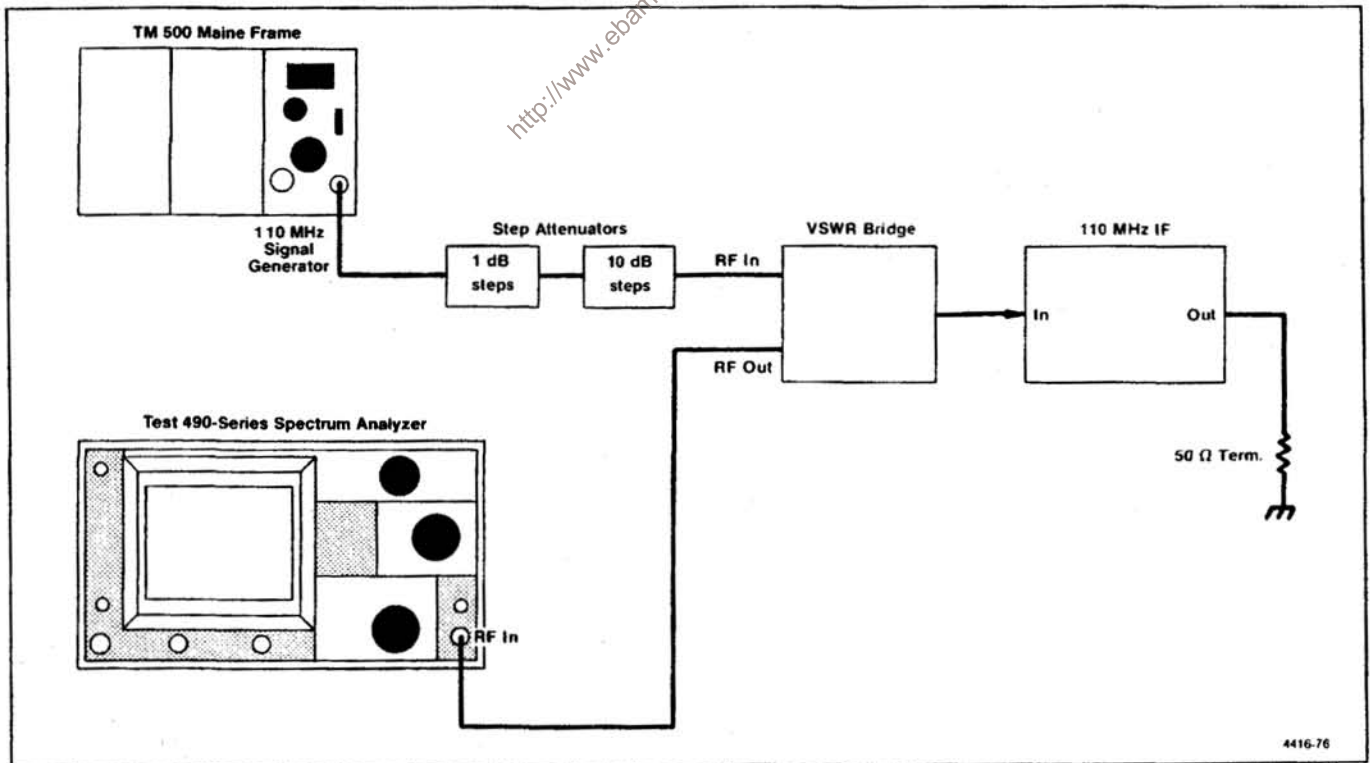
Figure 6-9. 110 MHz IF return loss adjustment setup.
