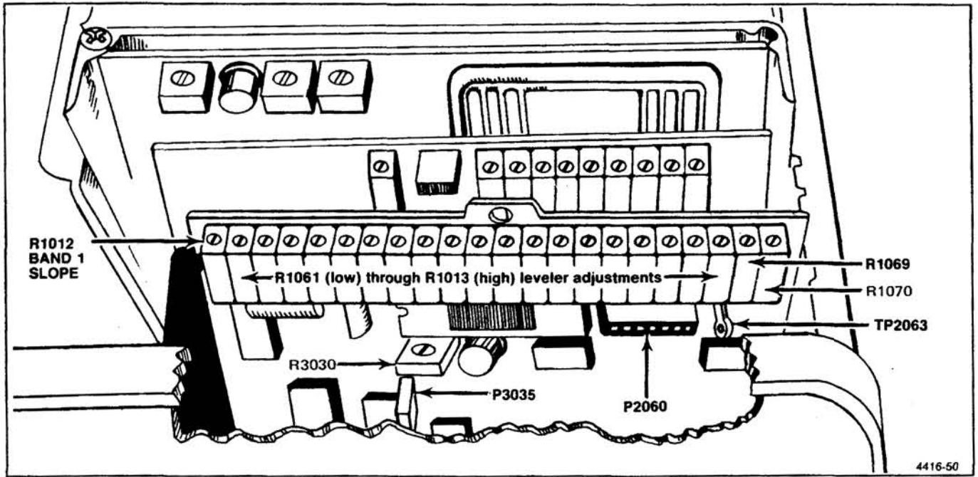
Figure 6-30. Baseline leveling adjustment and test point locations.
