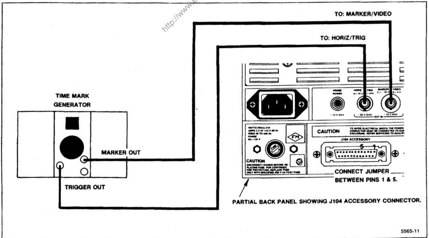
Figure 5-8. Test equipment setup for adjusting sweep timing.
