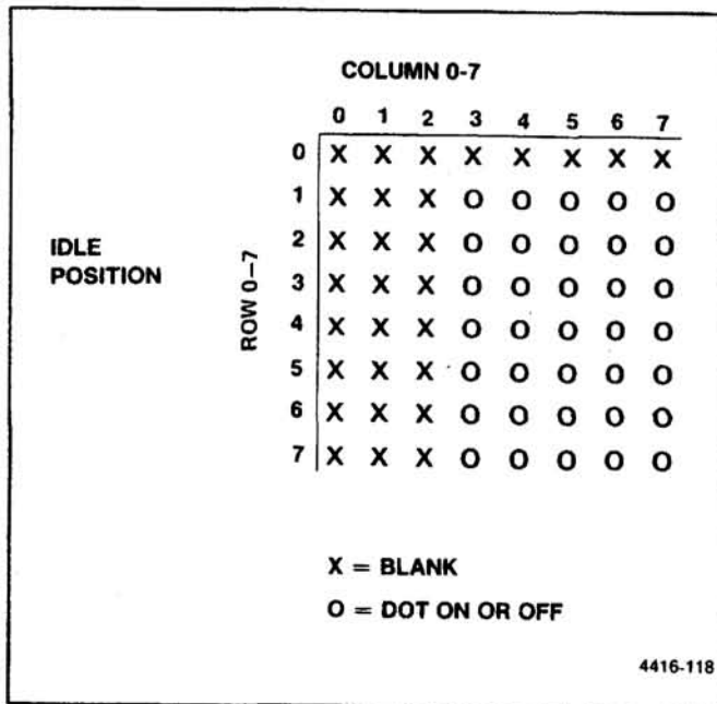
Figure 7-19. Character scan.
