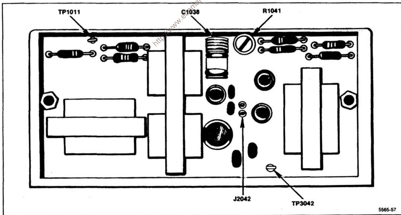
Figure 6-25. 3rd Converter test points and adjustments.
