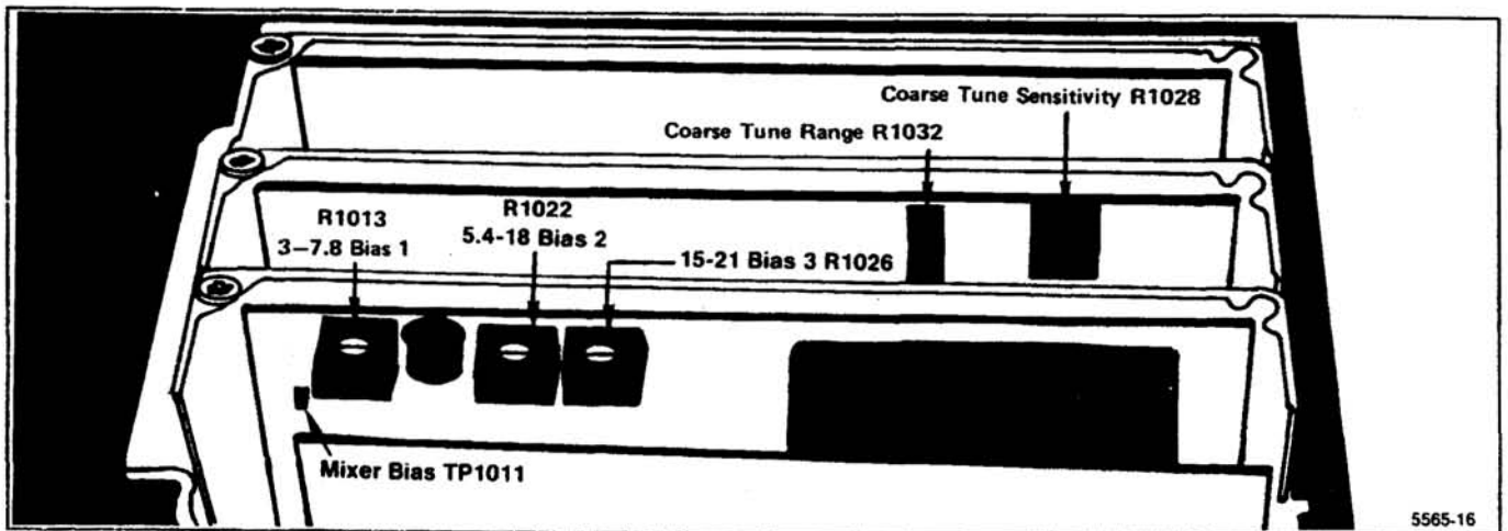
Figure 6-27. 1st LO Driver board adjustment and test point locations.
