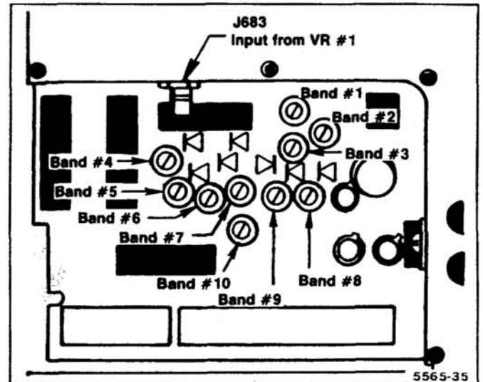
Figure 5-24. Band leveling adjustment and gain diode locations.
