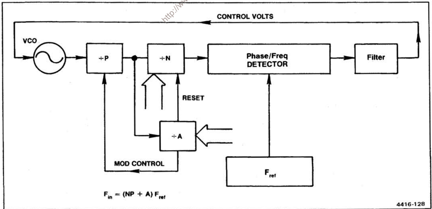
Figure 7-29. Basic block diagram of a +N synthesizer with a variable modulus prescaler.
