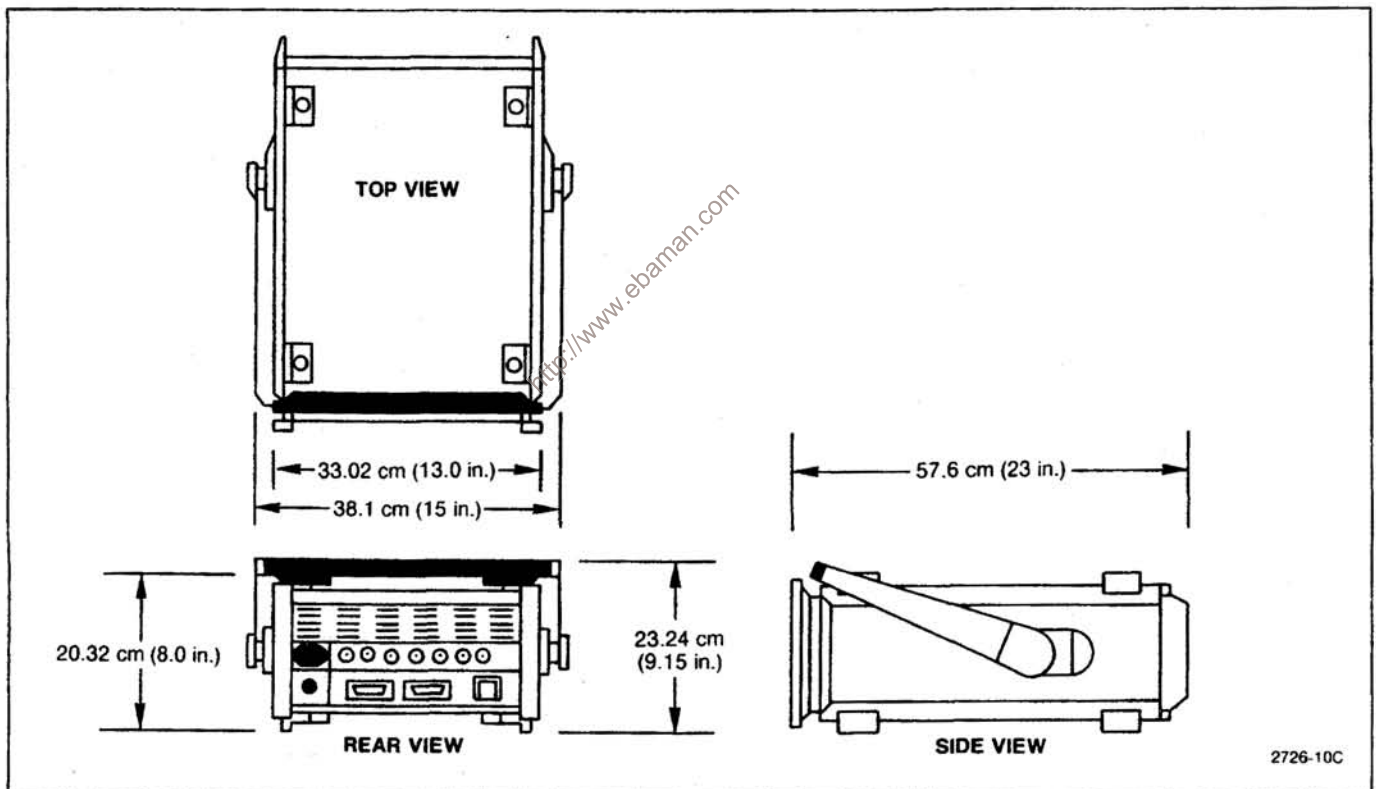
Figure 2-1. Dimensions.
