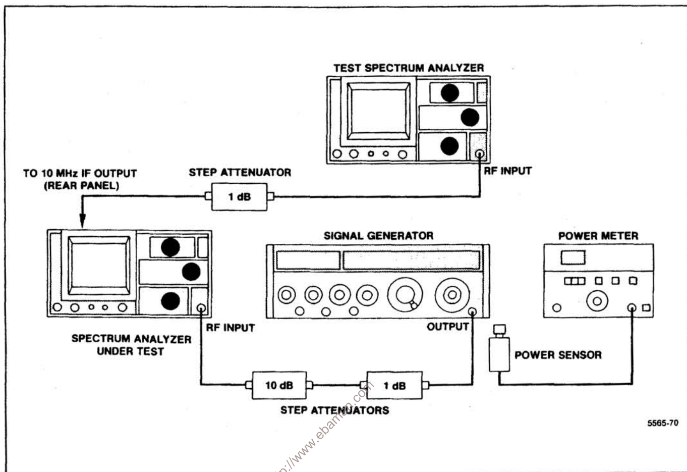
Figure 4-19. Test equipment setup for checking 1 dB input compression point.
