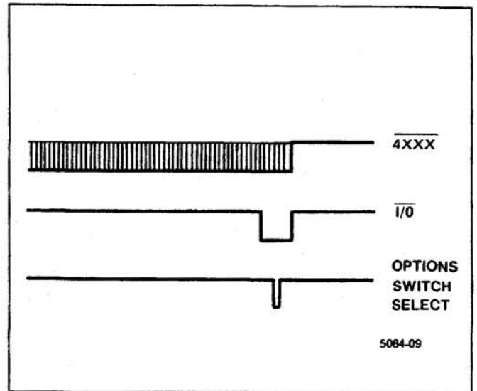
Figure 6-36. \overline{T/O} and S1050 select lines in relation to 0XXX.
