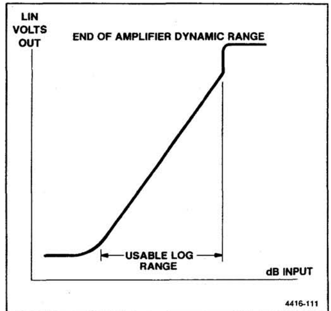
Figure 7-10. Curve showing end-of-range for a log amplifier.
