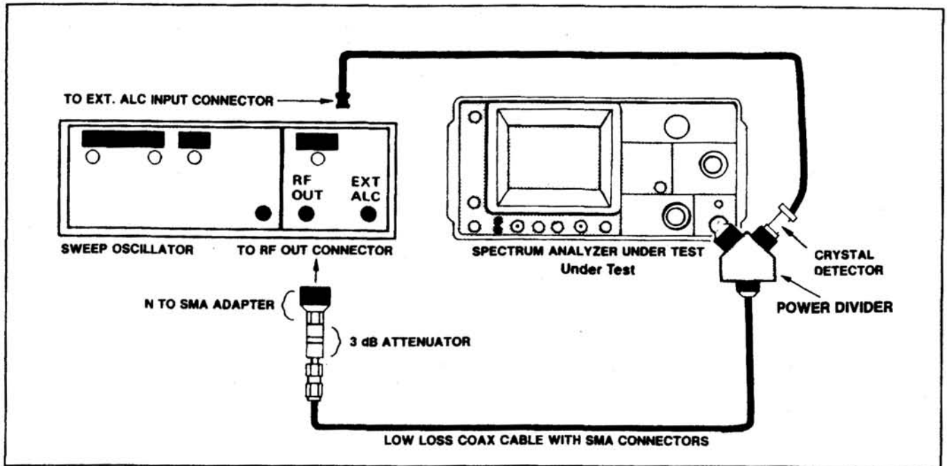
Figure 6-28. Baseline leveling test setup.
