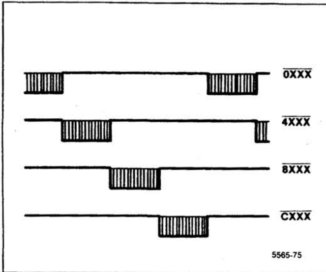
Figure 6-33. Four main block select outputs of address decoder U2045.
