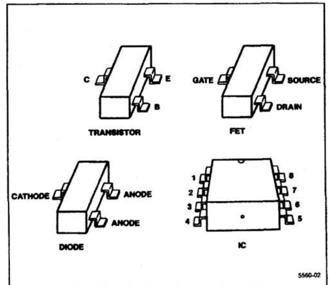
Figure 6-1. Surface-mounted components lead configuration.
