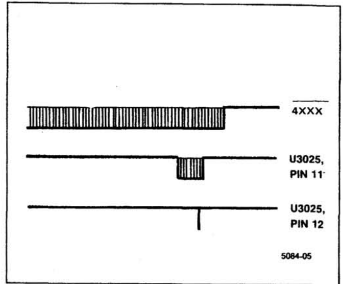
Figure 6-35. RAM select output in relation to 4XXX.
