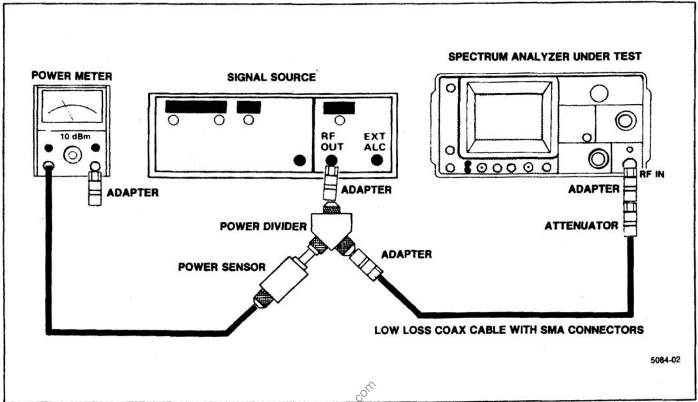
Figure 4-14. RF attenuator test equipment setup.
