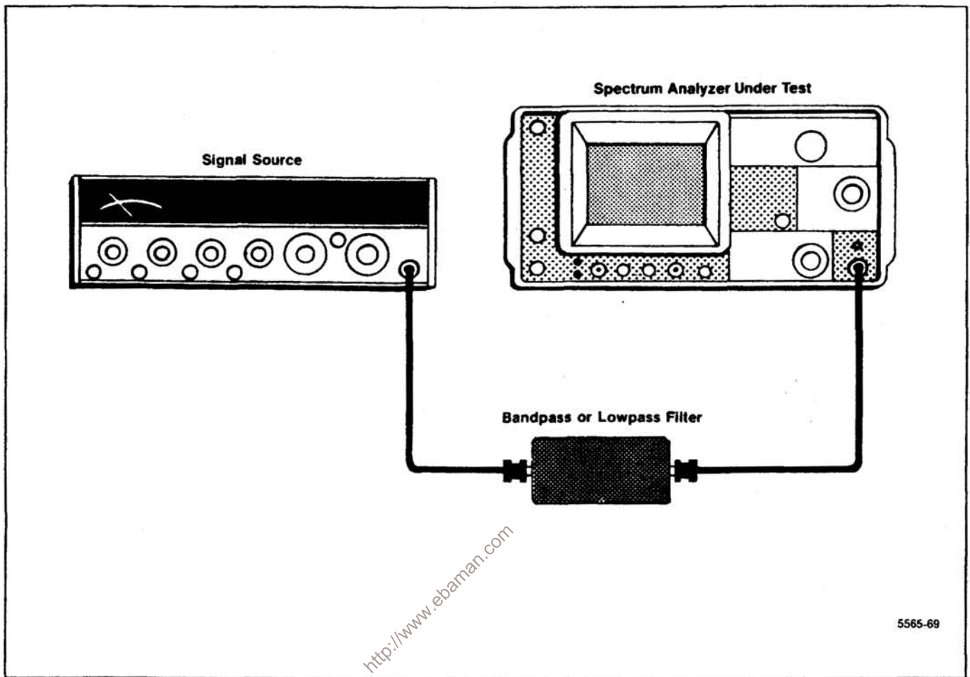
Figure 4-18. Test equipment setup for checking harmonic distortion.
