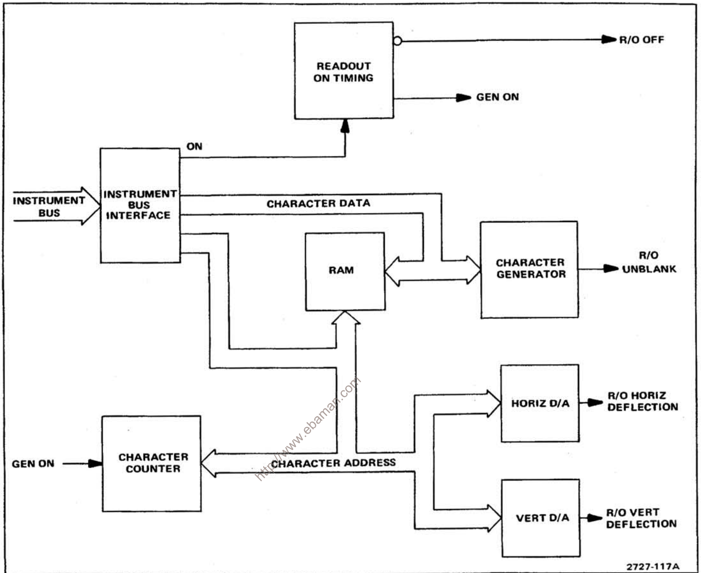
Figure 7-17. Block diagram of crt readout.
