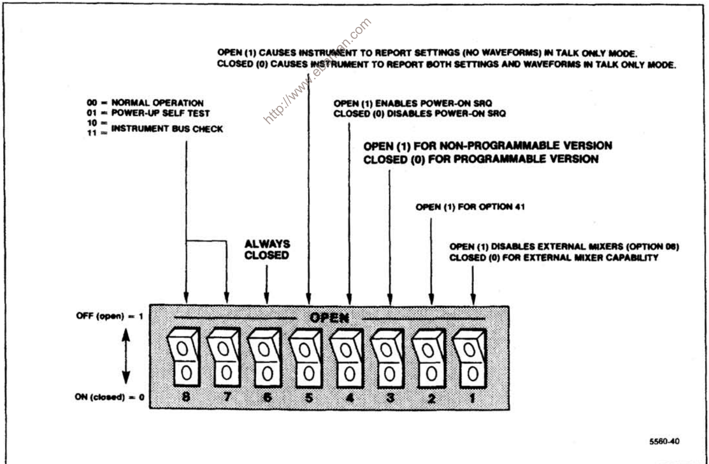
Figure 7-33. Options switch bank on the Memory board.
