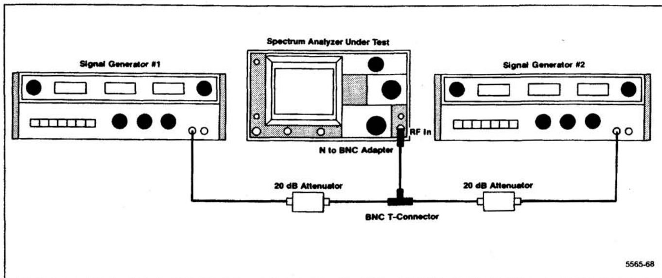
Figure 4-16. Test equipment setup for checking intermodulation distortion.
