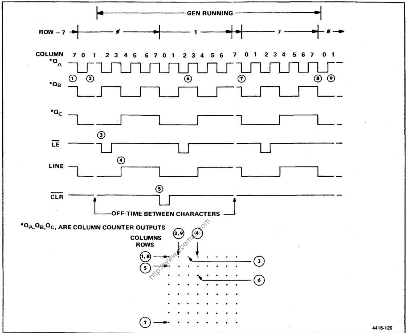
Figure 7-21. Character timing diagram.
