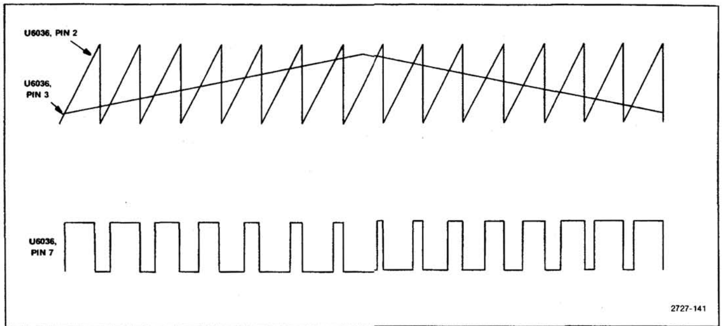
Figure 7-34. Primary regulator input and output waveforms.
