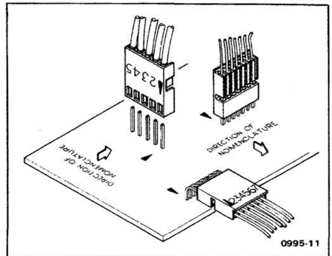
Figure 6-3. Multipin (harmonica) connectors.
