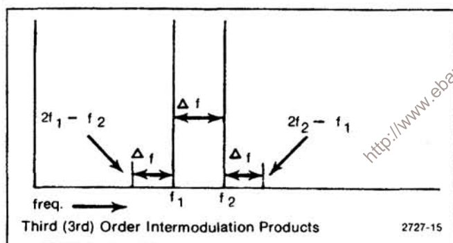
Figure 4-17. Intermodulation products.
