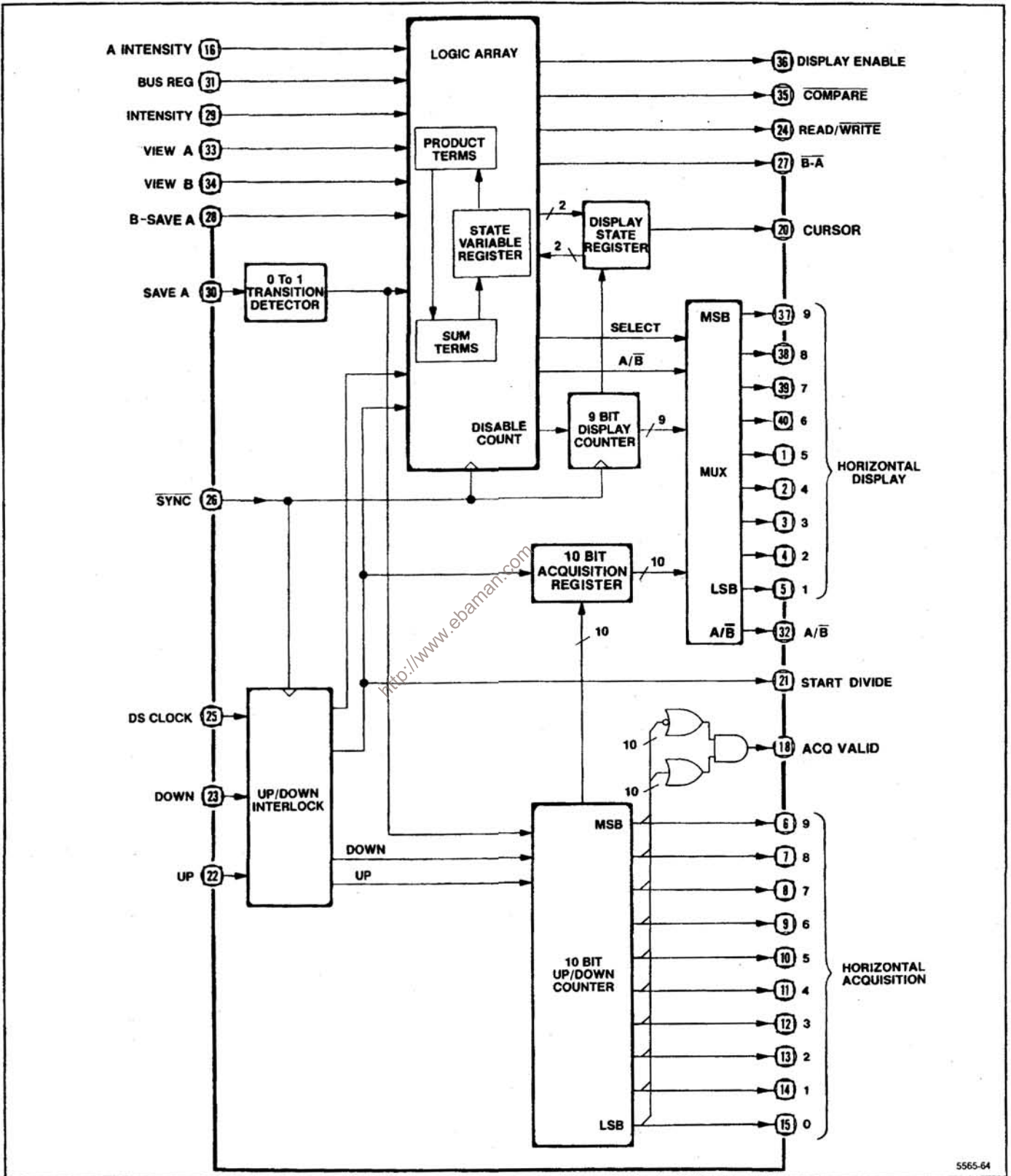
Figure 7-16. Horizontal control IC block diagram.
