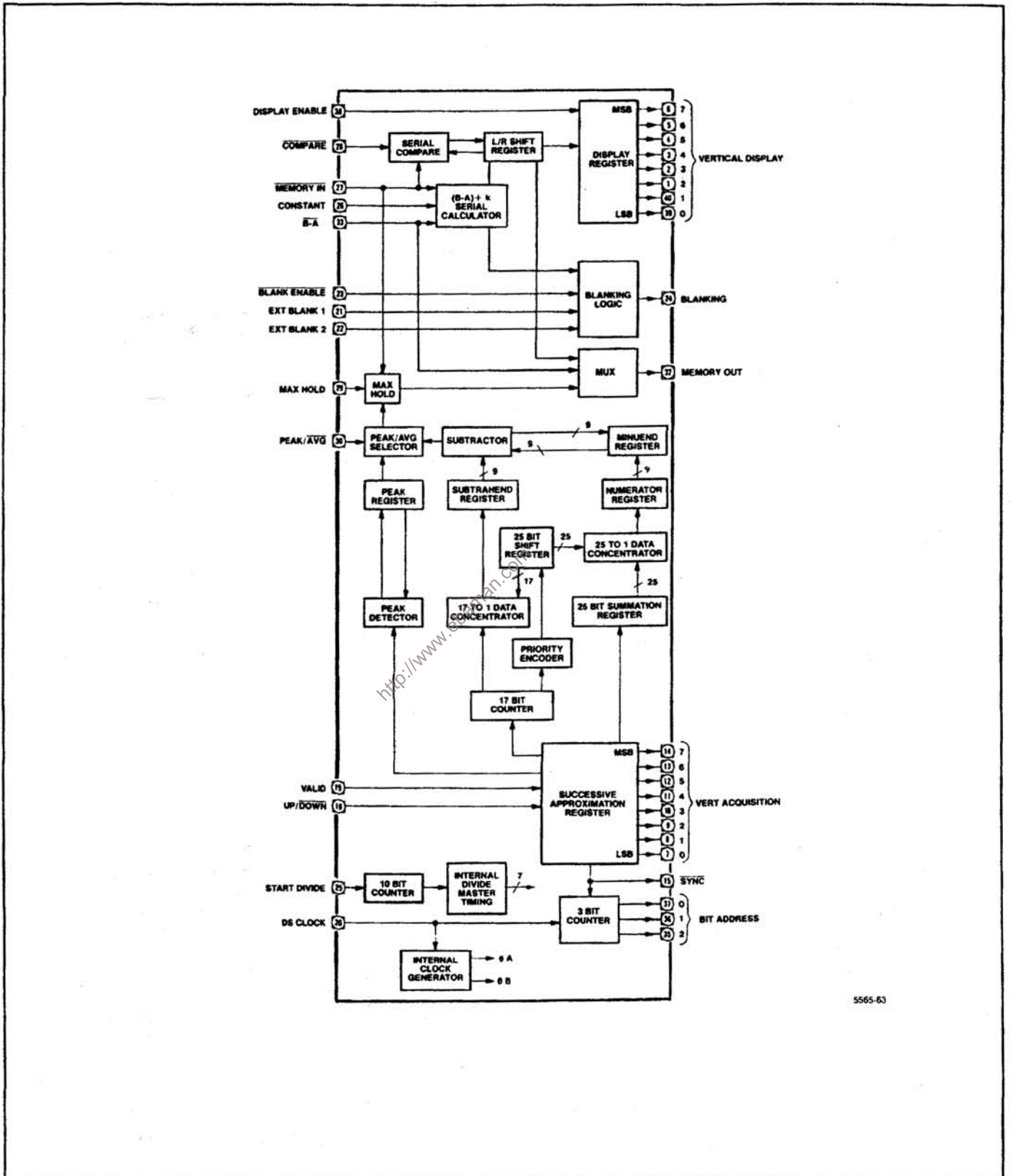
Figure 7-15. Vertical control IC block diagram.
