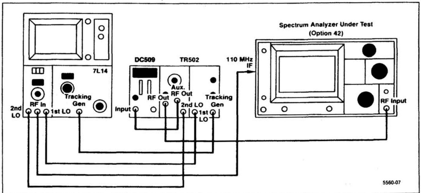
Figure 4-27. Test equipment setup for checking Option 42 frequency characteristics.
