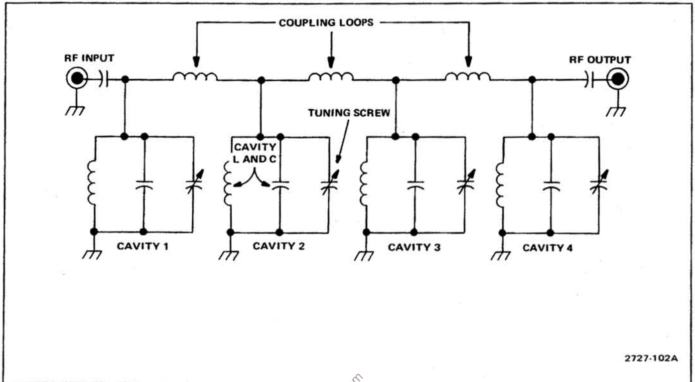
Figure 7-2. Equivalent circuit of the four-cavity filter.
