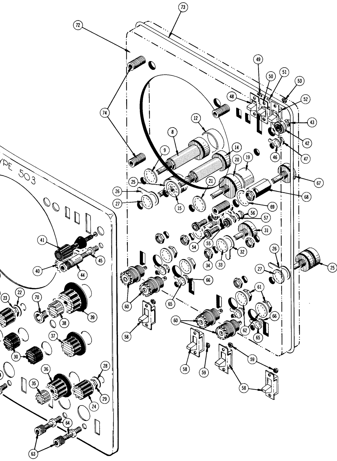
FIG. 1 FRONT
