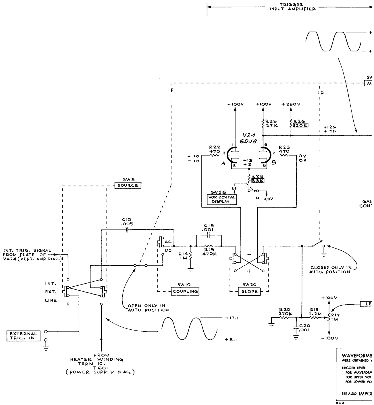
TYPE 503 OSCILLOSCOPE
