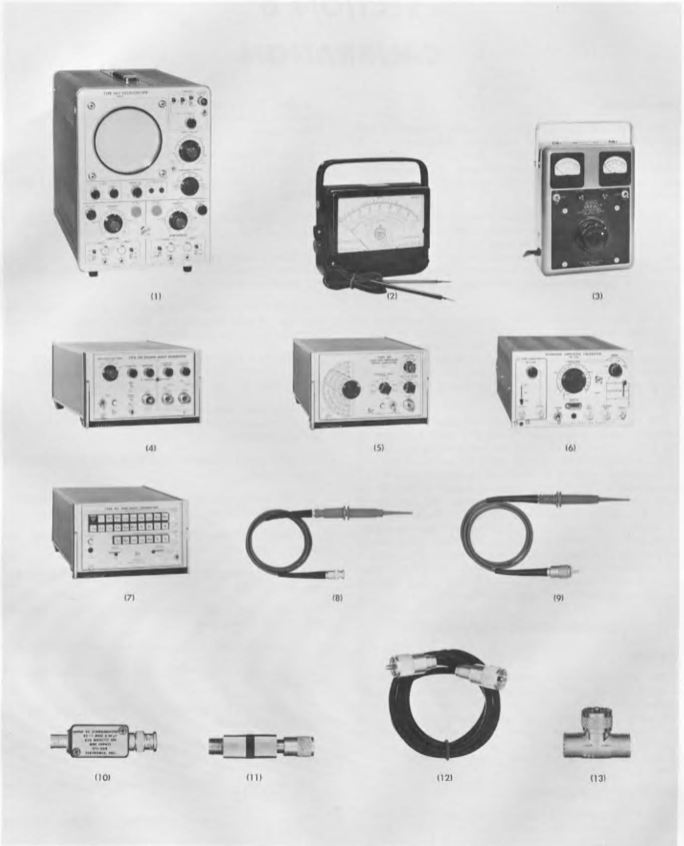
Fig. 6-1. Recommended equipment for calibration of the Type 503 Oscilloscope.
