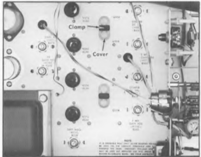
Fig. 4-3. Transistor heat-stabilizing covers used in instruments serial numbered 6997 and later.
