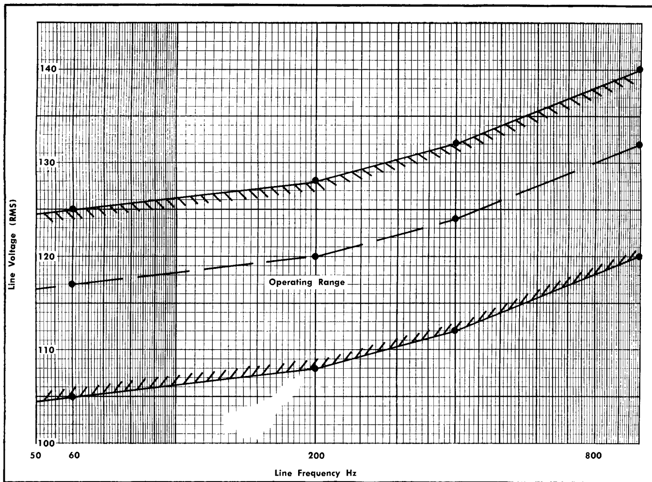
Fig. 2-1. Line voltage requirements at various line frequencies.
