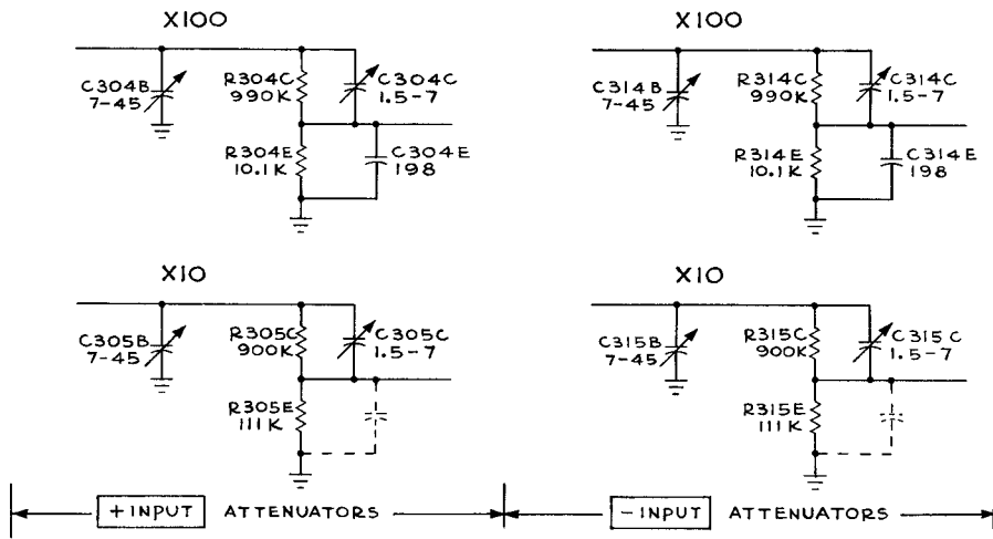
TYPE 503 OSCILLOSCOPE
