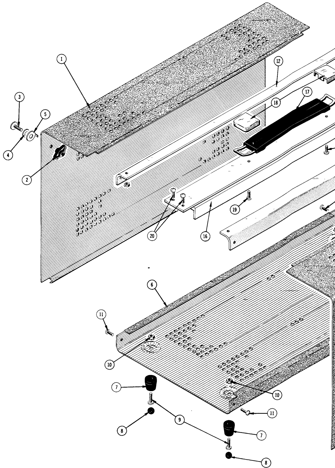
FIG. 5 CABINET
