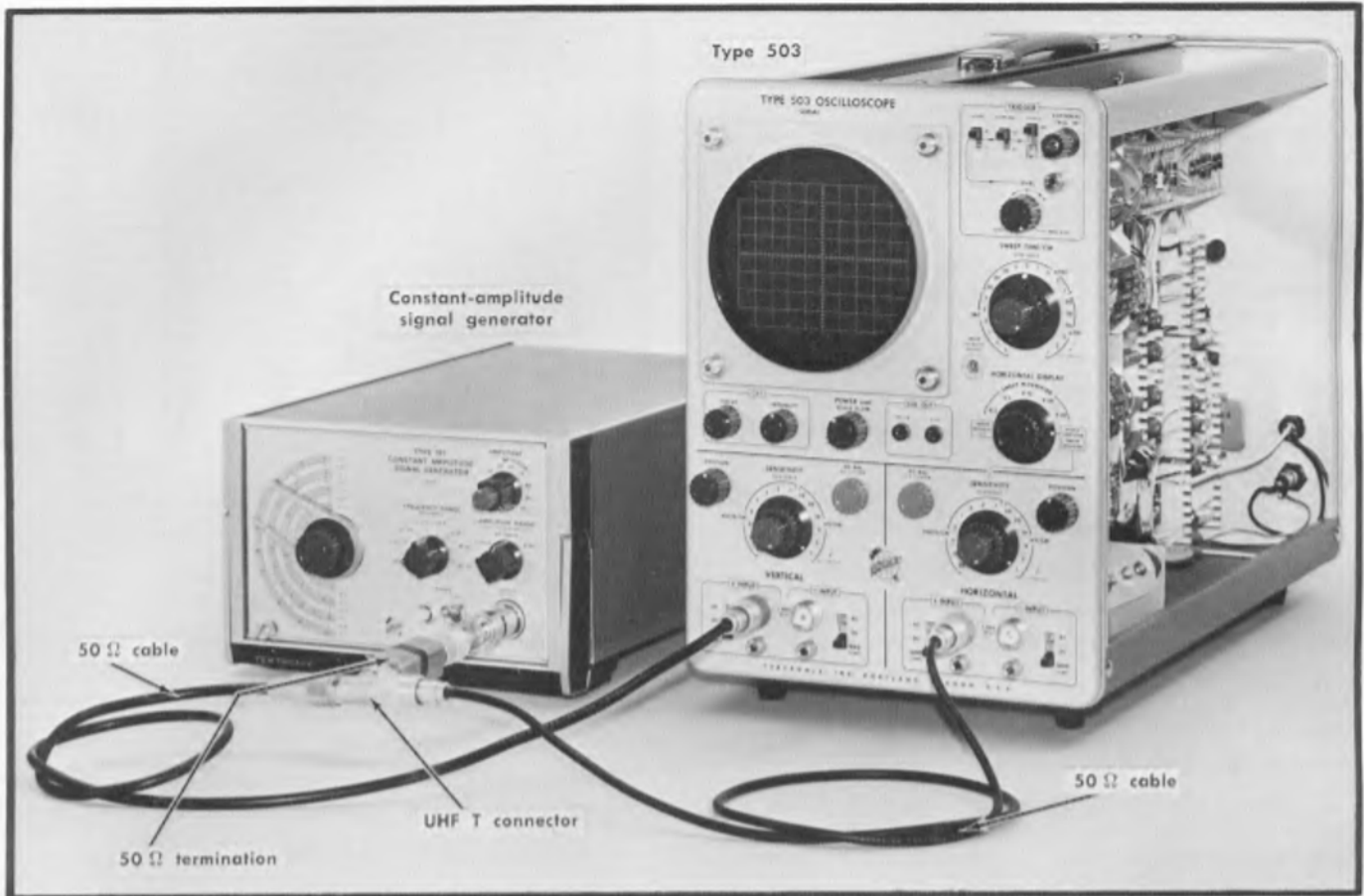
Fig. 6-24. Test setup for adjusting amplifier phasing.
