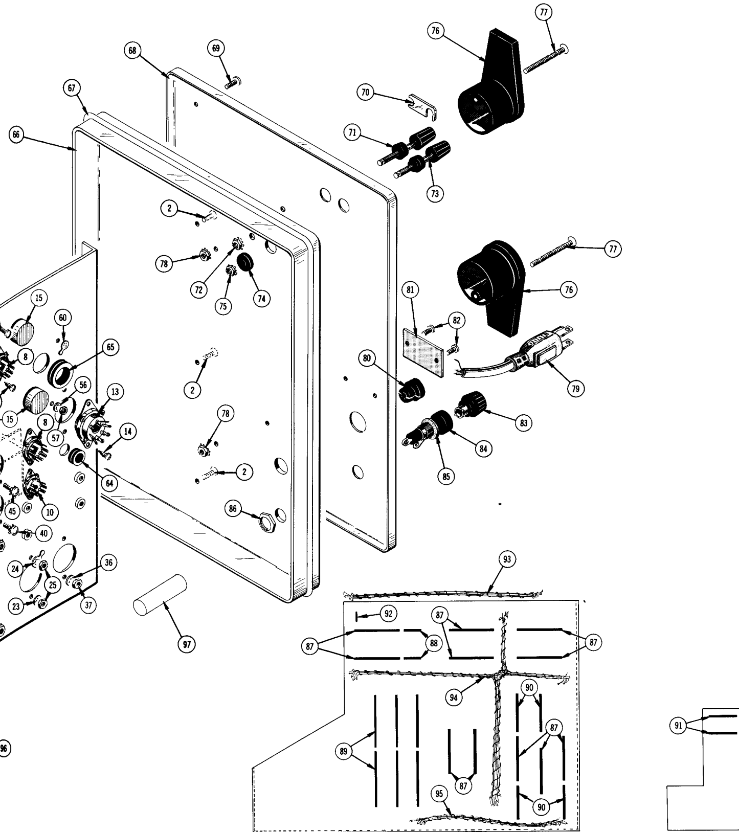
FIG. 4 CHASSIS & REAR
