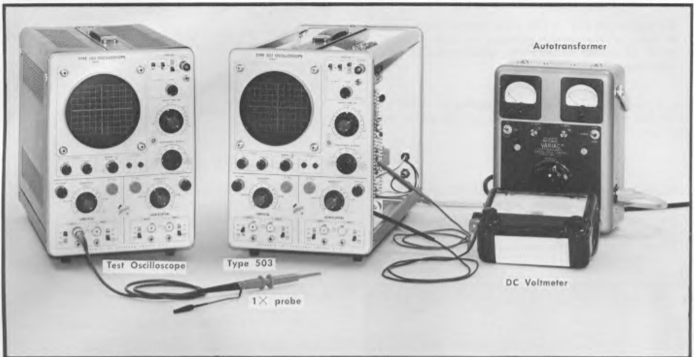
Fig. 6-6. Test equipment setup for power supply ripple and regulation check.
