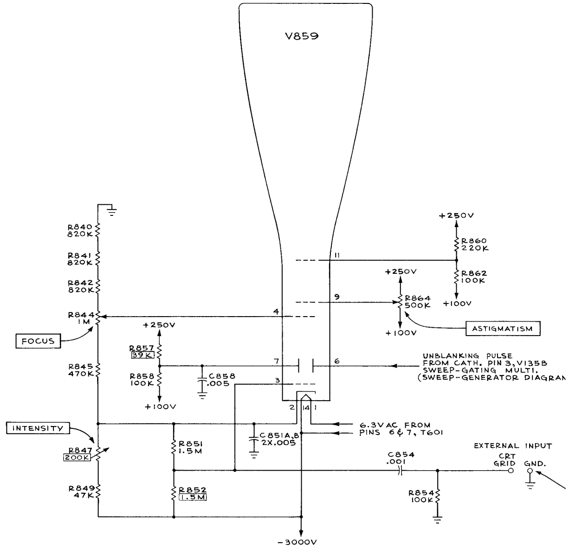
TYPE 503 OSCILLOSCOPE
