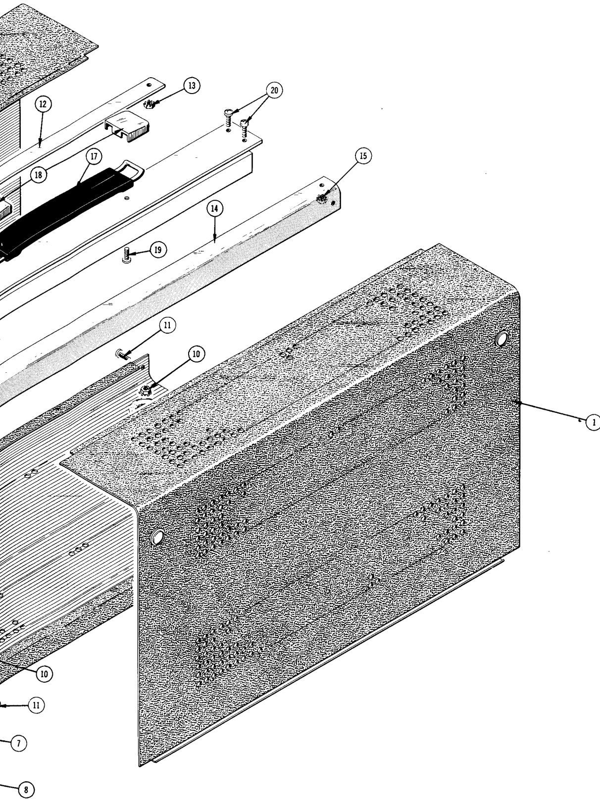
FIG. 5 CABINET
