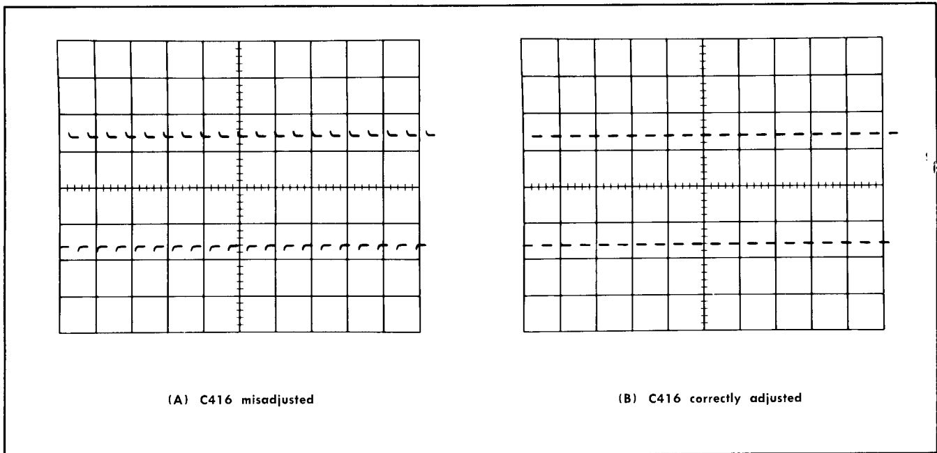
Fig. 5-2. Typical displays, Vertical Amplifier attenuator compensation check; 1 kHz square-wave input; sweep speed, 2 milliseconds/cm.
