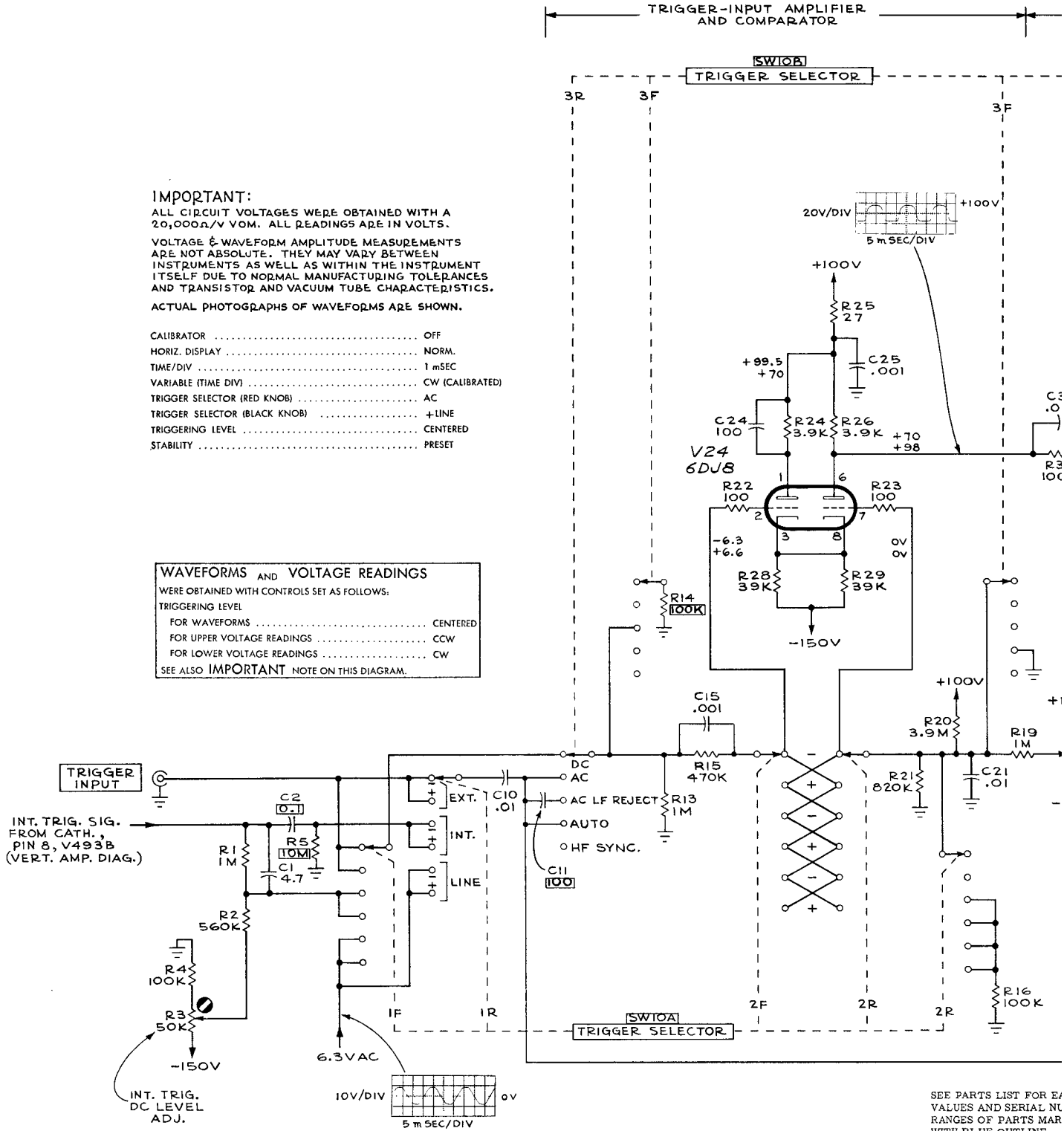
TYPE 516 OSCILLOSCOPE
