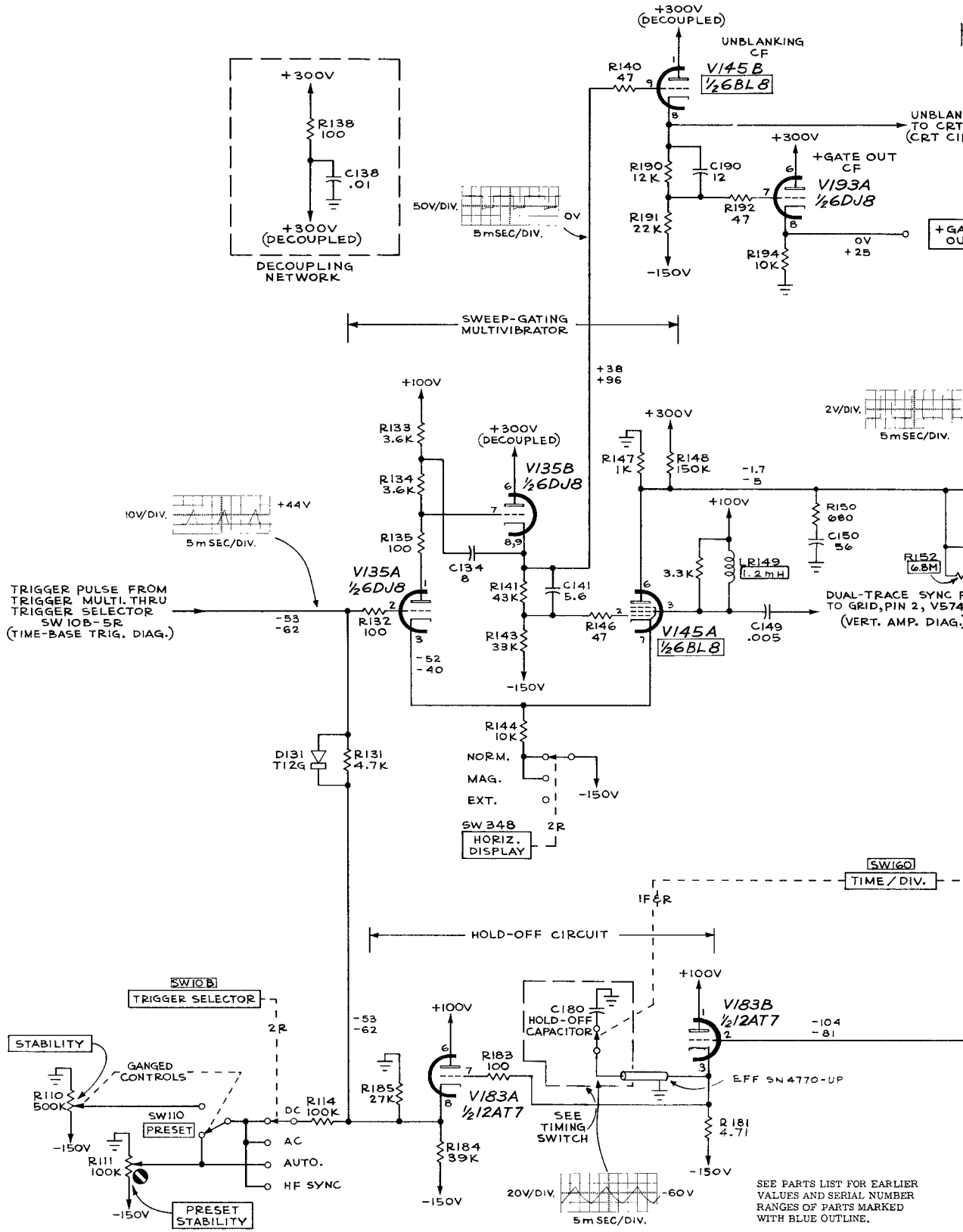
TYPE 516 OSCILLOSCOPE
