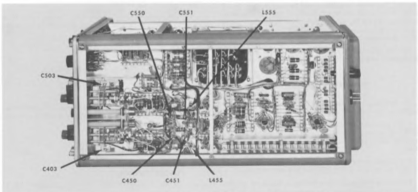
Fig. 6-2. Bottom of Type 516 Oscilloscope, showing location of internal adjustments.
