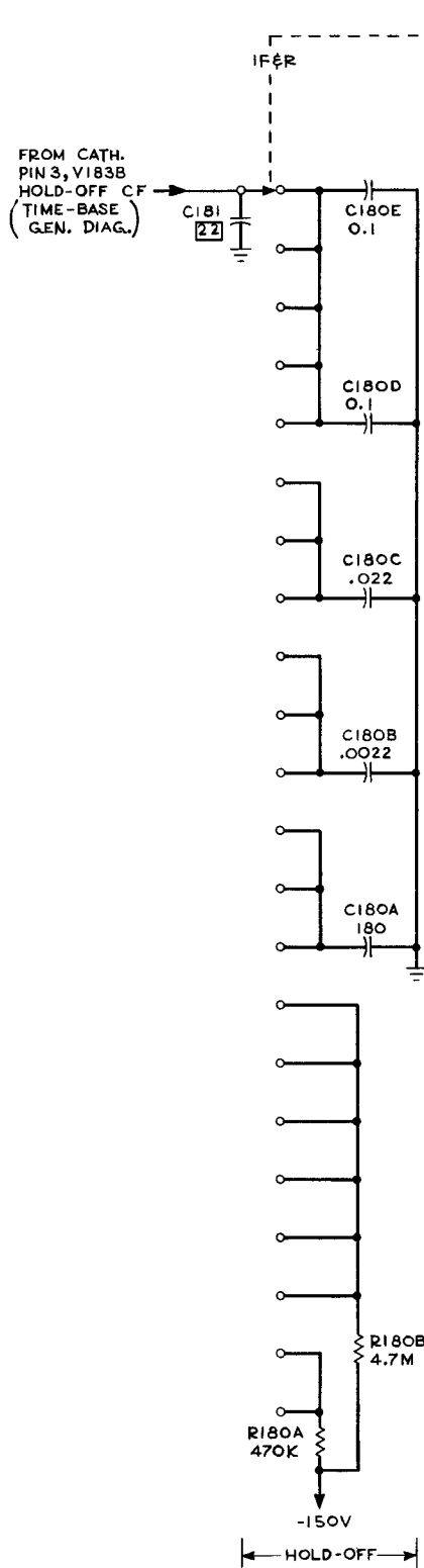
TYPE 516 OSCILLOSCOPE
