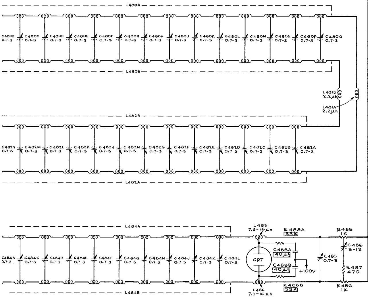
C 1 VERTICAL OUTPUT STAGE & DELAY LINE CIRCUIT NUMBERS 450 THRU 499 664 TP
