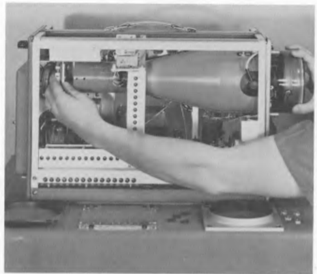
Fig. 5-2. Removing the cathode-ray tube.
