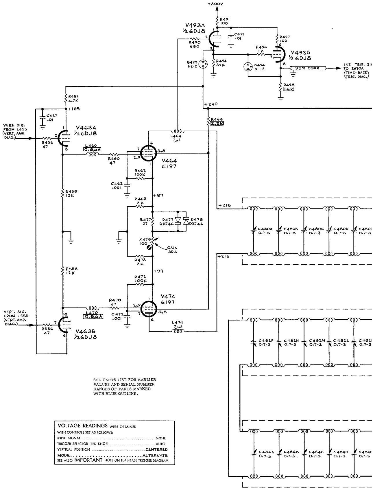
TYPE 516 OSCILLOSCOPE
