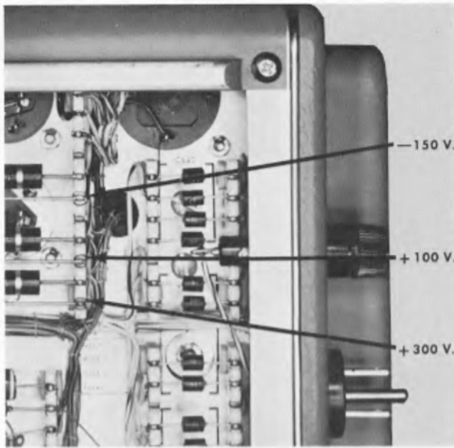
Fig. 6-4. Location of Power Supply test points.
