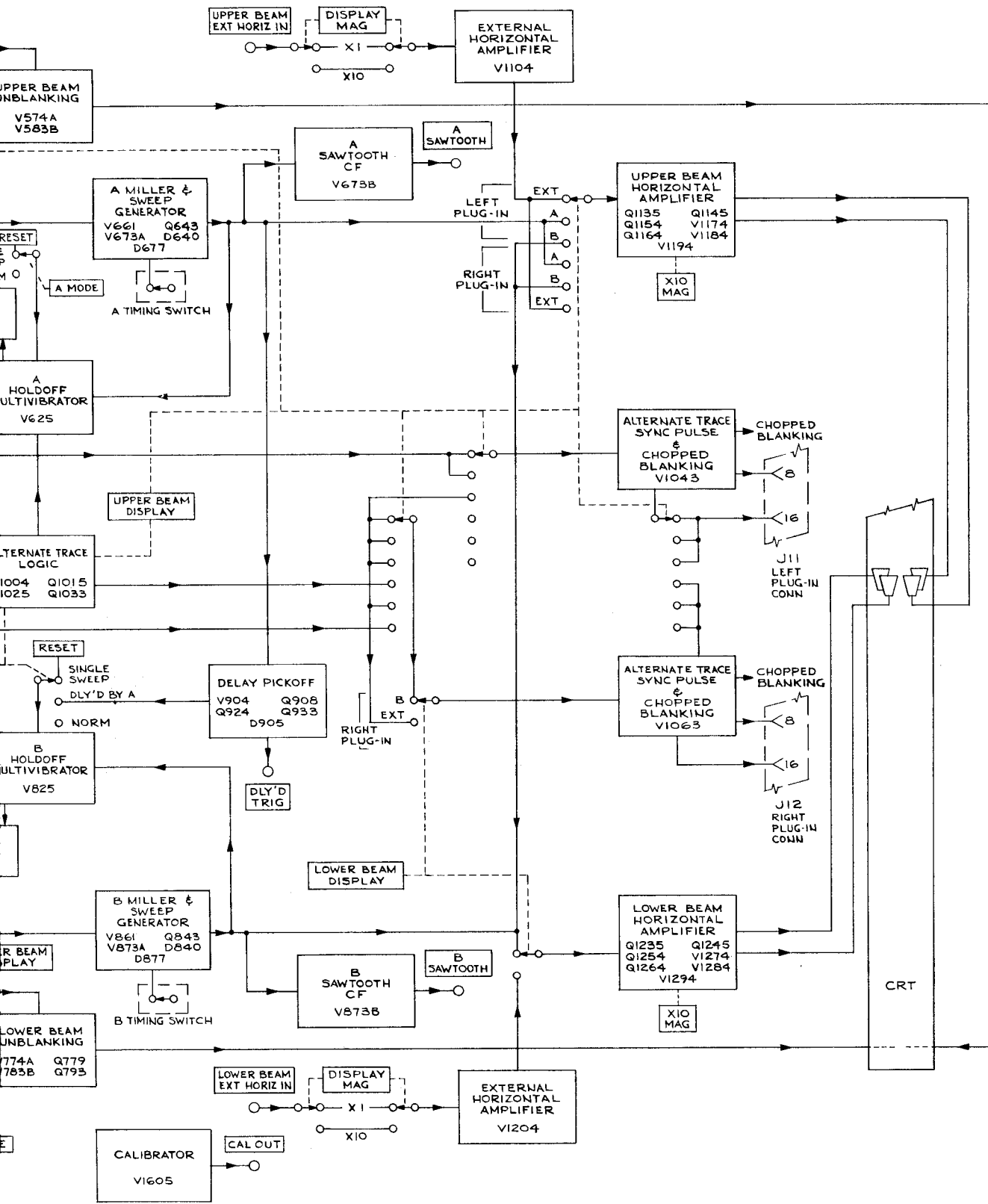
HORIZONTAL BLOCK DIAGRAM
