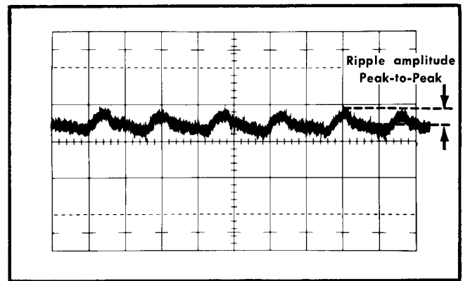
Fig. 6-9. Typical display showing ripple on +350-volt supply (60 cycle line). Vertical deflection, 0.005 volts/cm; sweep rate, 5 milliseconds/cm; high load condition.
