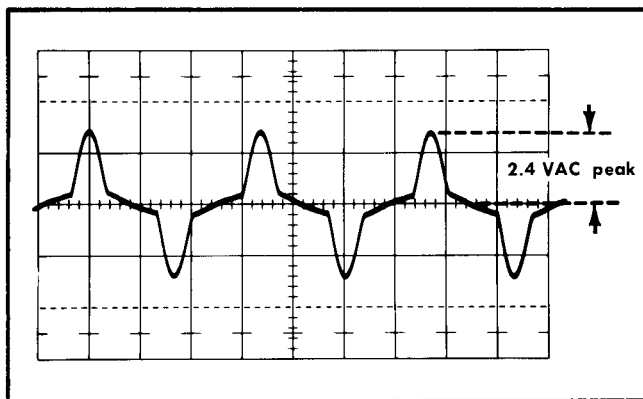
Fig. 5-4. Illustrating measurement of voltage drop in neutral wire. Probe connected between grounding pin and neutral wire; Type W Time/cm, 5 milliseconds; vertical sensitivity, 2 volts/cm.
