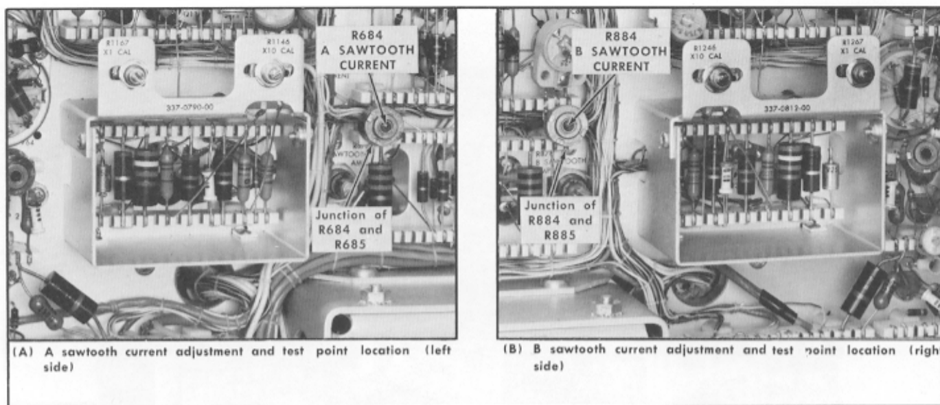
Fig. 6-39. A and B sawtooth current adjustment and test point locations.
