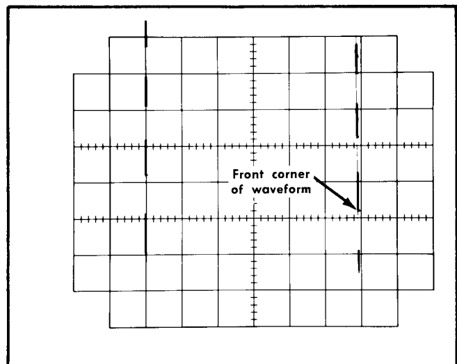
Fig. 5-10. Typical display, External Horizontal Amplifier Compensation check.
