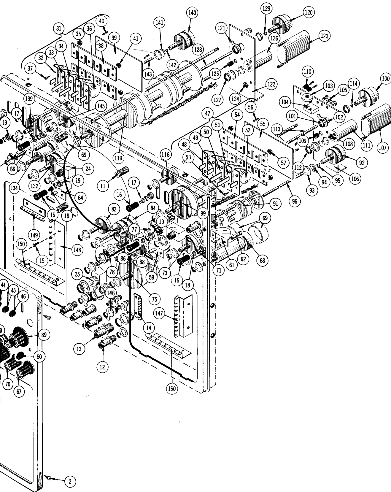
FIG. 1 FRONT & SWITCHES
