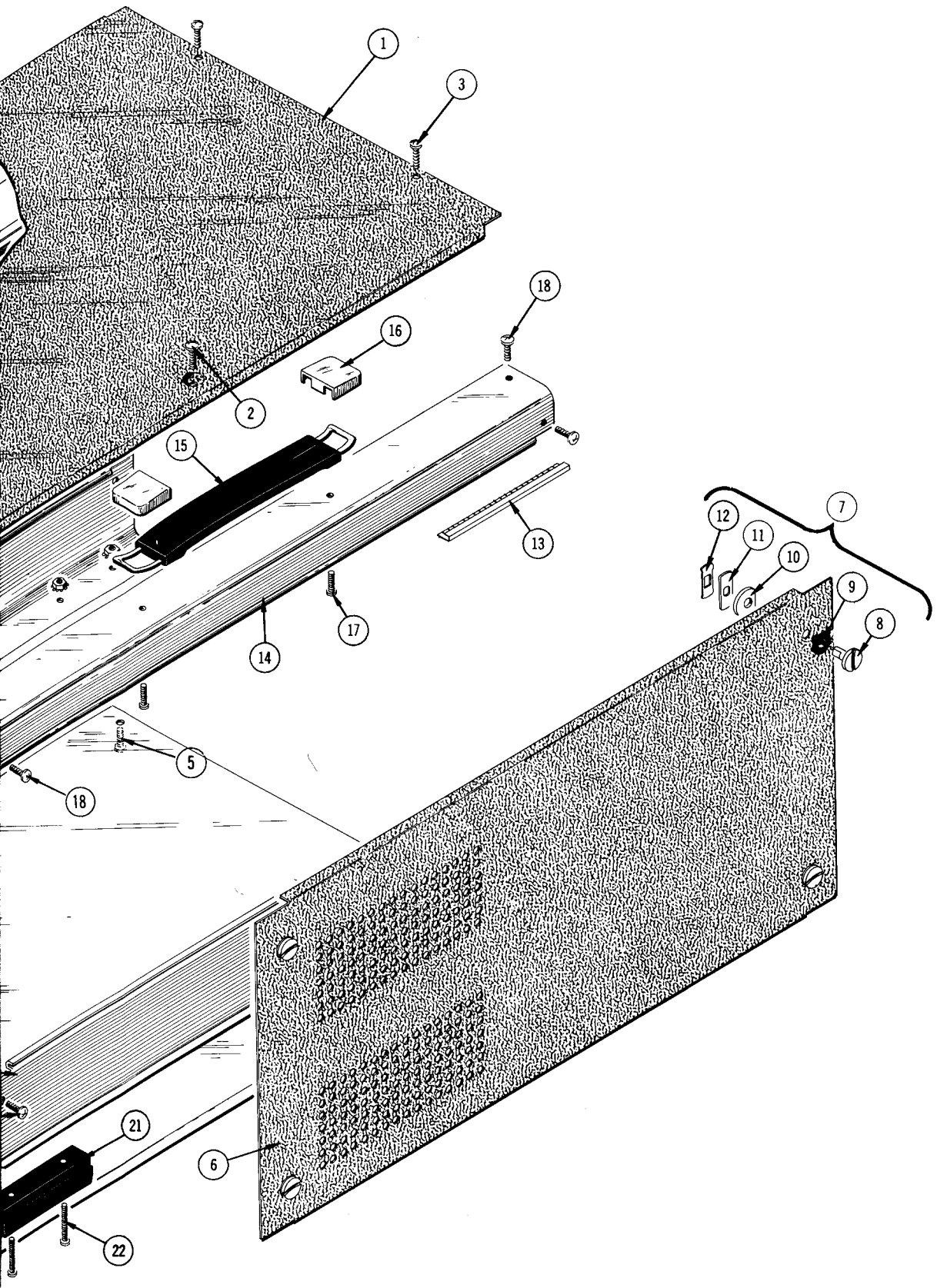
FIG. 8 CABINET & RAILS
