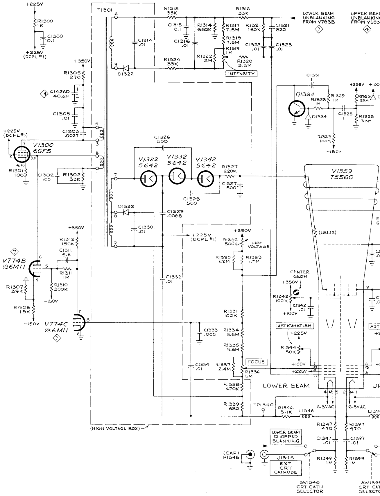
TYPE 556 OSCILLOSCOPE
