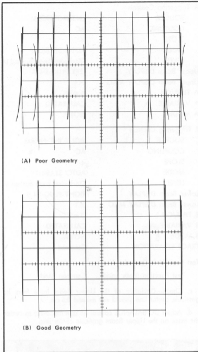
Fig. 6-18. Typical CRT displays showing (A) poor geometry adjustment; (B) good geometry adjustment.
