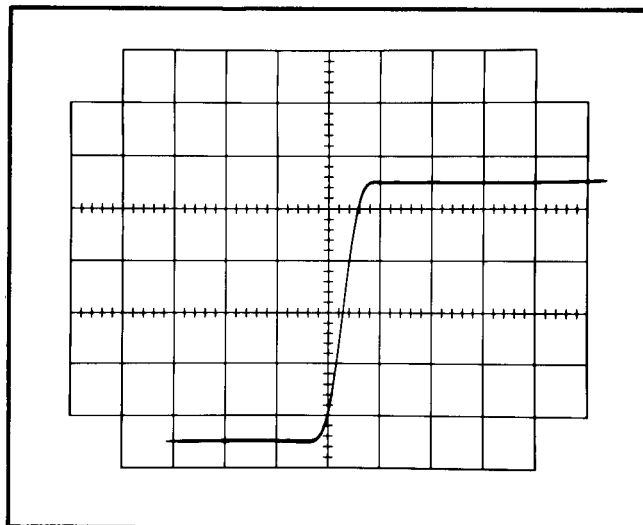
Fig. 5-14. Correct positioning of Lower Beam waveform for risetime check.
