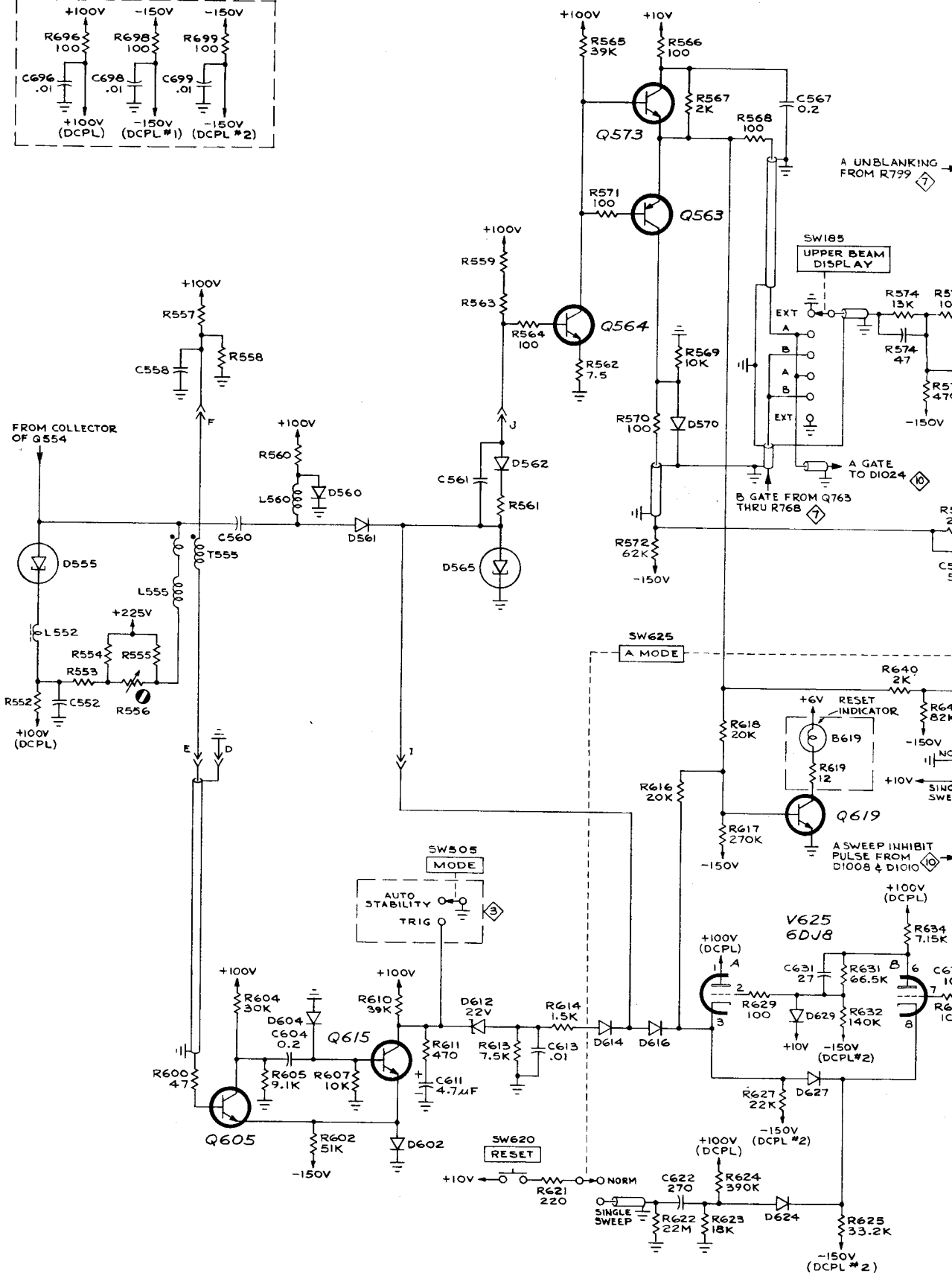
TYPE 556 OSCILLOSCOPE
