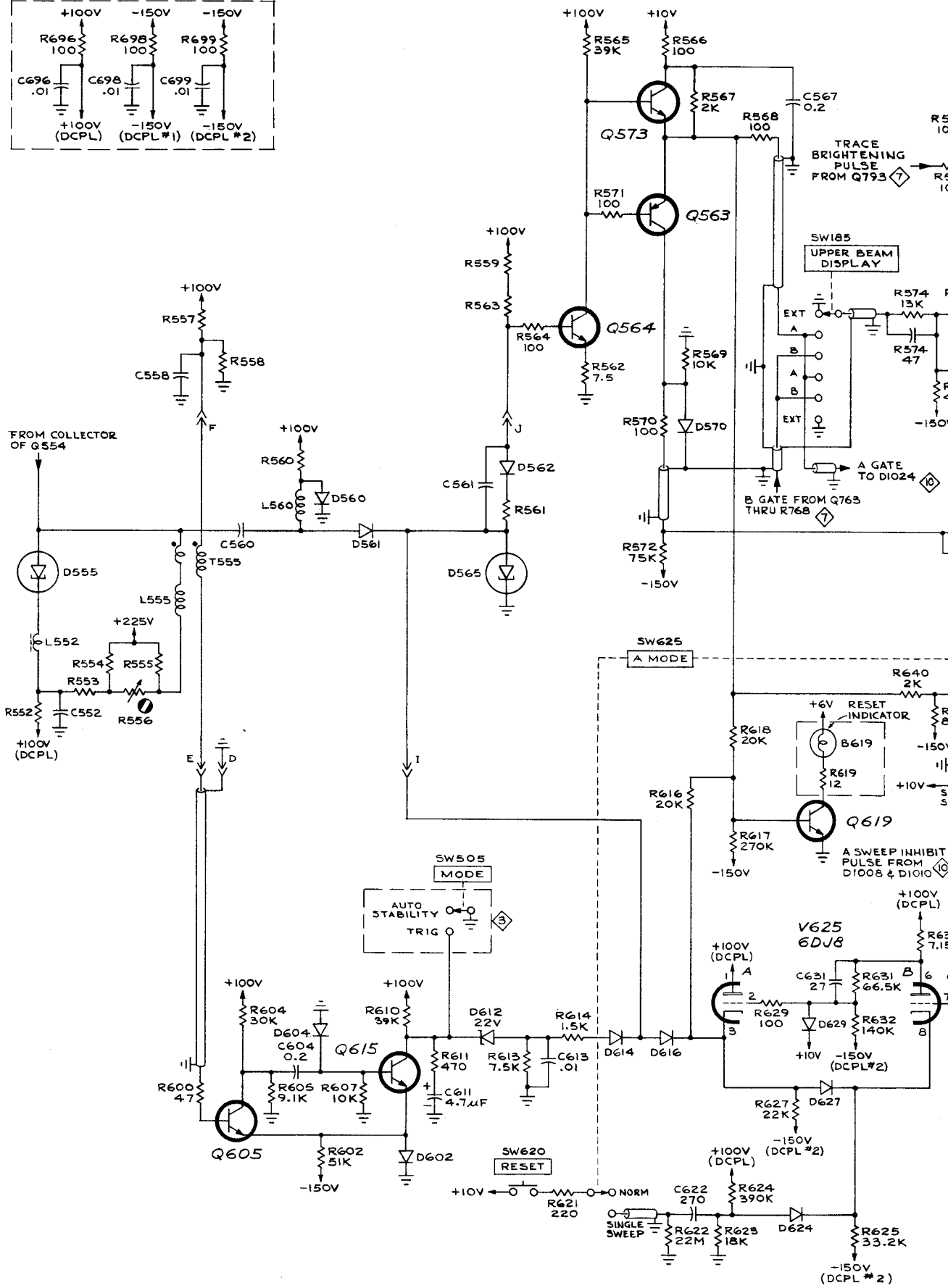
TYPE 556 OSCILLOSCOPE
