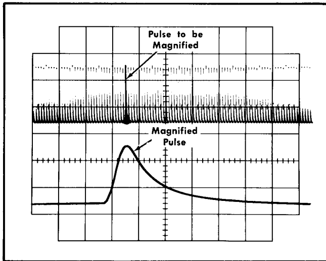
Fig. 2-20. Using delayed sweep for sweep magnification.
