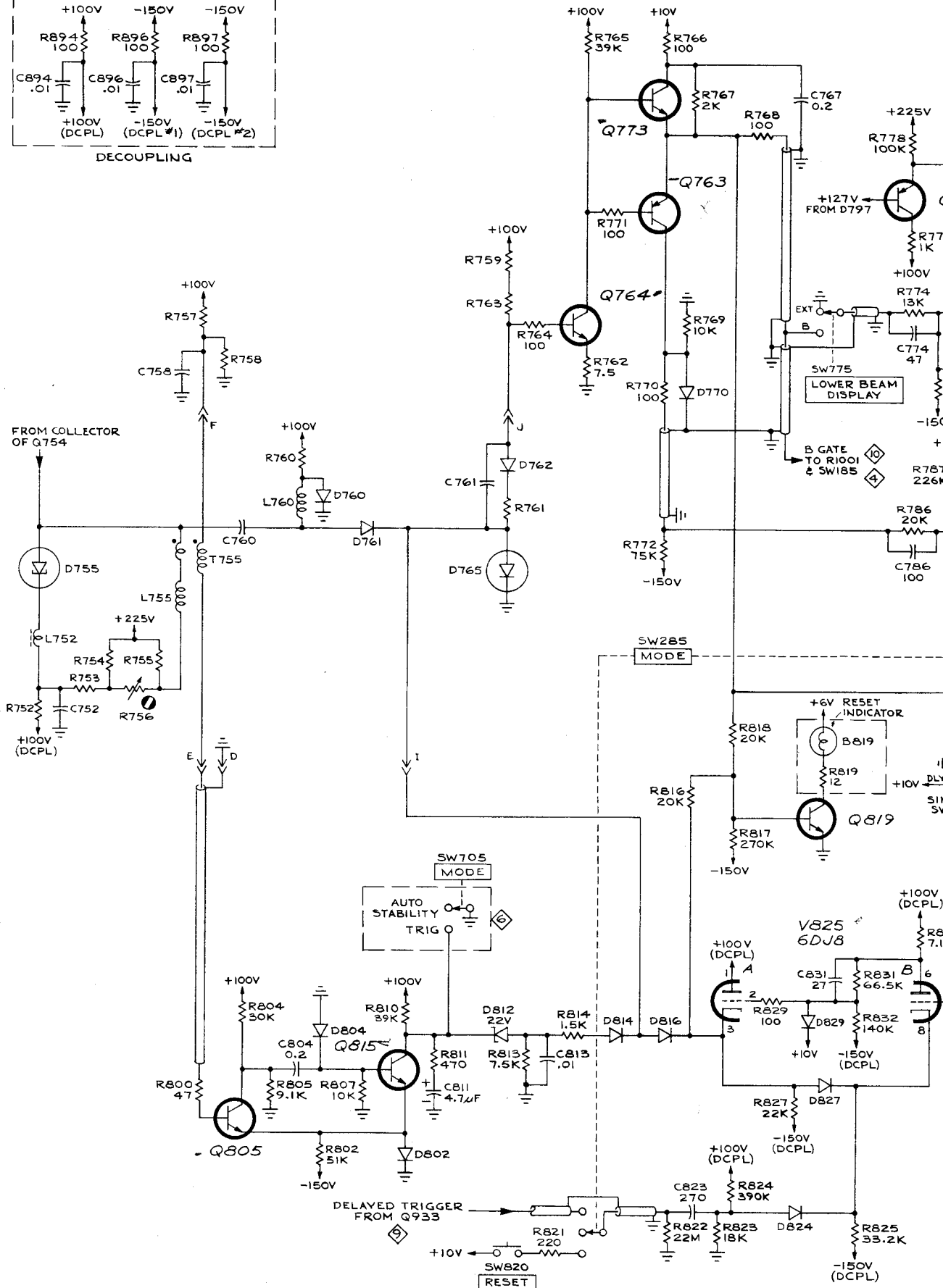
TYPE 556 OSCILLOSCOPE
