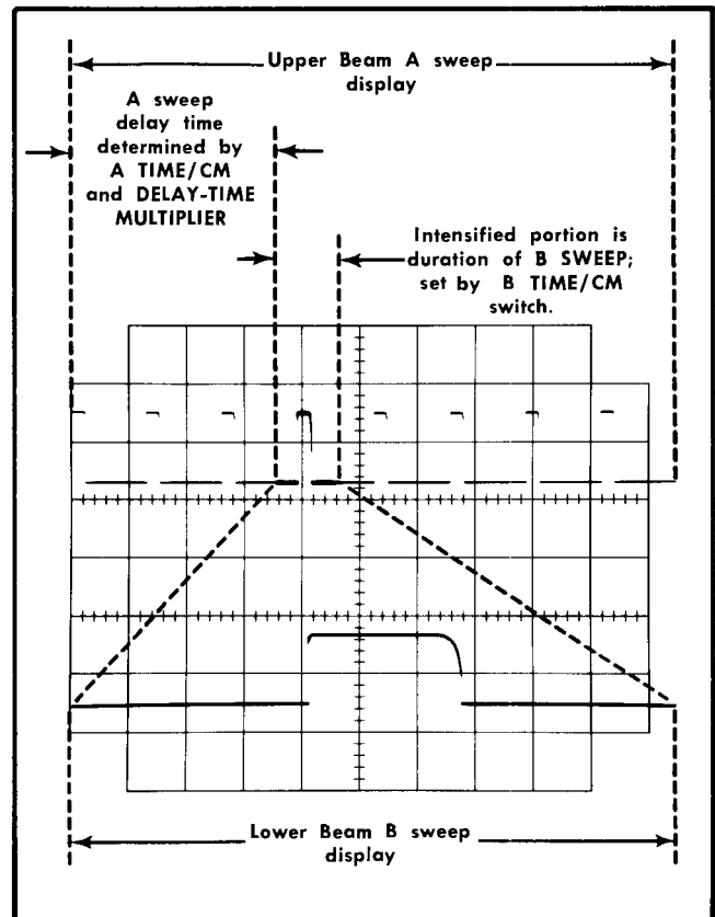
Fig. 2-11. DLY'D BY A mode of operation. The intensified portion of the Upper Beam is expanded and displayed by the Lower Beam. A TIME/CM, .5 mSEC; B TIME/CM, 50 μSEC.
