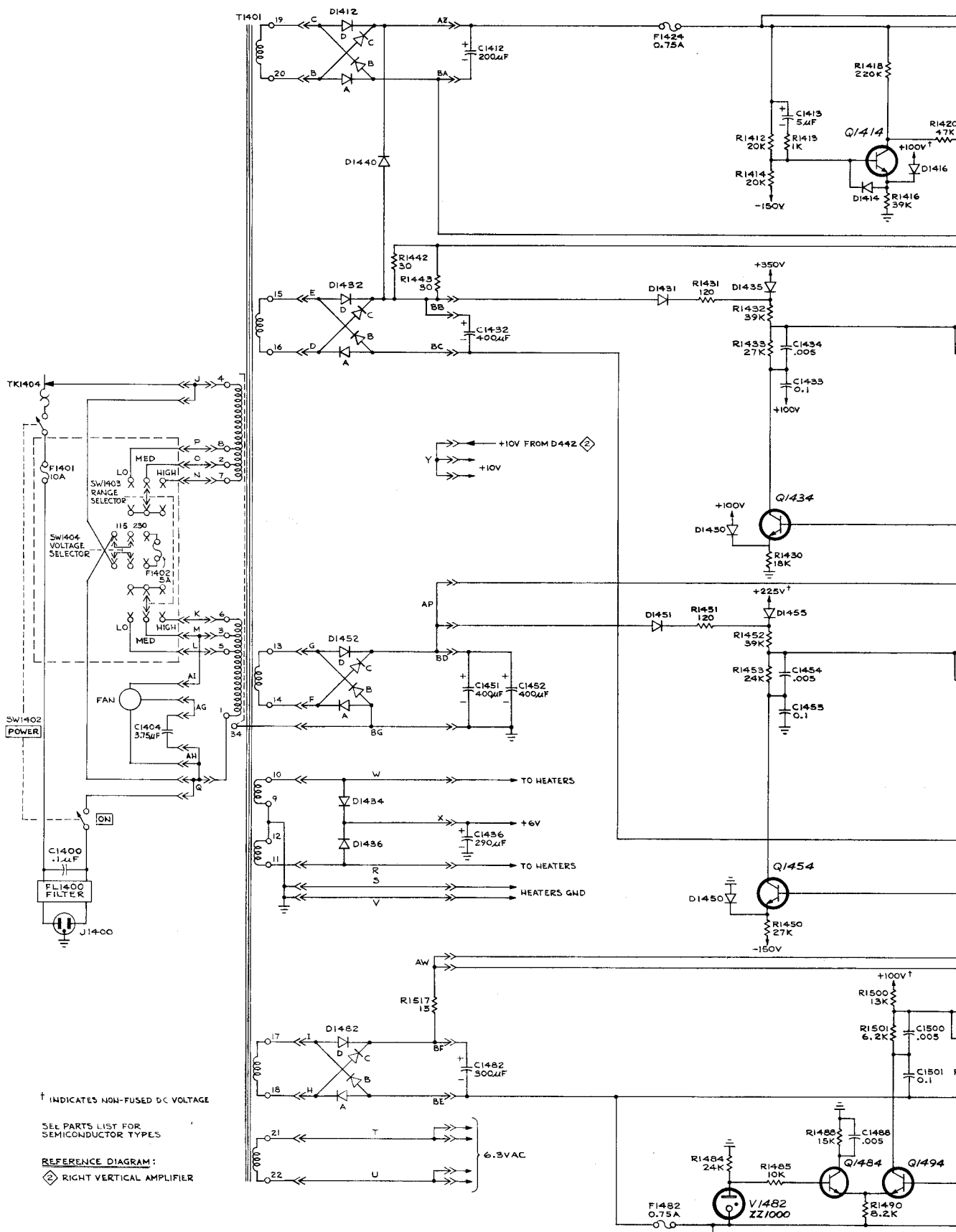
TYPE 556 OSCILLOSCOPE
