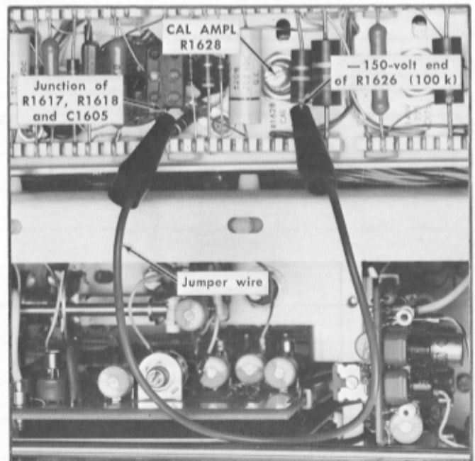
Fig. 6-12. Test setup for Amplitude Calibrator adjustment.
