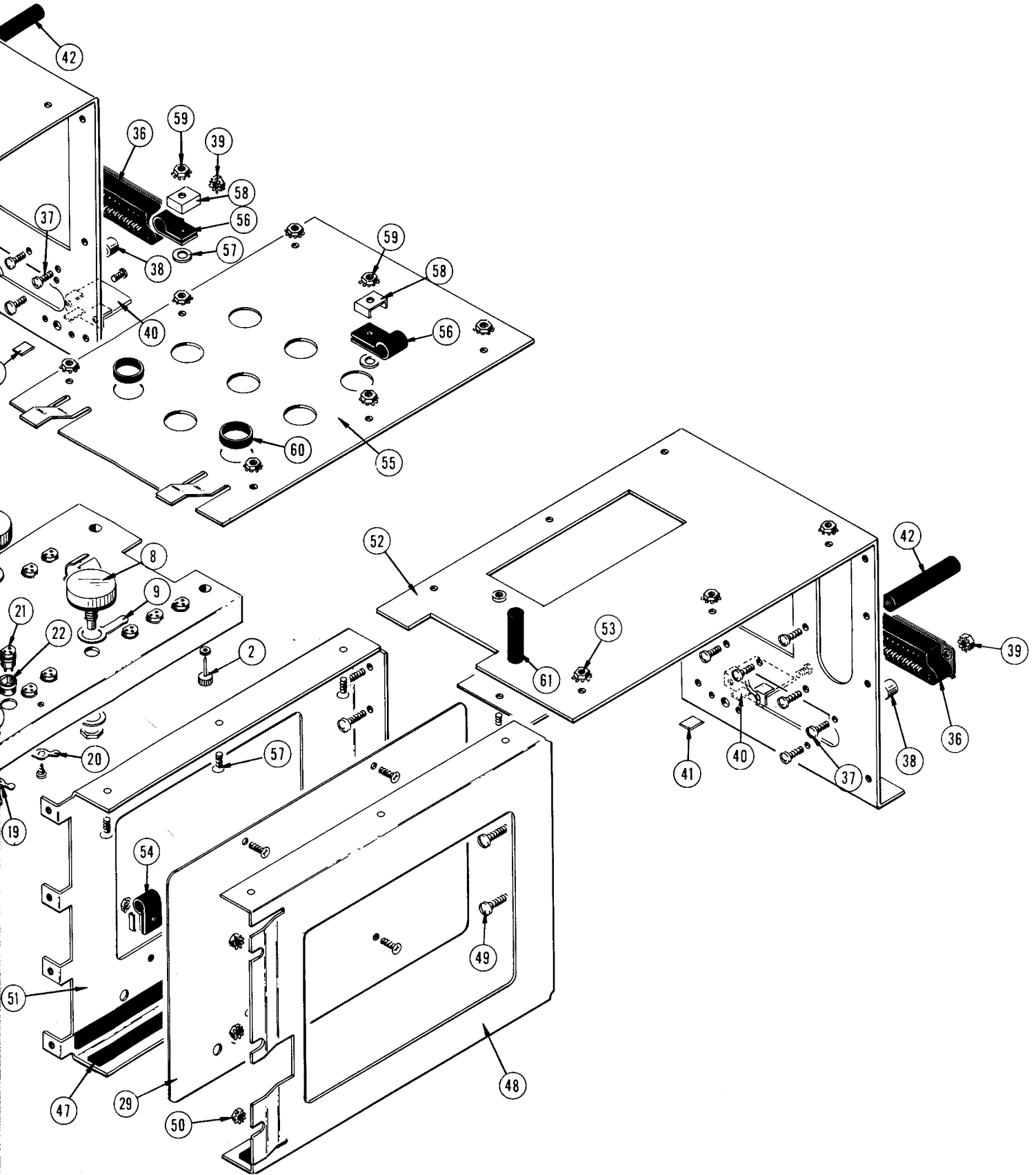
TYPE 556 OSCILLOSCOPE
