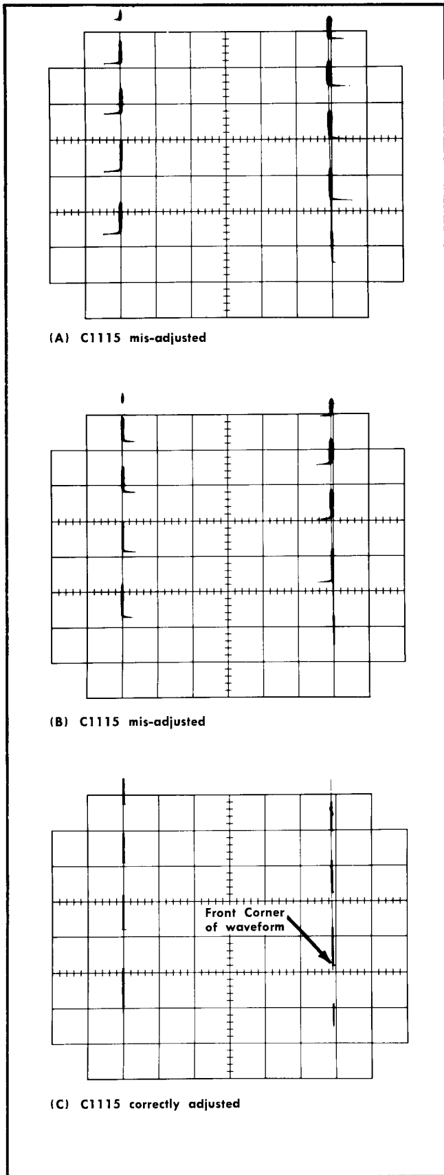
Fig. 6-55. Horizontal Amplifier \times 1 - \times 10 Compensation—Upper Beam.
