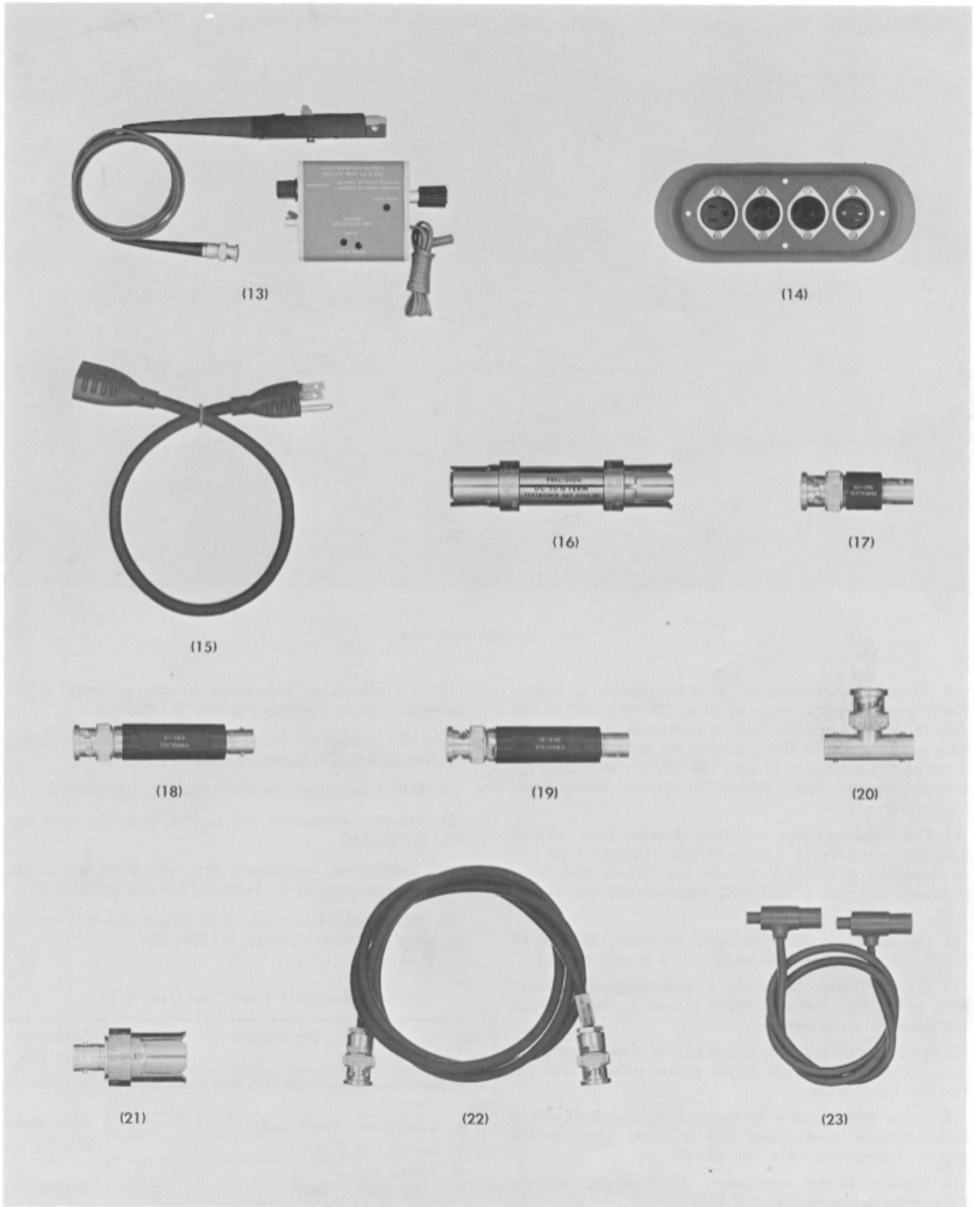
Fig. 6-2. Recommended calibration equipment. Items 13 through 23.
