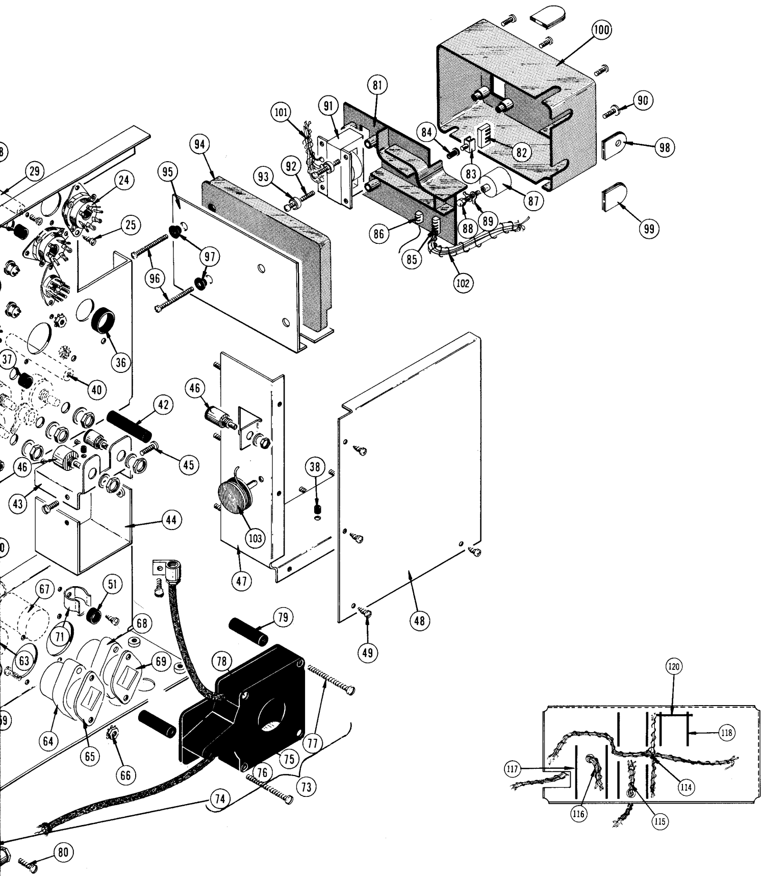
TYPE 556 OSCILLOSCOPE
