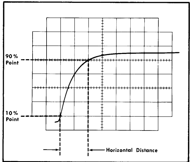
Fig. 2-23. Measuring risetime.
