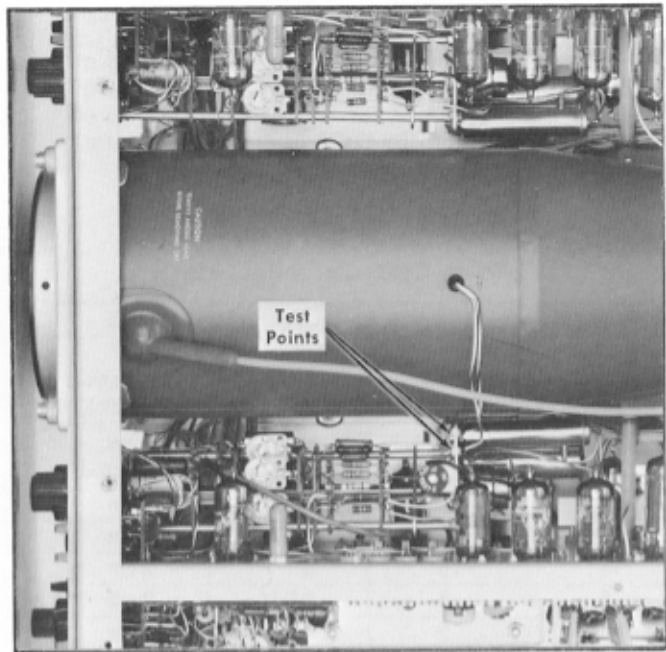
Fig. 6-16. Location of trace rotation coil test points.
