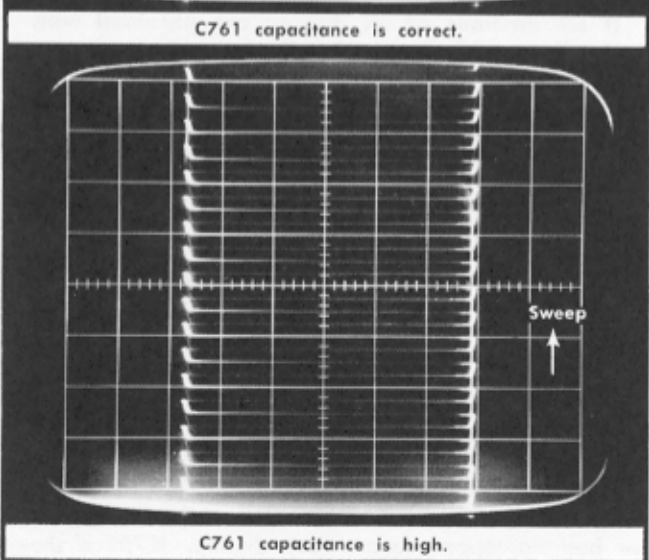
Fig. 5-18. Waveforms for step 9b.
