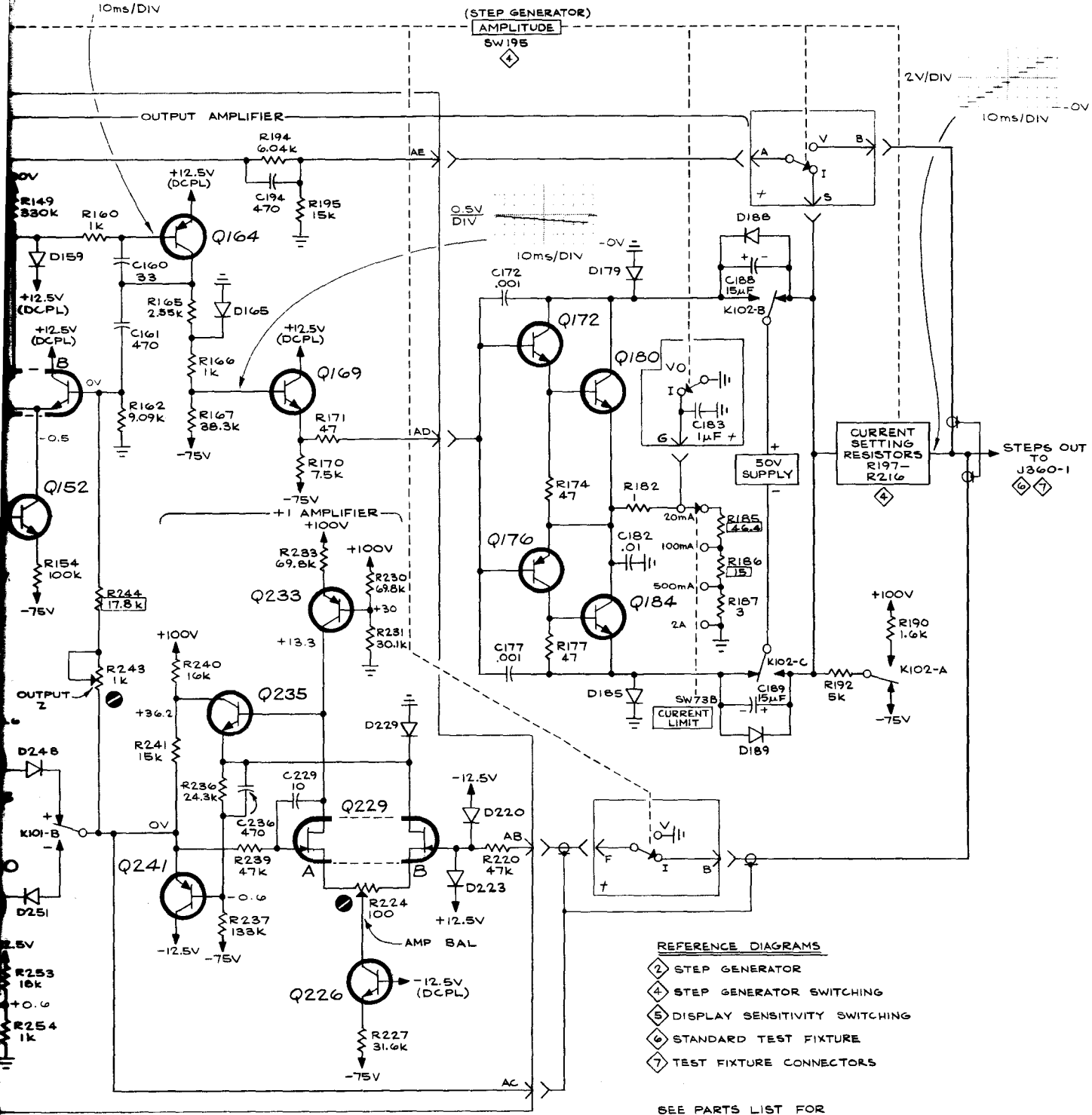
PARTIAL STEP GENERATOR BOARD
