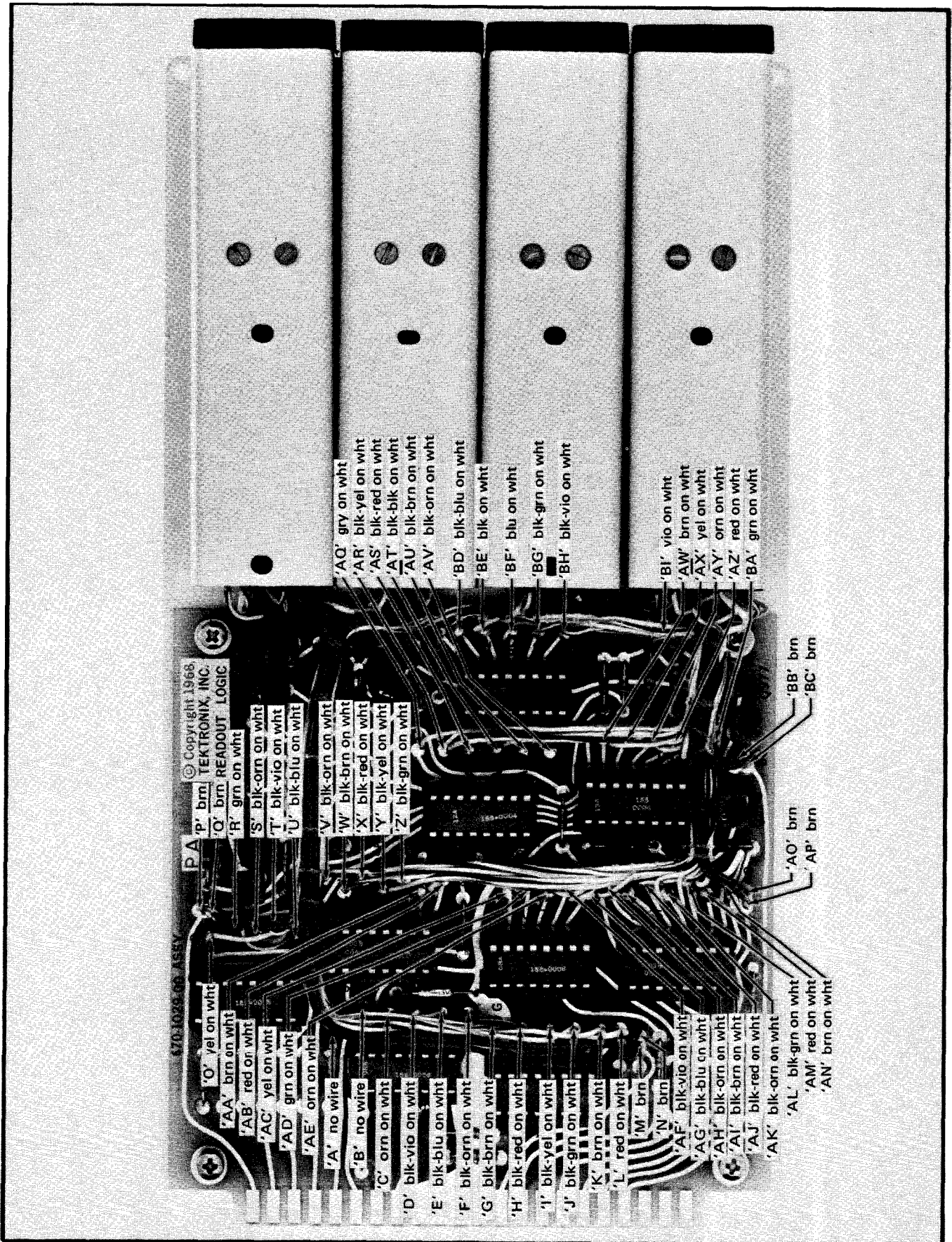
Fig. 4-21. Wiring color codes on Readout logic circuit board.
