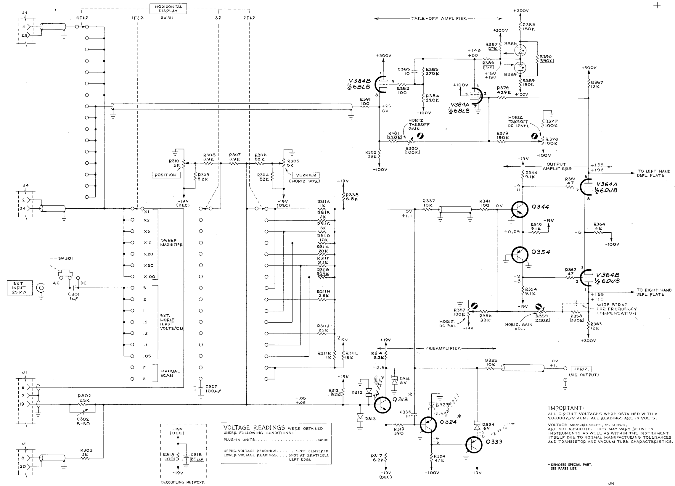
TYPE 661 OSCILLOSCOPE
