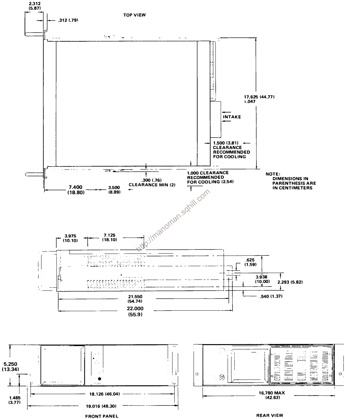
Fig. 6-6. Dimensional drawing.
