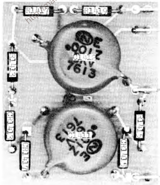
C1410 mounted on back of board.
