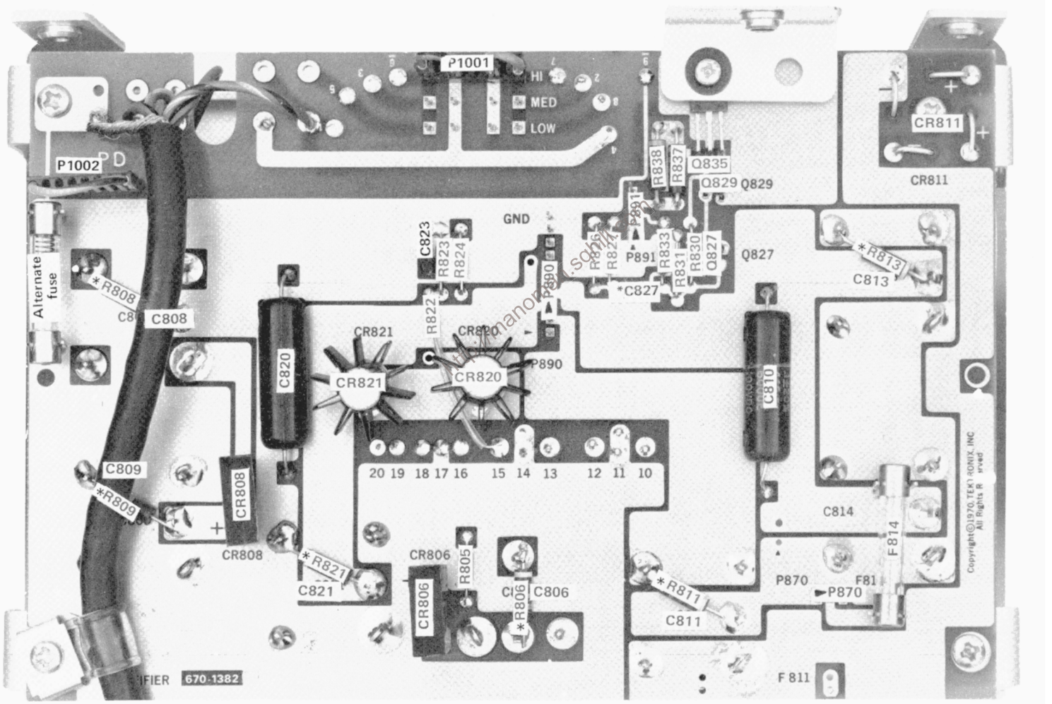
Fig. 8-13B. A10. Rectifier circuit board below B061550.
