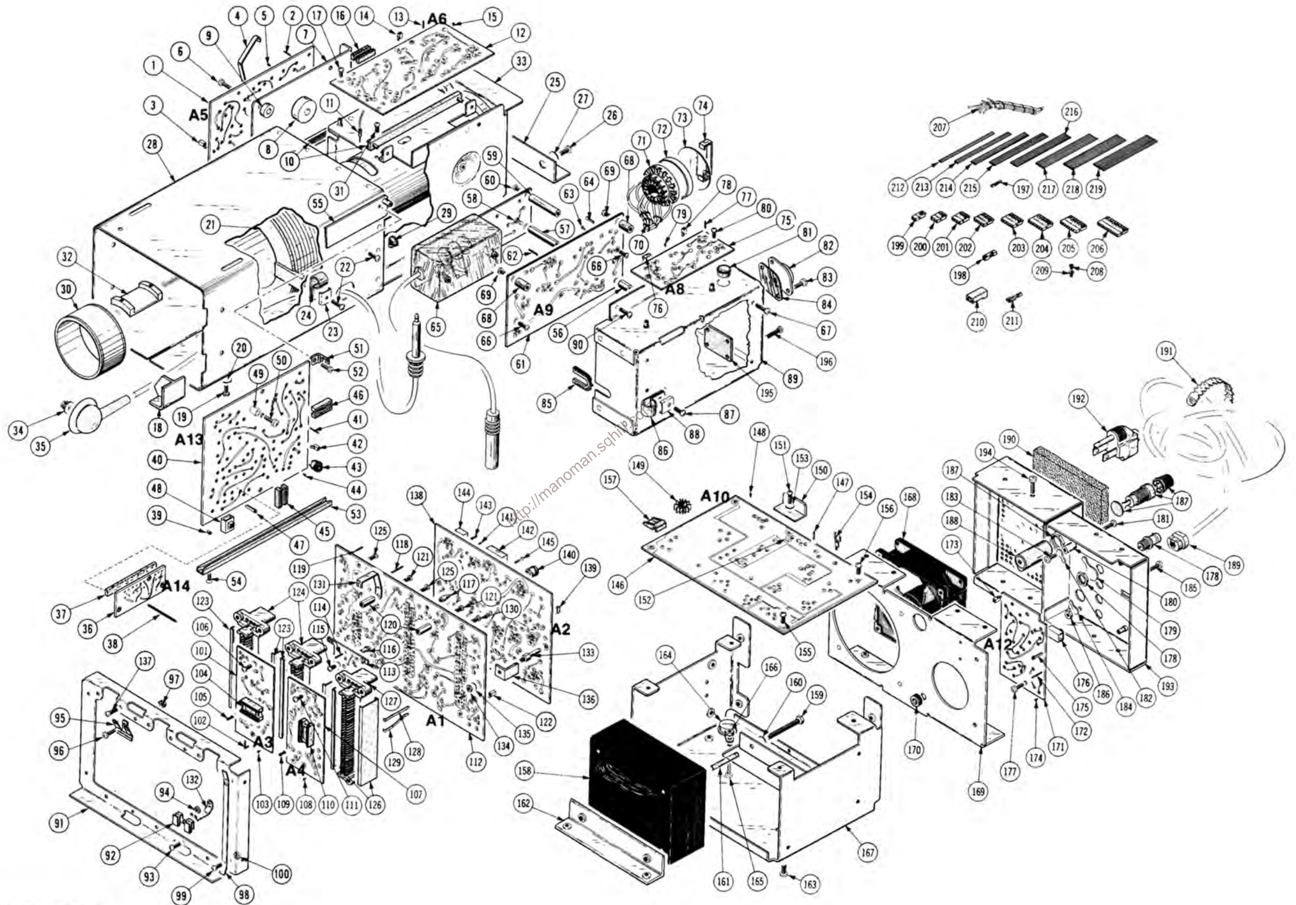
7603/R7603 OSCILLOSCOPE
