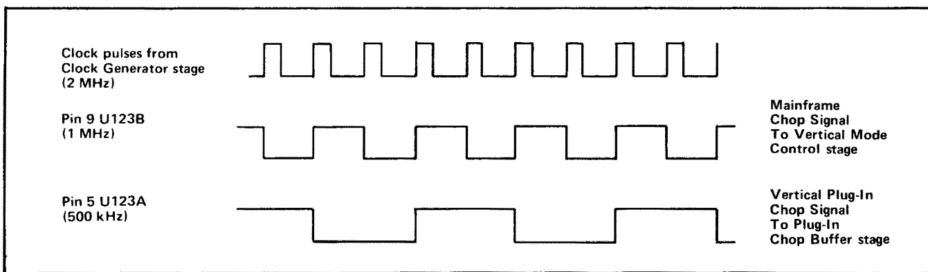
Fig. 4-8. Idealized input and output waveforms for Chop Counter stage.
