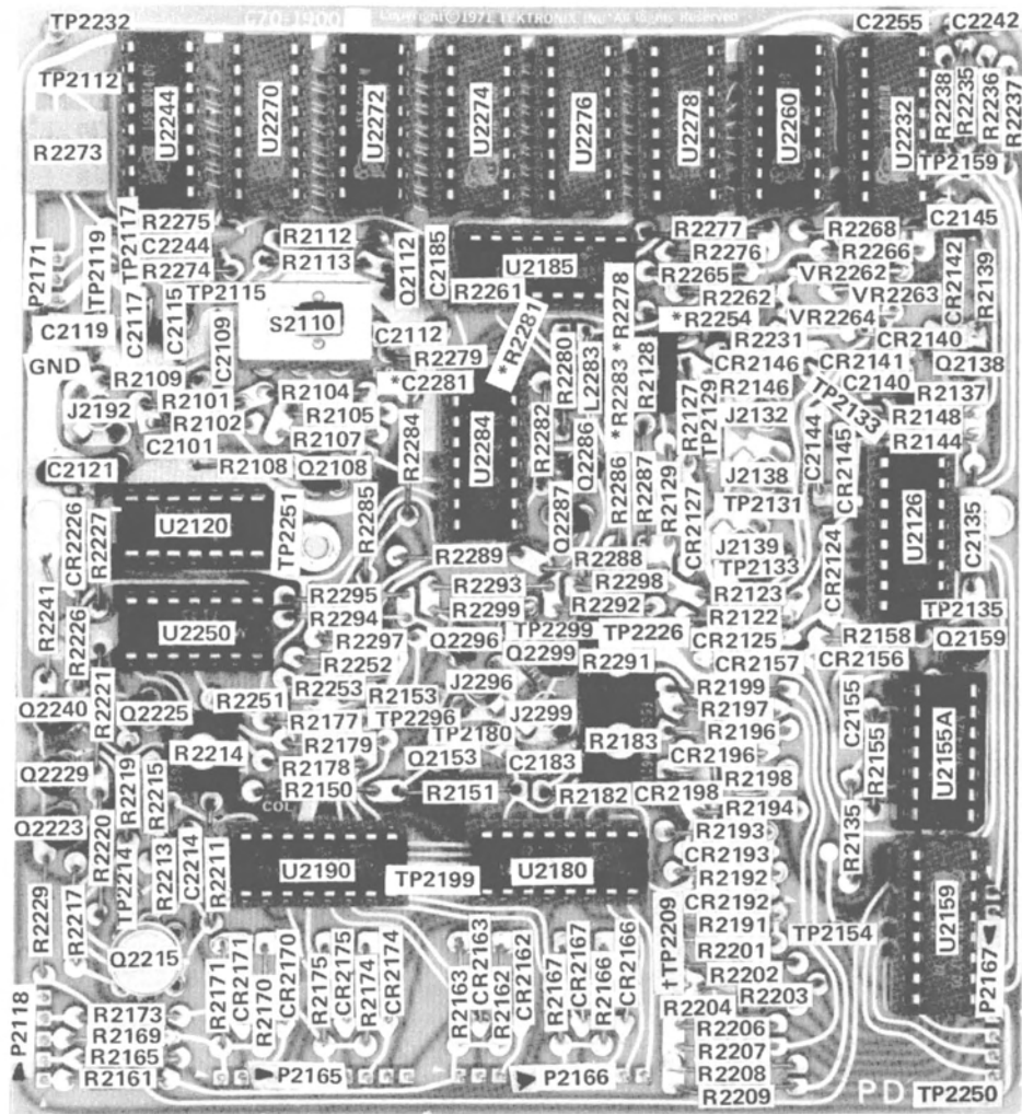
Fig. 8-14. A13. Readout circuit board.
