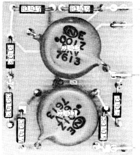
C1410 mounted on back of board.
