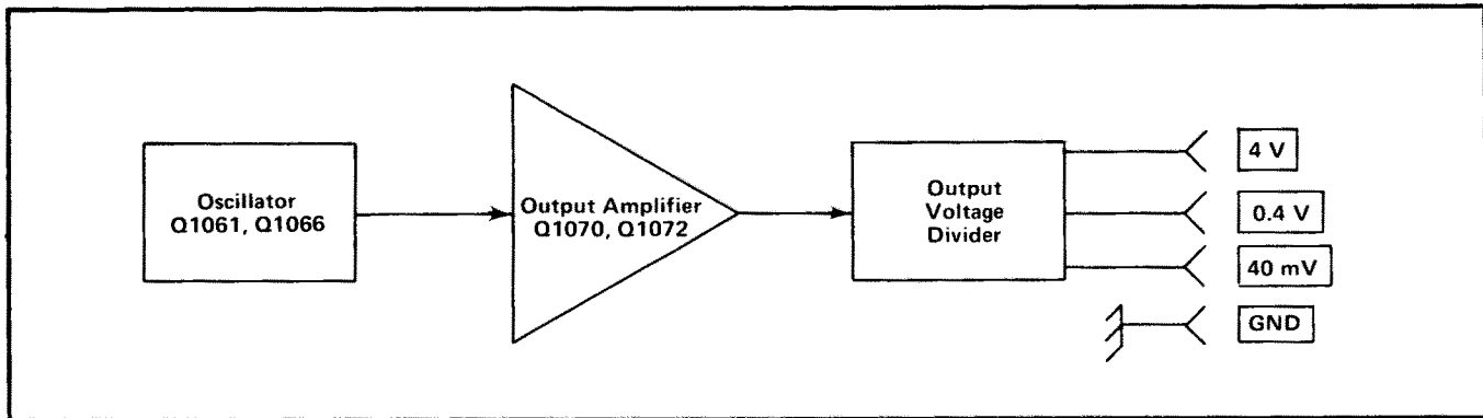
Fig. 4-20. Calibrator detailed block diagram.
