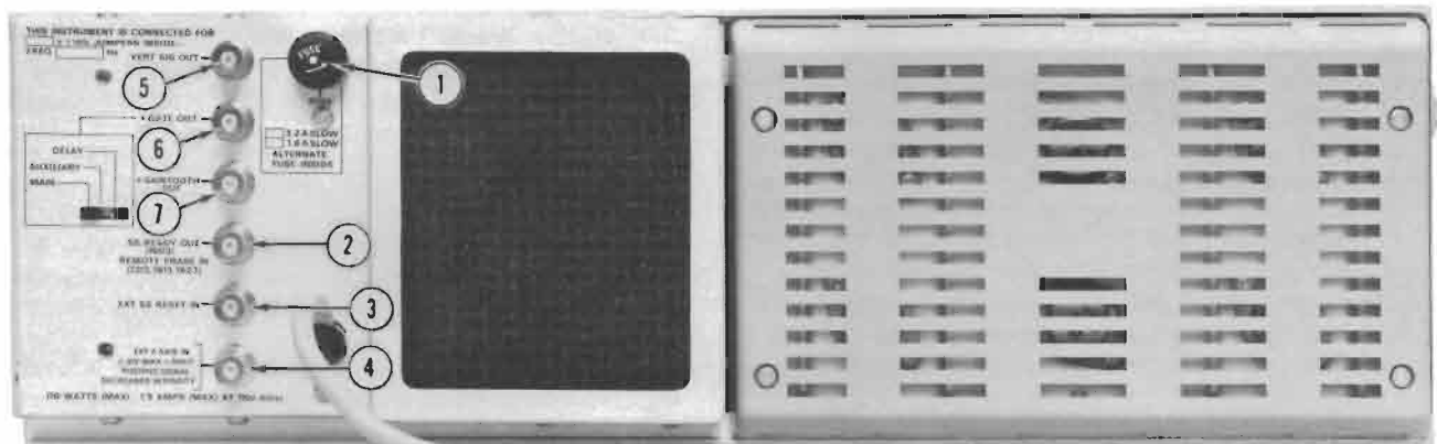
Fig. 1-3. Rear-panel controls and connectors.
