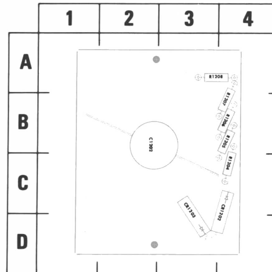
Figure 8-11. A9-Anode board.
