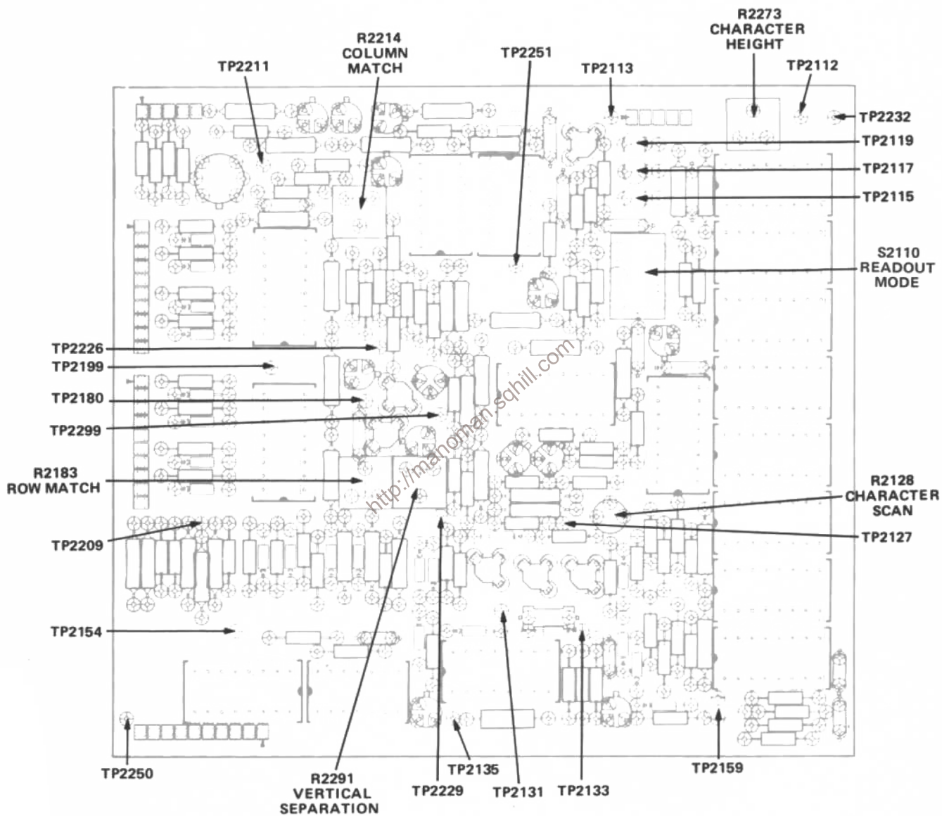
Figure 8-23. Readout board.
