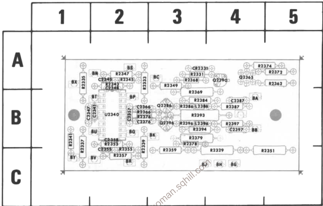
Figure B-5. A4-Vertical Interface board.
