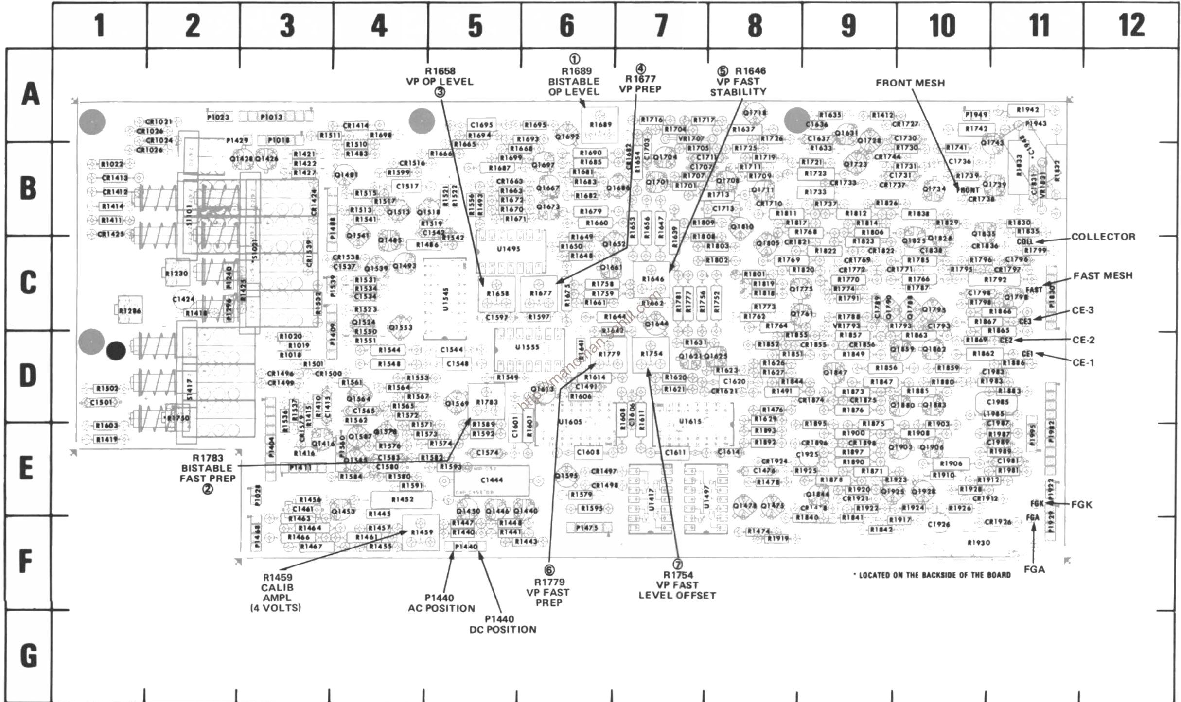
Figure 8-16. A14-Storage board.
