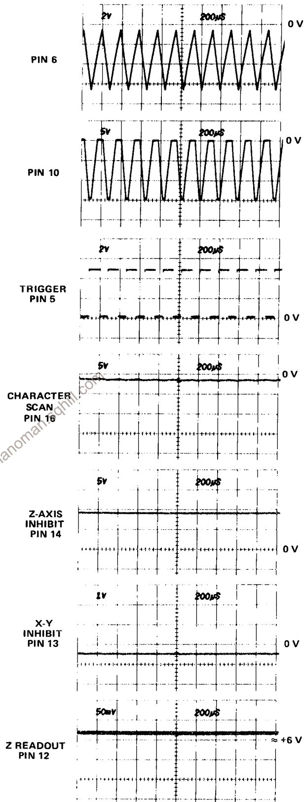
NOTE: TEST OSCILLOSCOPE EXTERNALLY TRIGGERED FROM TP2251.
