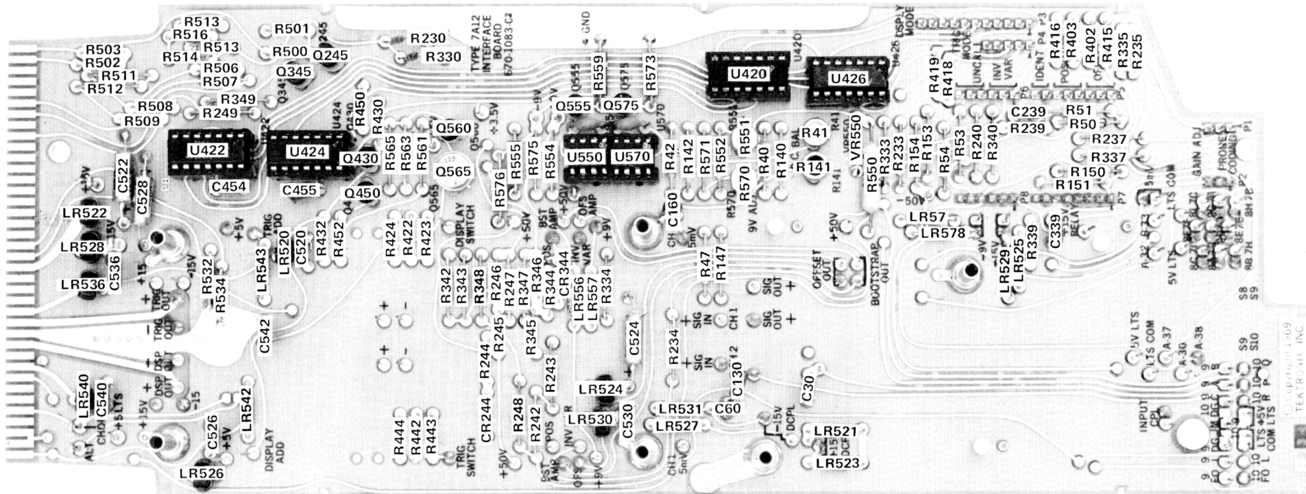
Fig. 7-5. Interface circuit board showing location of components.
