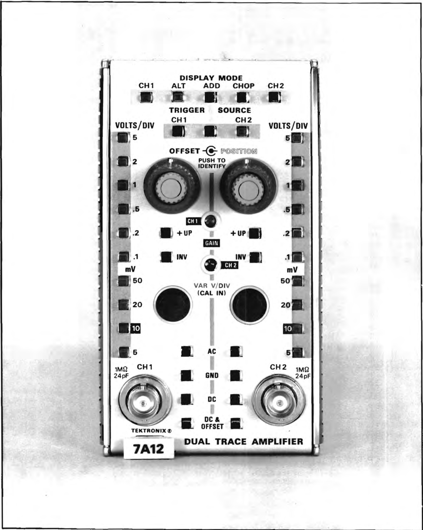
Fig. 2-1. Front-Panel Controls and Connectors.
