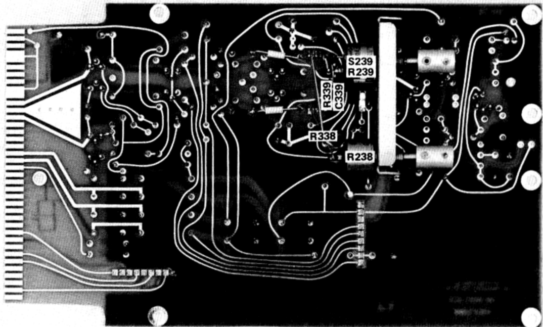
Fig. 7-2. Amplifier circuit board and component location.
