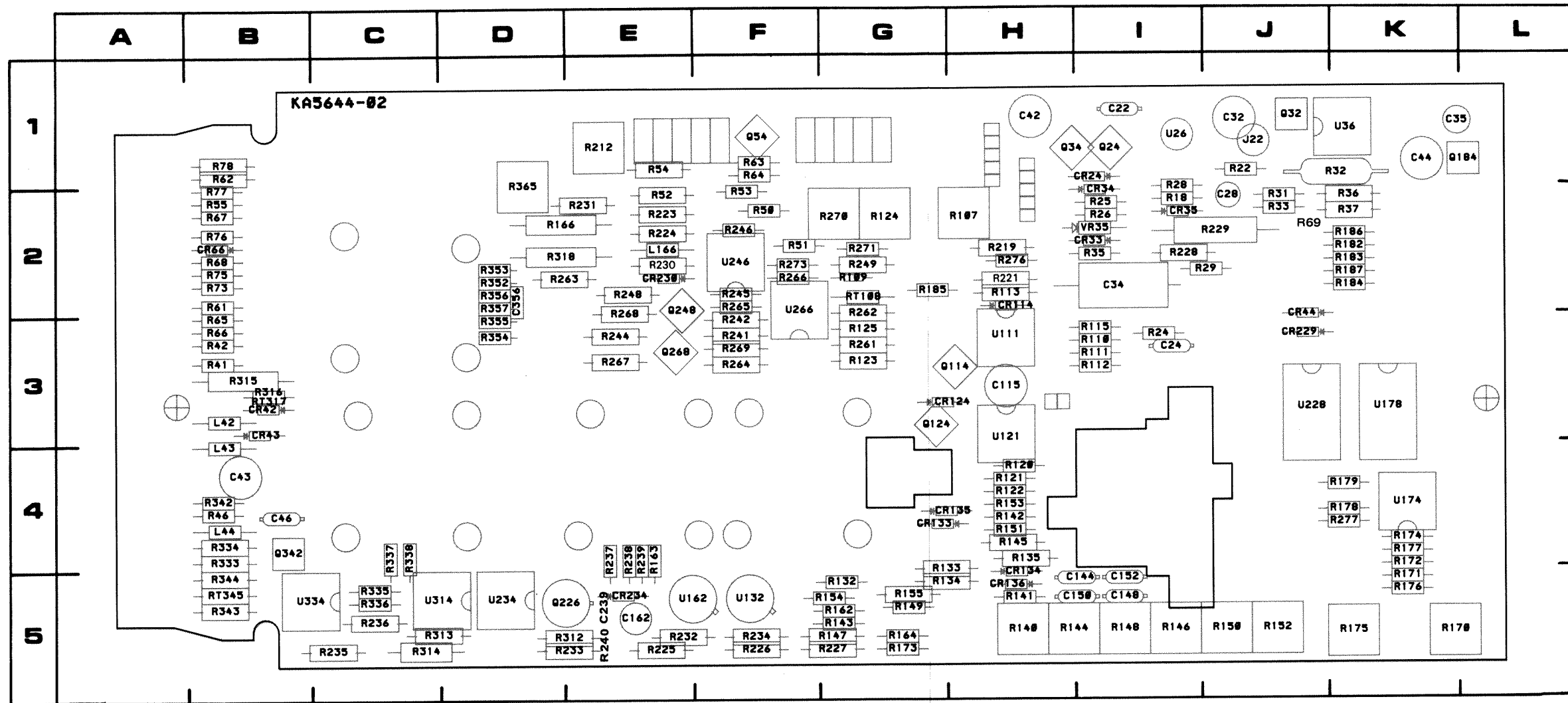
Figure 8-3. A1—Main circuit board assembly.
