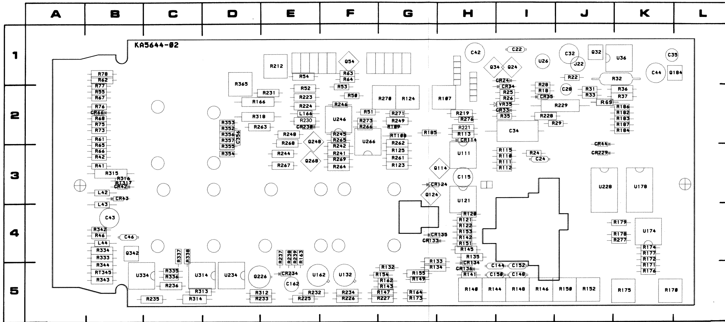
Figure 8-7. A1—Main circuit board assembly.
