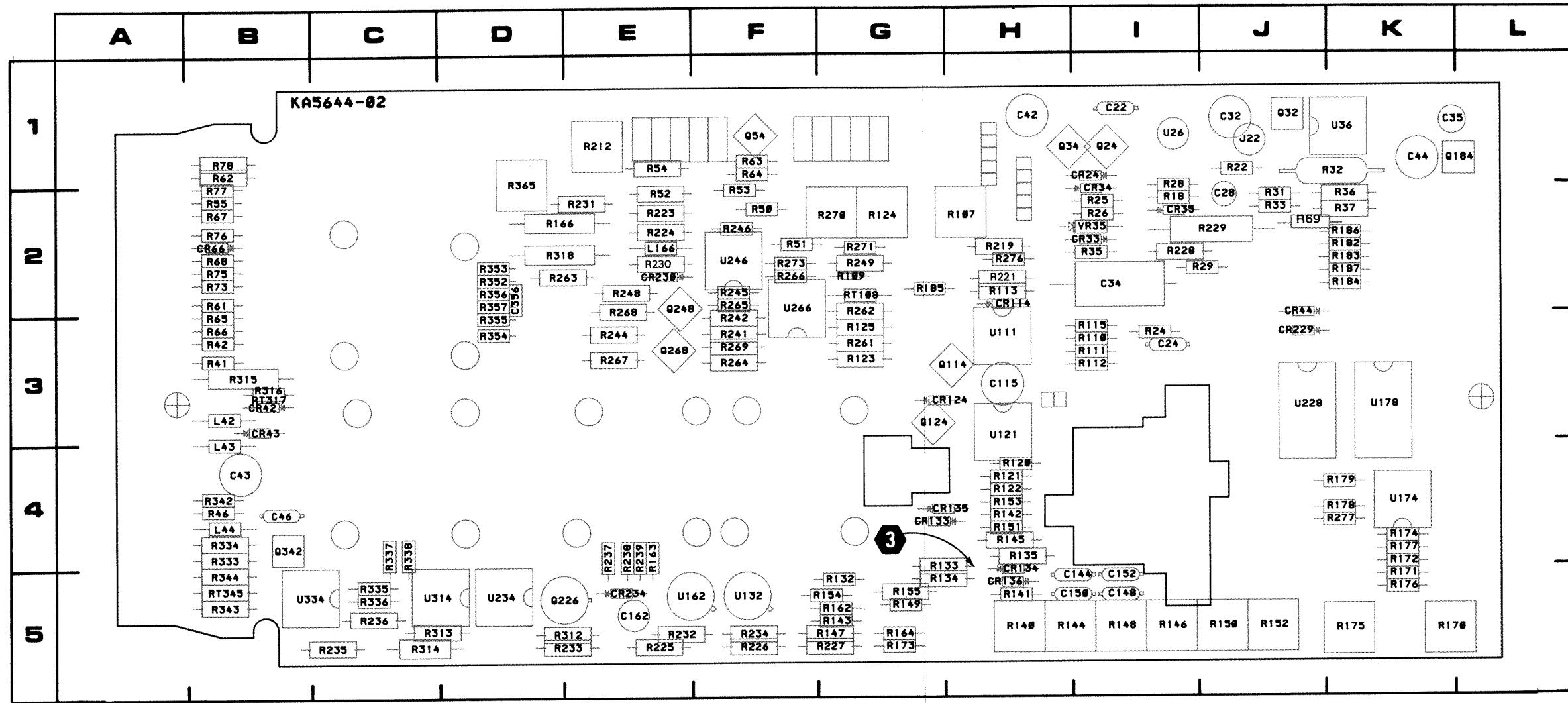
Figure 8-5. A1—Main circuit board assembly.
