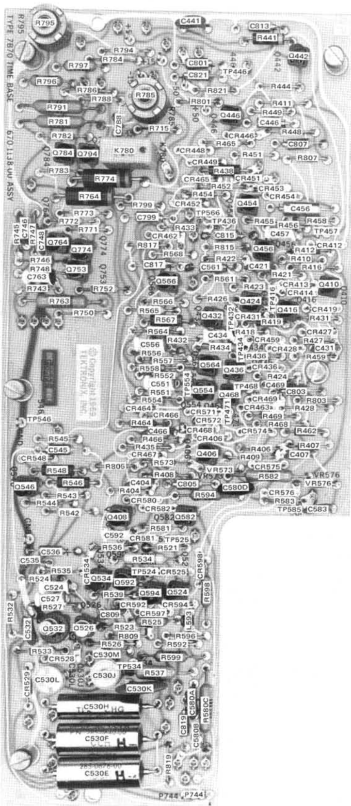
Fig. 4-5. Time Base board showing location of components.
