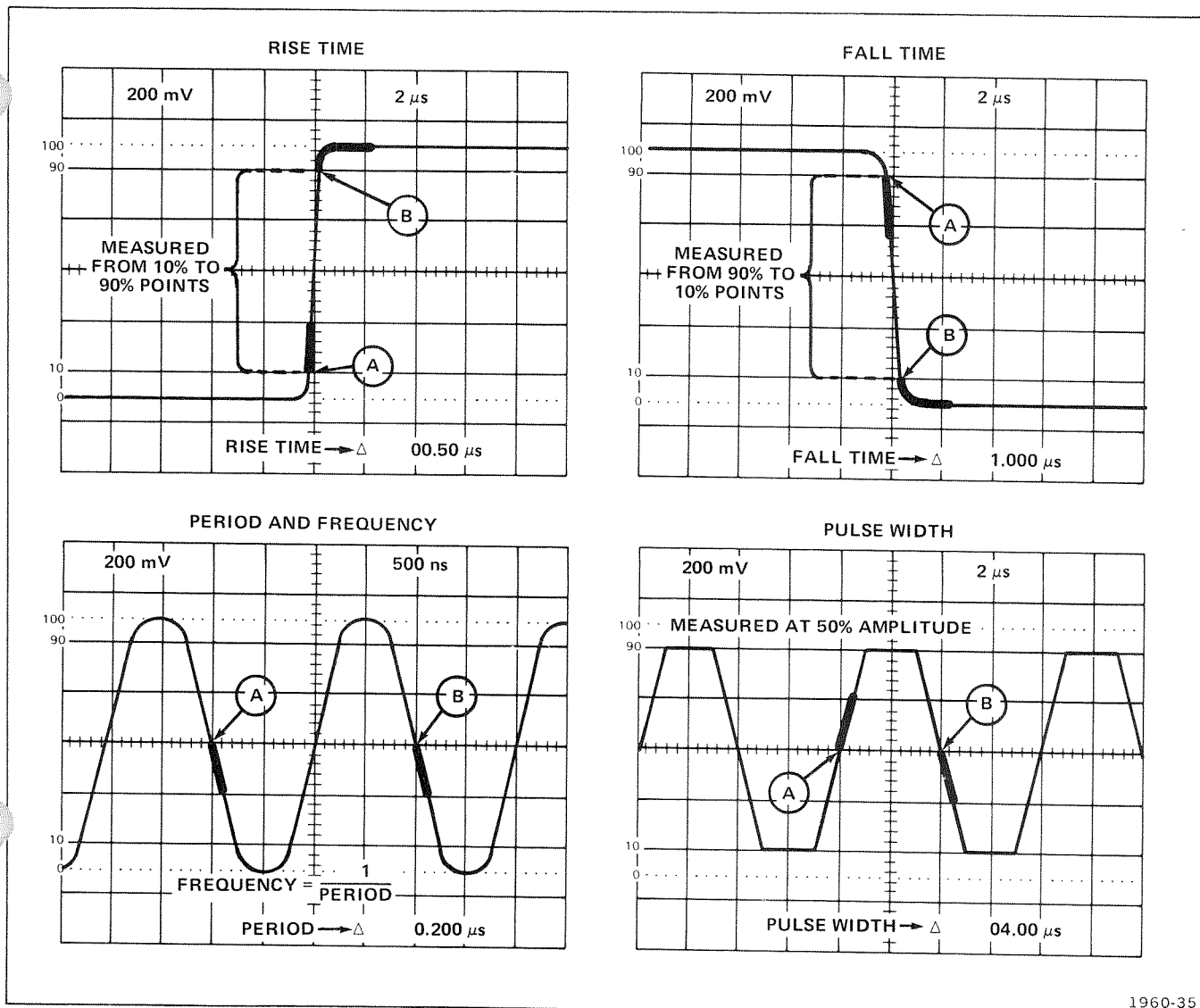
Fig. 1-9. Measuring rise time, fall time, period, frequency, or pulse width in the \Delta (differential) time mode.
