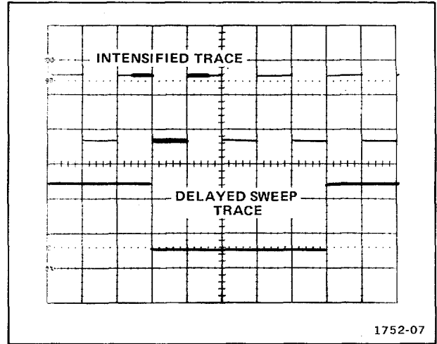
Figure 2-6. Typical alternate sweep display.
