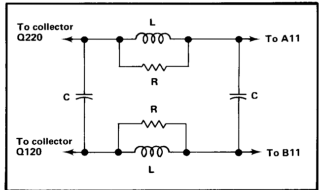
Fig. 9. Bandwidth Limiter.
