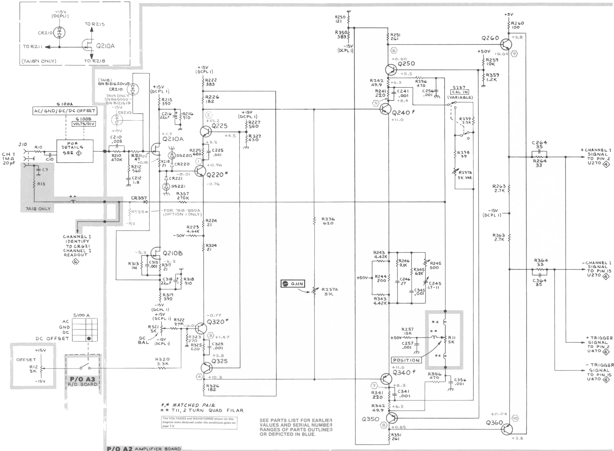
P/O A2 AMPLIFIER BOARD
