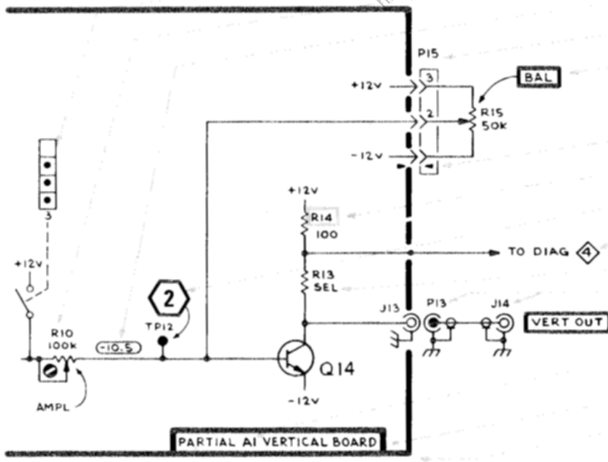
VERTICAL AMPLIFIER 2 LMD 12.74
