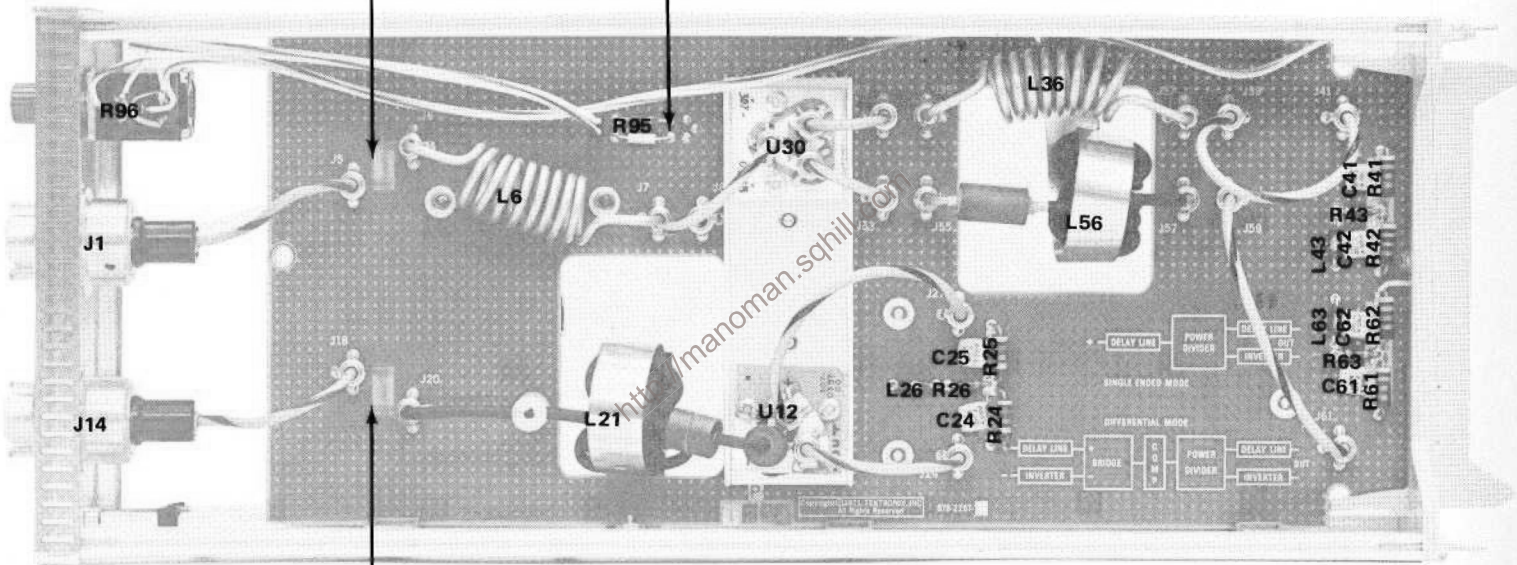
7A21N component location.
