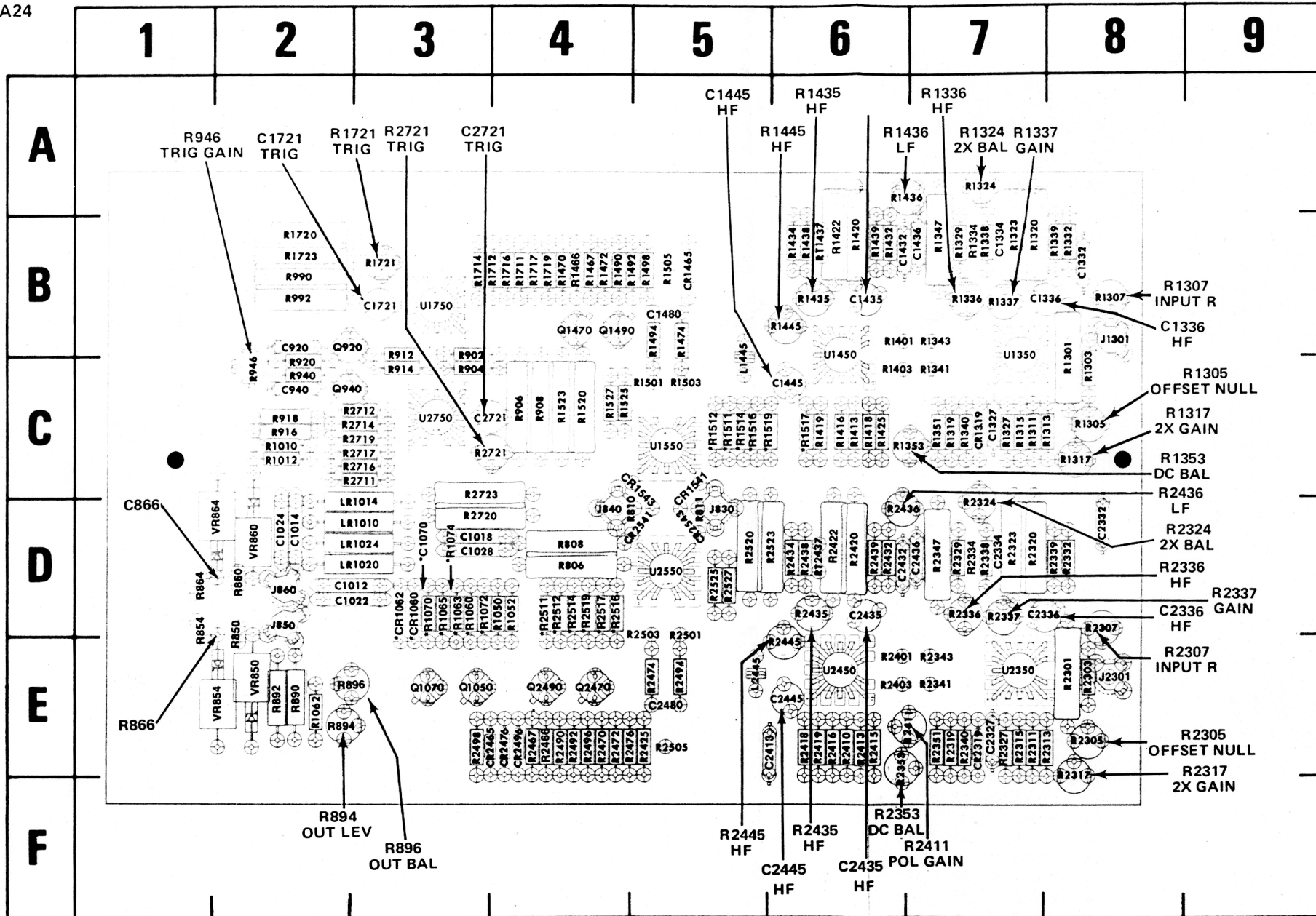
Fig. 7-6. A5—Amplifier circuit board.
