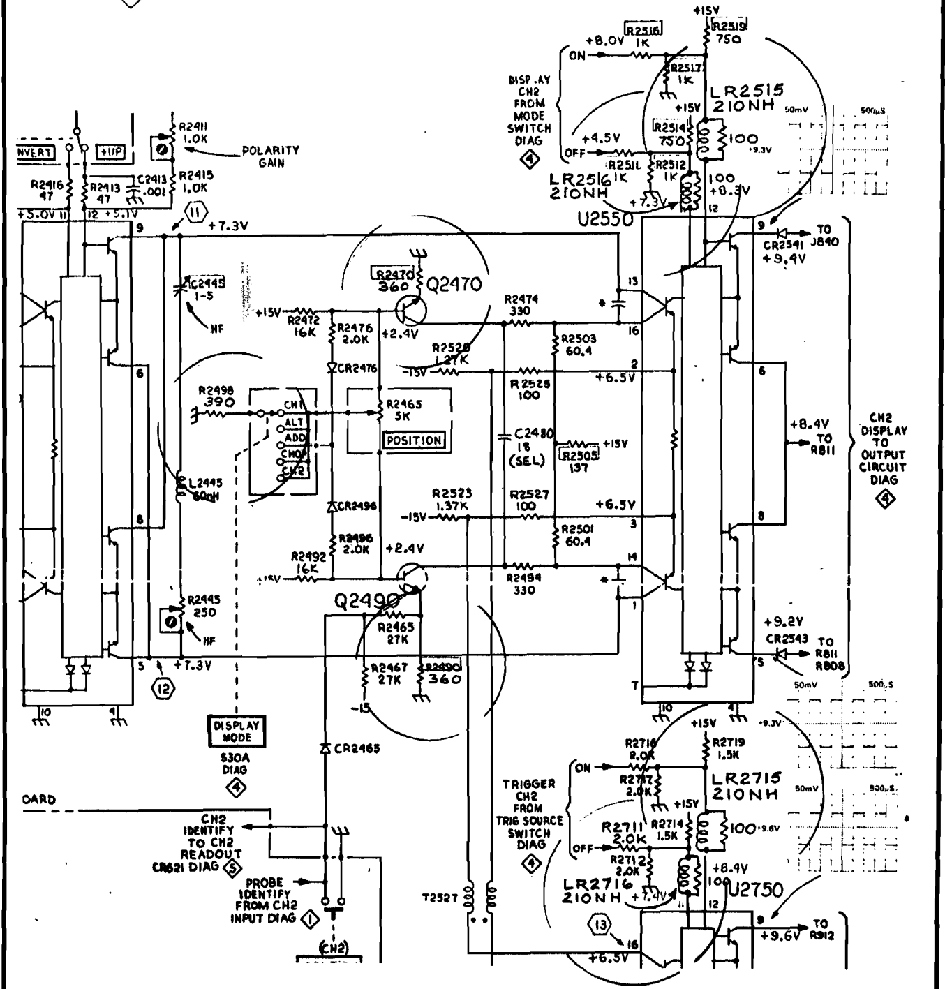
DIAGRAM 3 CH 2 AMPLIFIER - Partial
