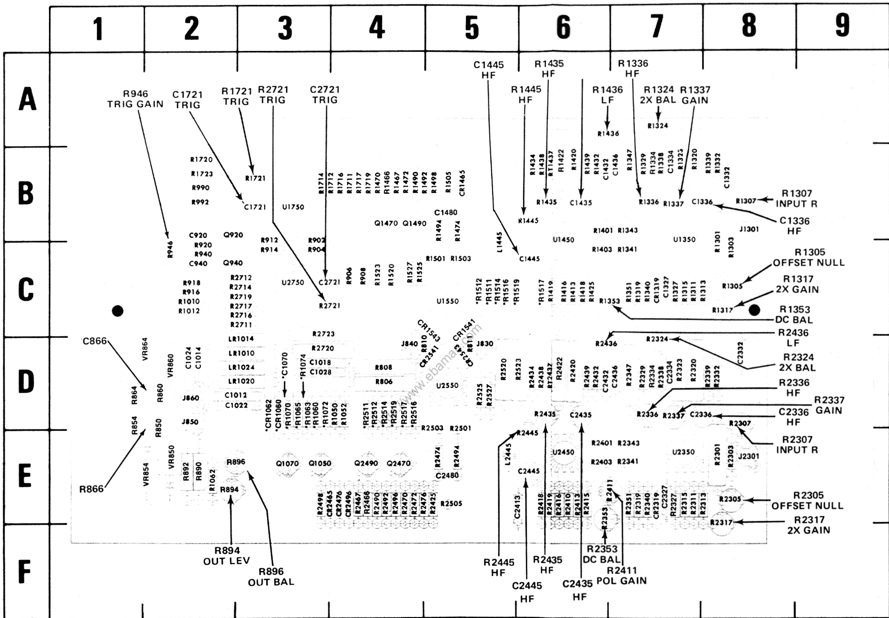
Fig. 7-4. A5—Amplifier circuit board.
