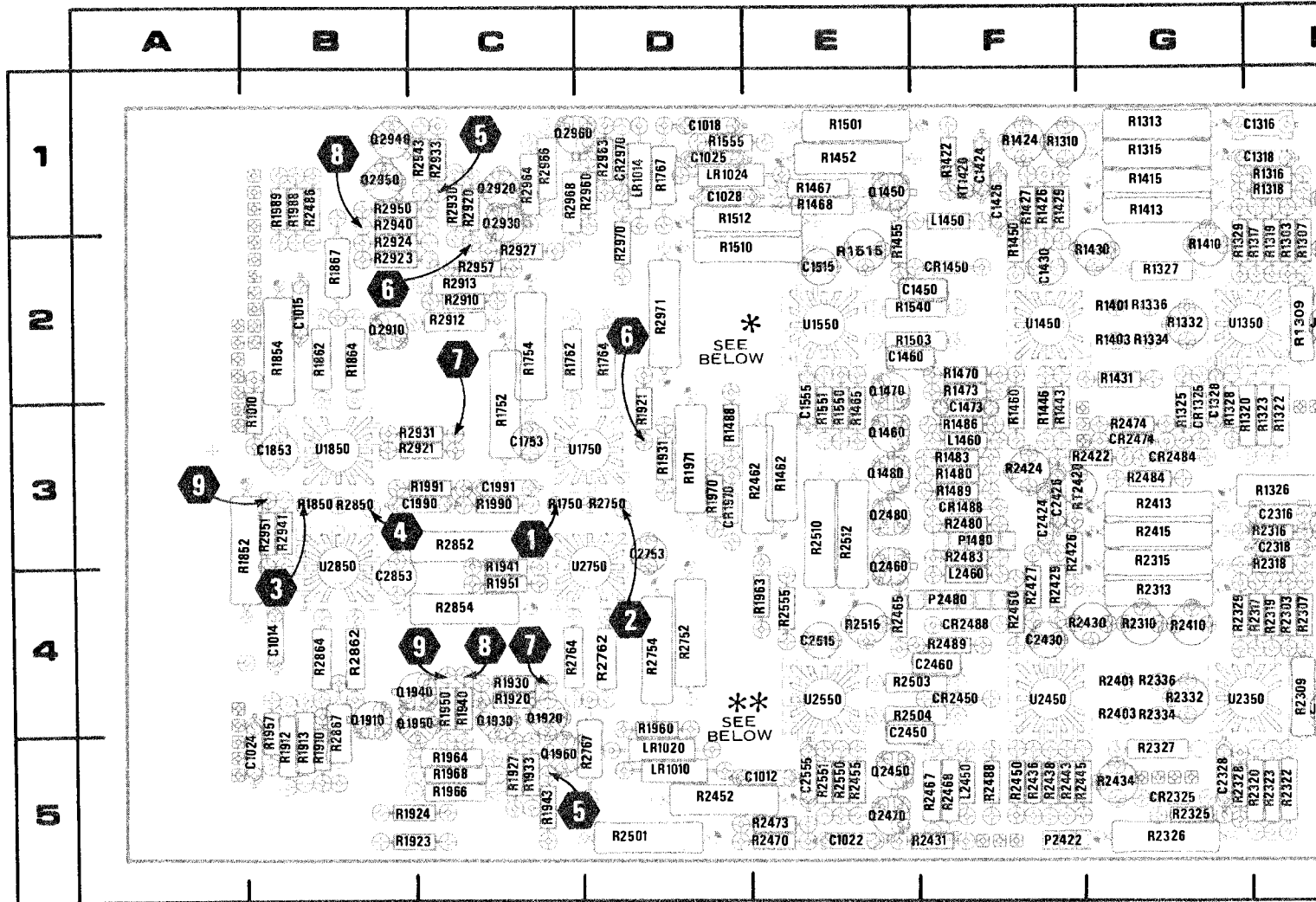
Figure 8-5. A5 and A6—Amplifier circuit board assembly.
