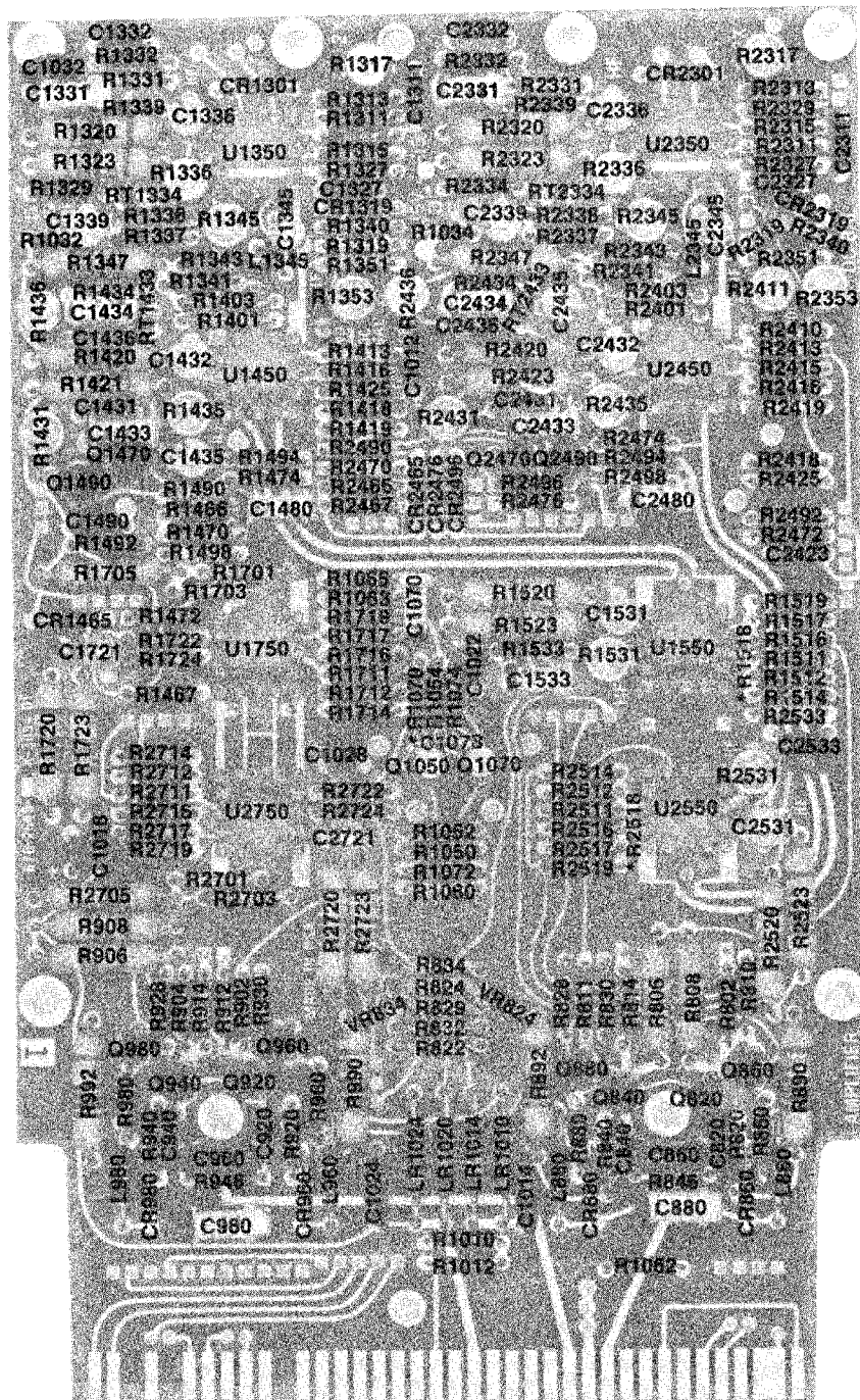
A2 Amplifier Board, SN B16000-above.
