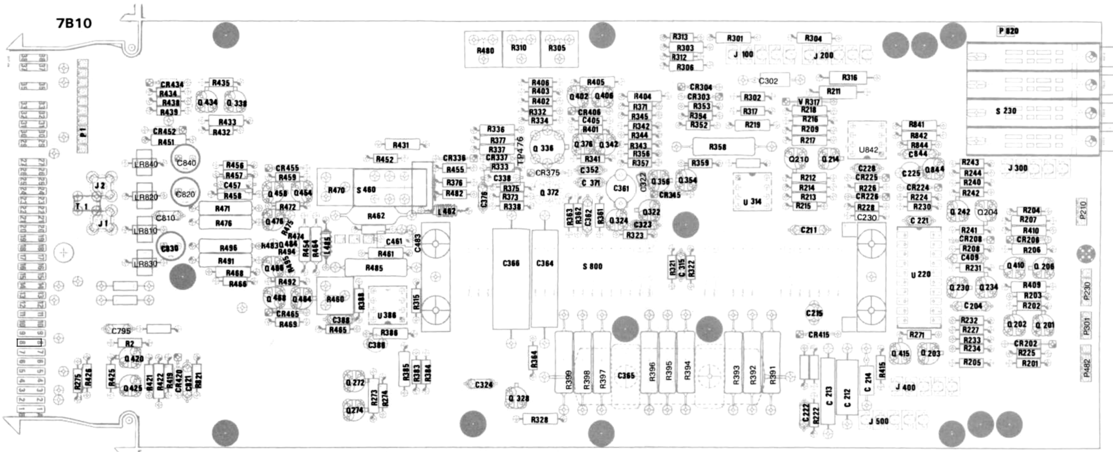
Figure 8-3. A1-Interface circuit board assembly.
