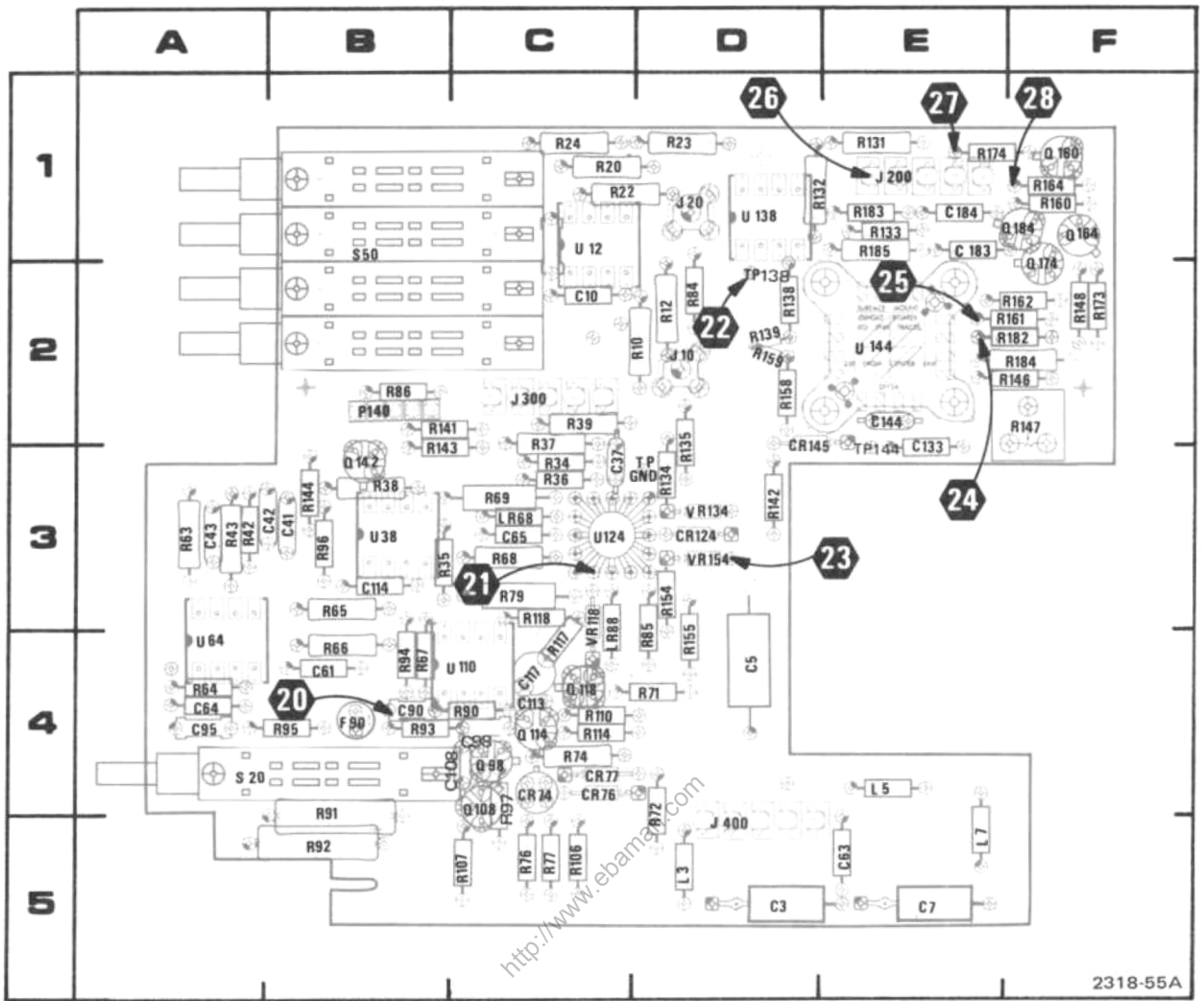
Figure 8-4. A2-Trigger circuit board assembly.
