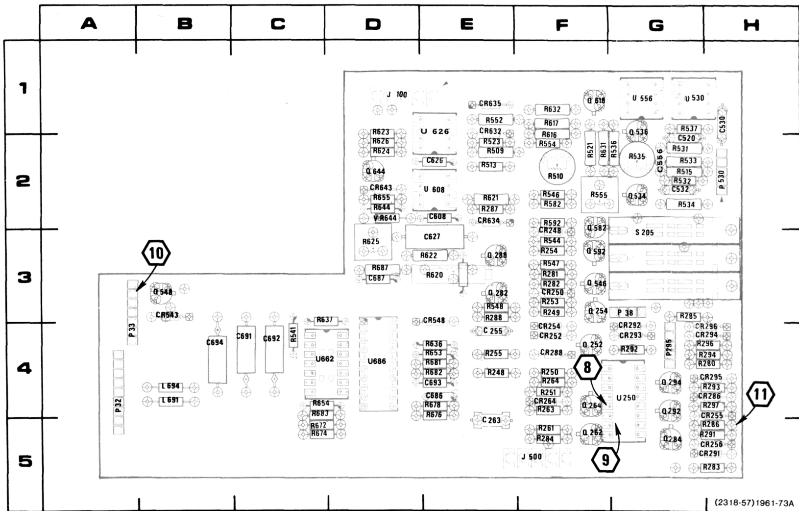
Fig. 8-3A. A4-Digital Voltmeter circuit board assembly (SN B088750 & up).
