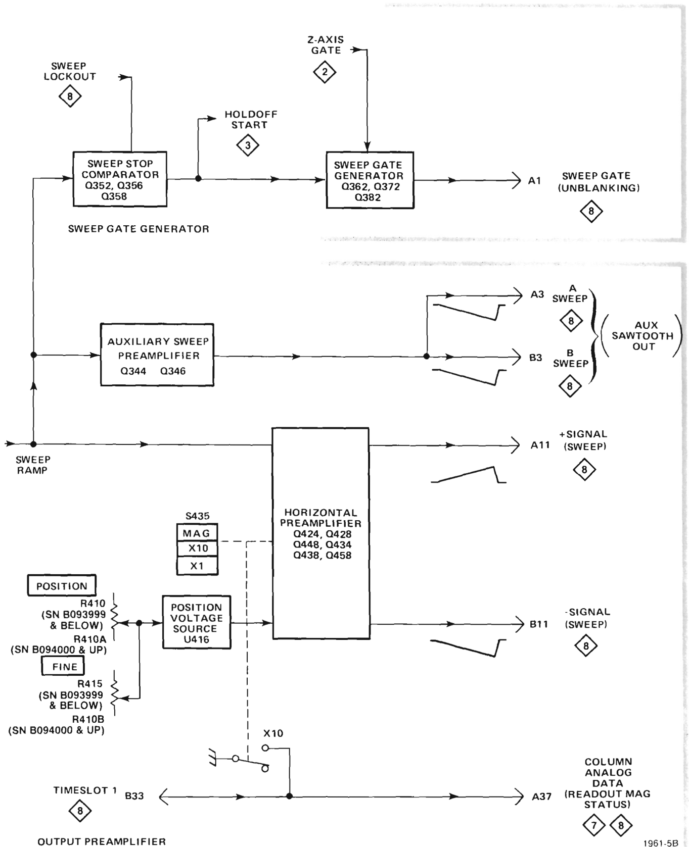
Fig. 3-7. Detailed block diagram of Sweep Generator (cont.).
