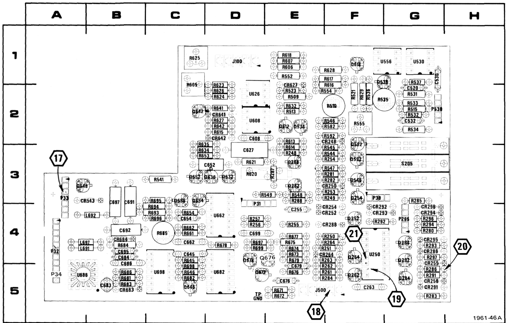
Fig. 8-3B. A4-Digital Voltmeter circuit board assembly (SN B088749 & below).
