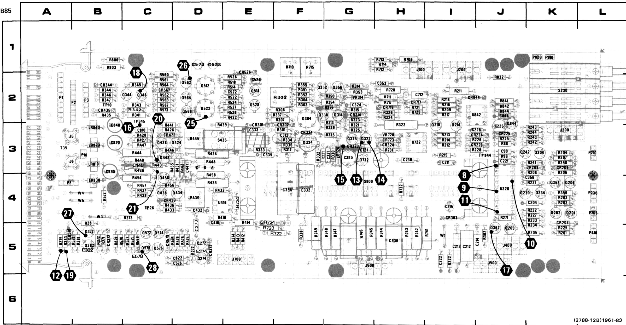
Fig. 8-1A. A1-Interface circuit board assembly (SN B094000 & up).
