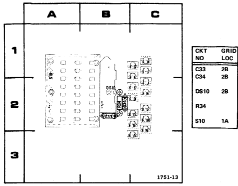
Fig 8-5. A-2--Source Switch Circuit Board.
