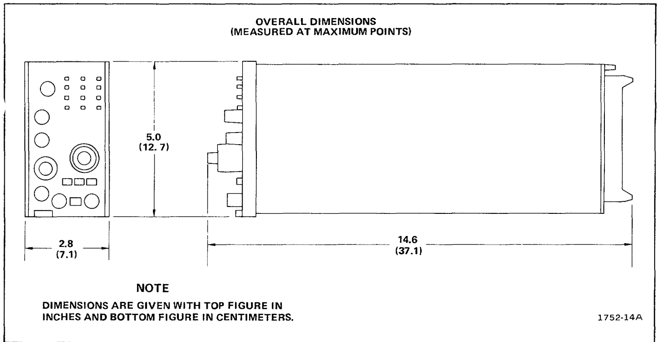
Fig. 2-1. Dimensional drawing.
