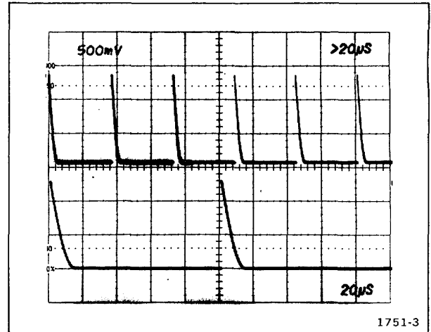
Fig. 5-14. Variable Time/Division Range
