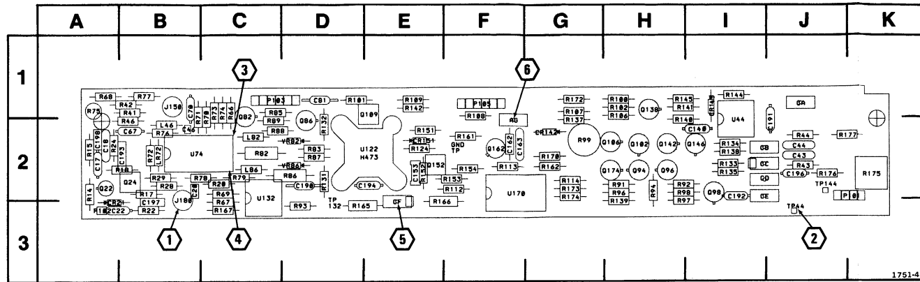
Fig. 8-8. A8—Main Trigger Circuit Board (SN B079999 & up).
