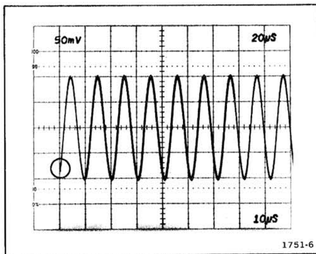
Fig. 5-10. Trigger sensitivity. (Circle denotes correct trigger point.)
