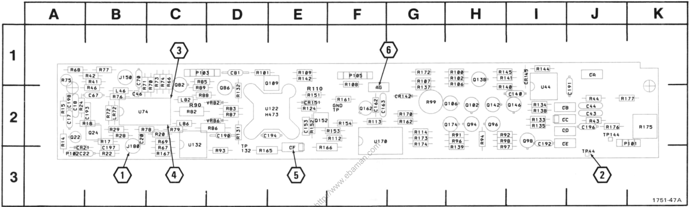
Fig. 8-8. A8—Main Trigger Circuit Board (SN B070000 &amp; up).
