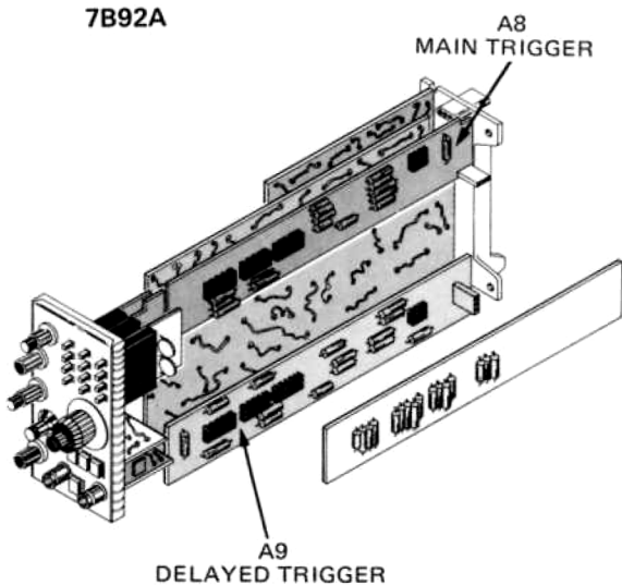
Fig. 8-21. Main Trigger Adjustment Location (SN B070000 & up).
