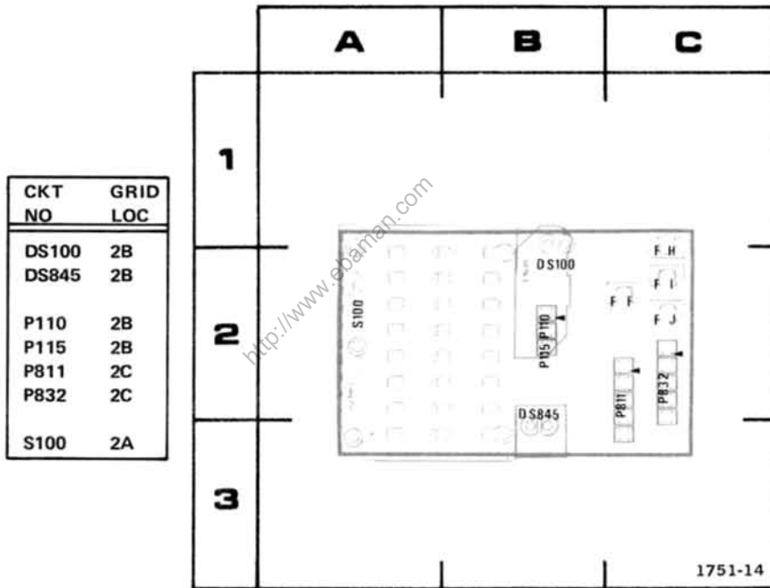
Fig. 8-6. A4—Mode Switch Circuit Board.
