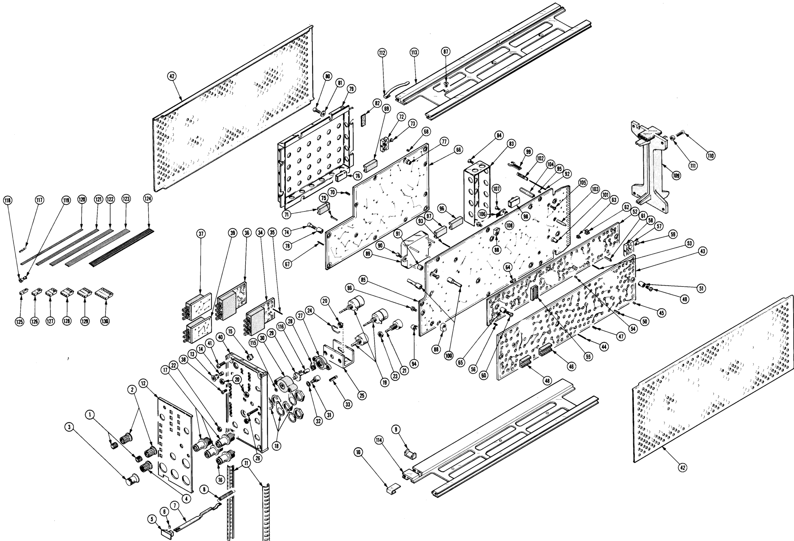
7D11 DIGITAL DELAY
