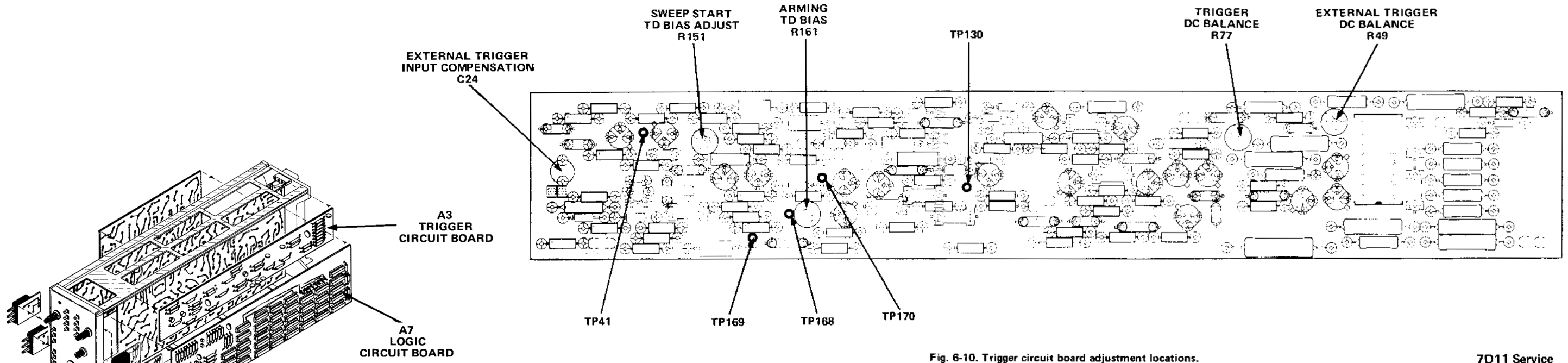
Fig. 6-10. Trigger circuit board adjustment locations.
