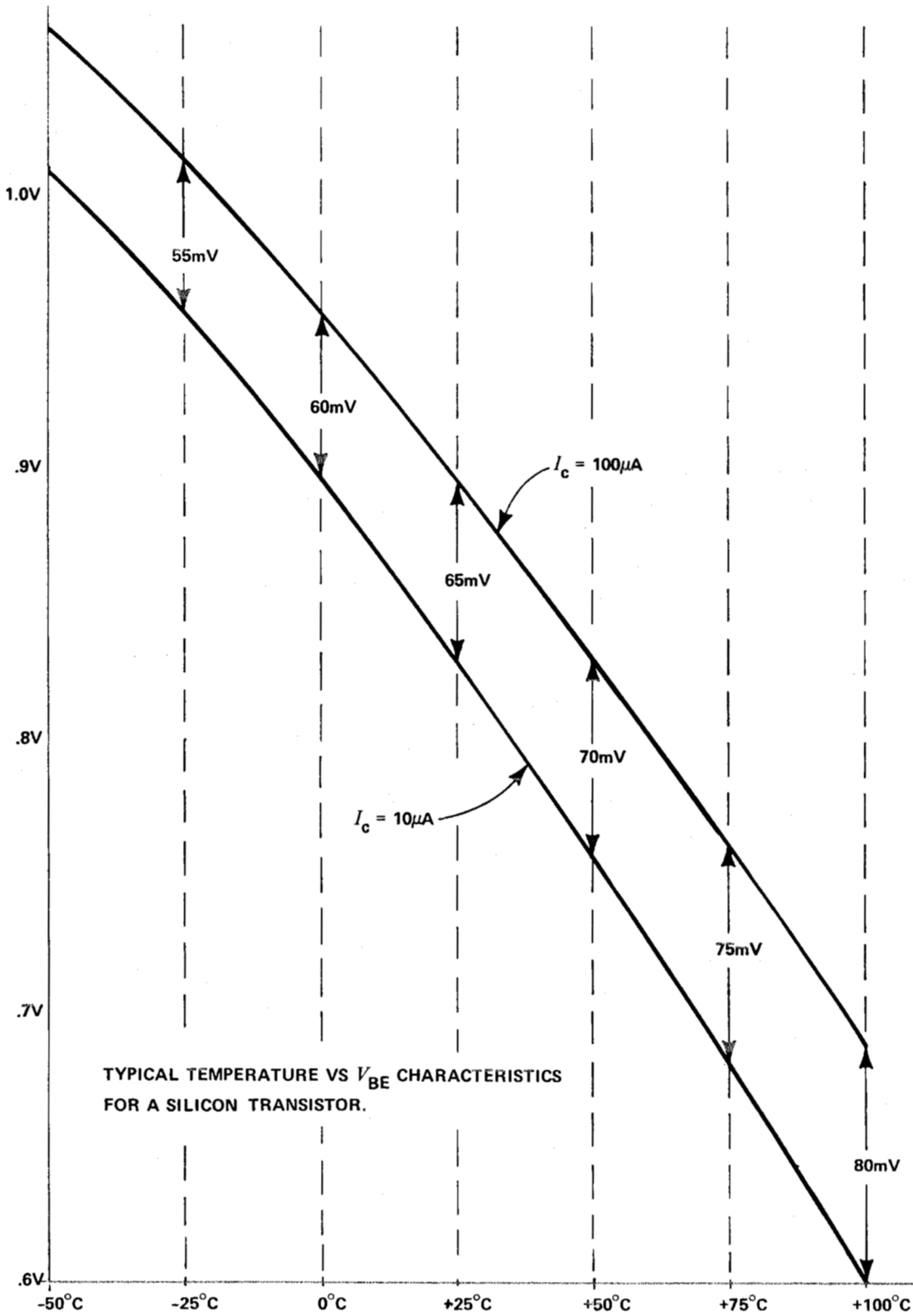
7D13 V_{BE} AS TEMP INDICATOR CHART
