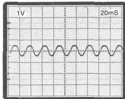
6 MODE: OSCILLATOR
