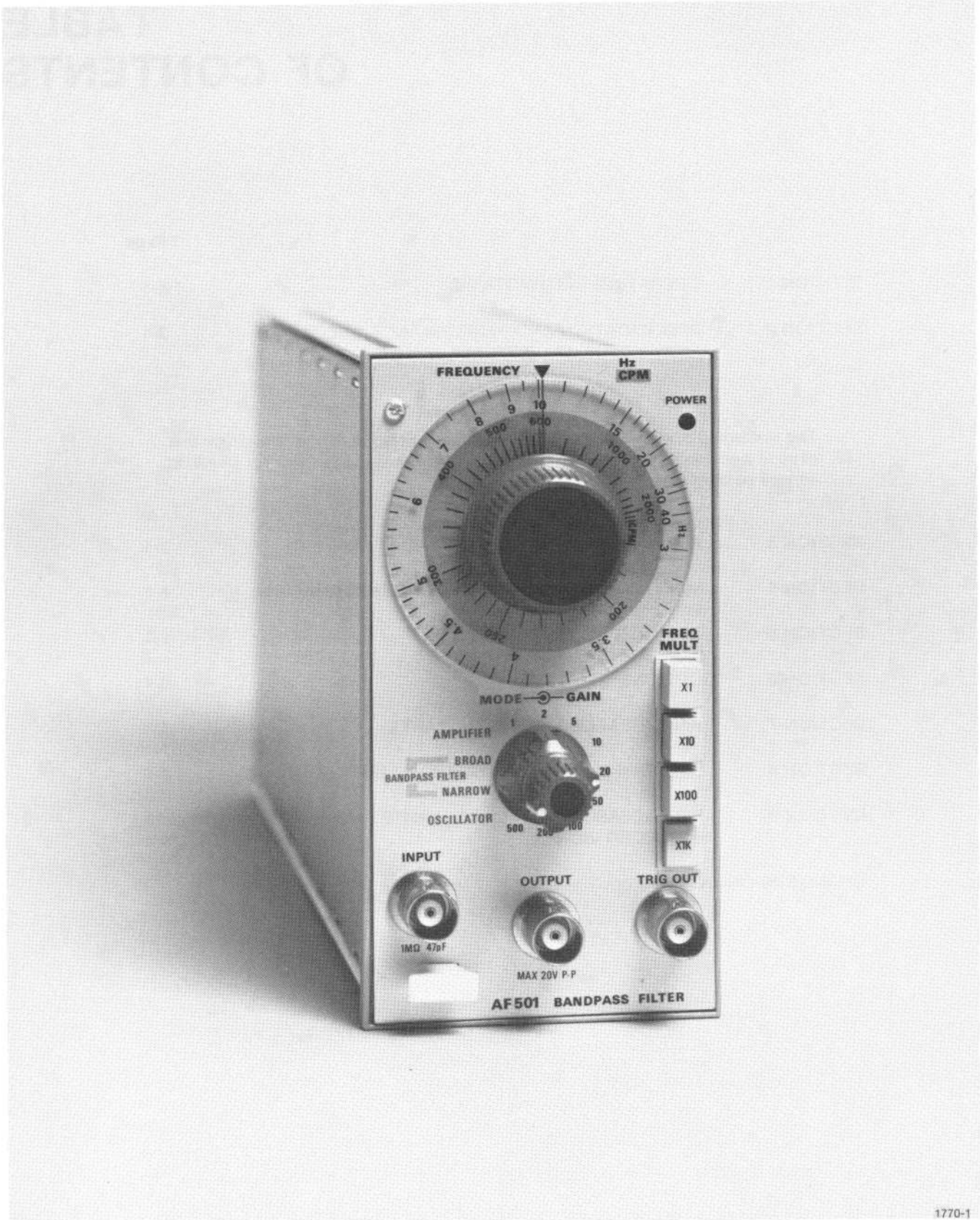
AF 501 Bandpass Filter plug-in unit.
