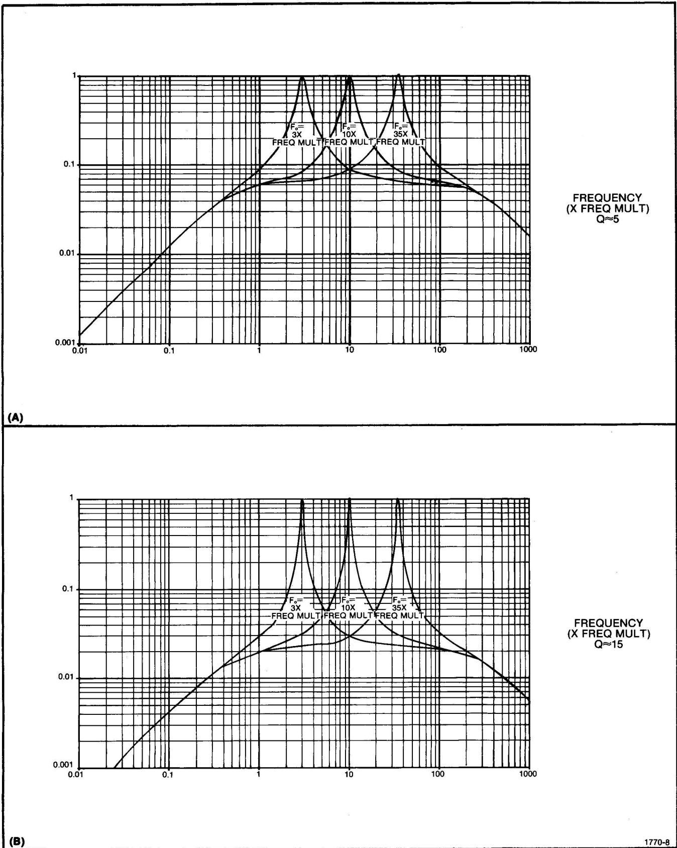
Fig. 2-1. Attenuation vs frequency (A) Q \approx 5 , (B) Q \approx 15 .
