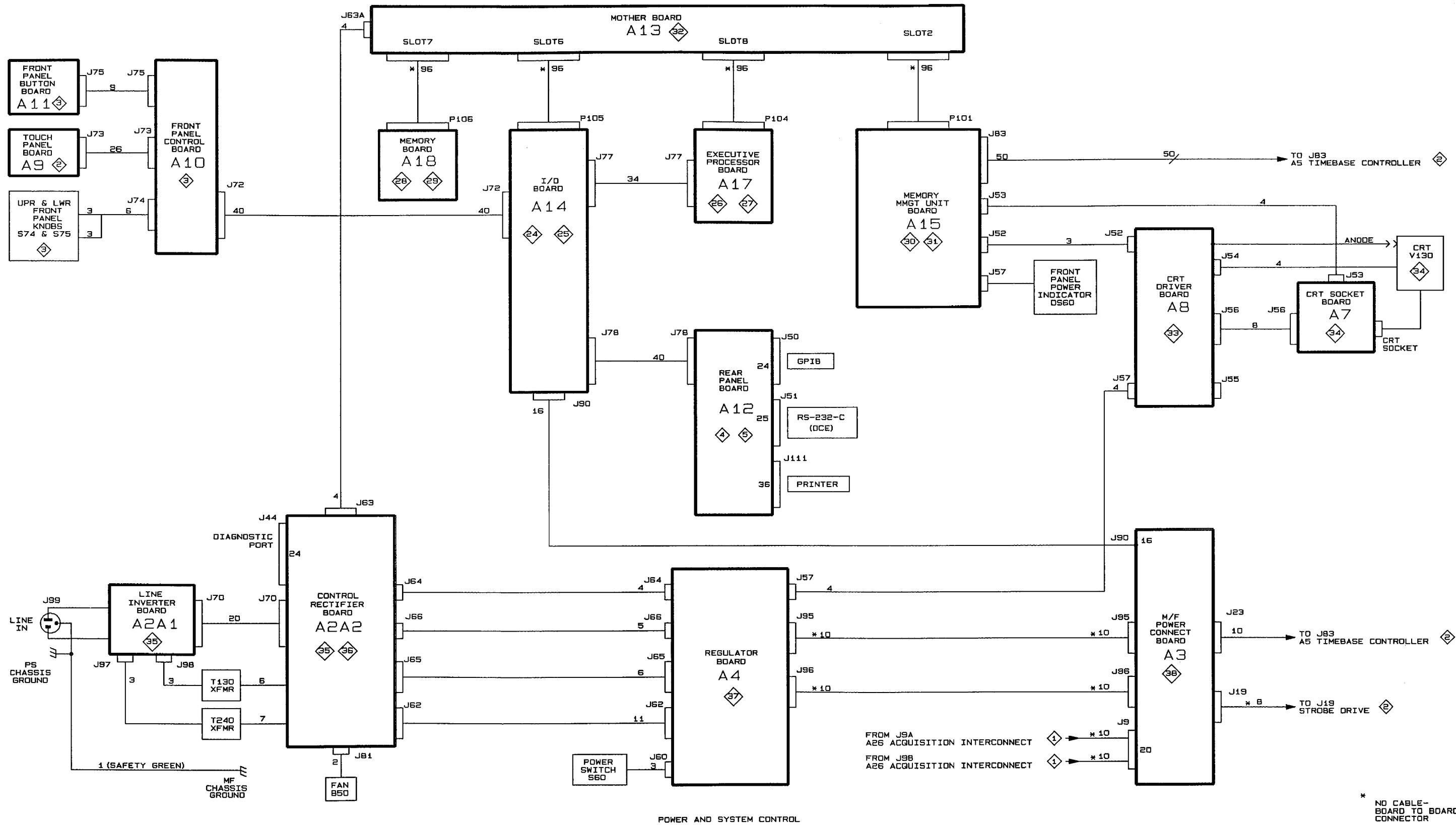
Figure 9-2: CSA 803A Detailed Block (Cabling) Diagram (Cont.)
