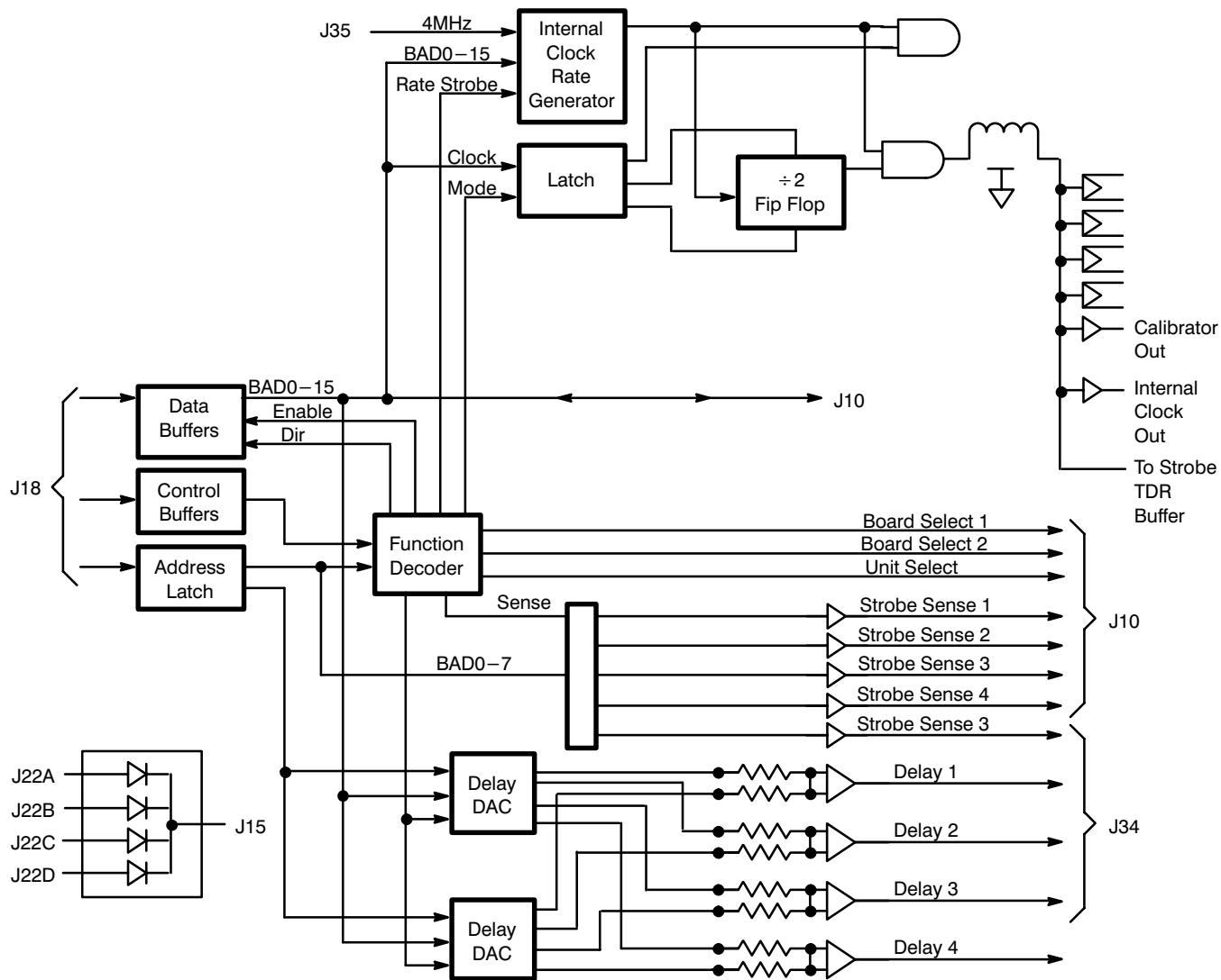
Figure 9-3: A1 M/F Strobe Drive Board Block Diagram
