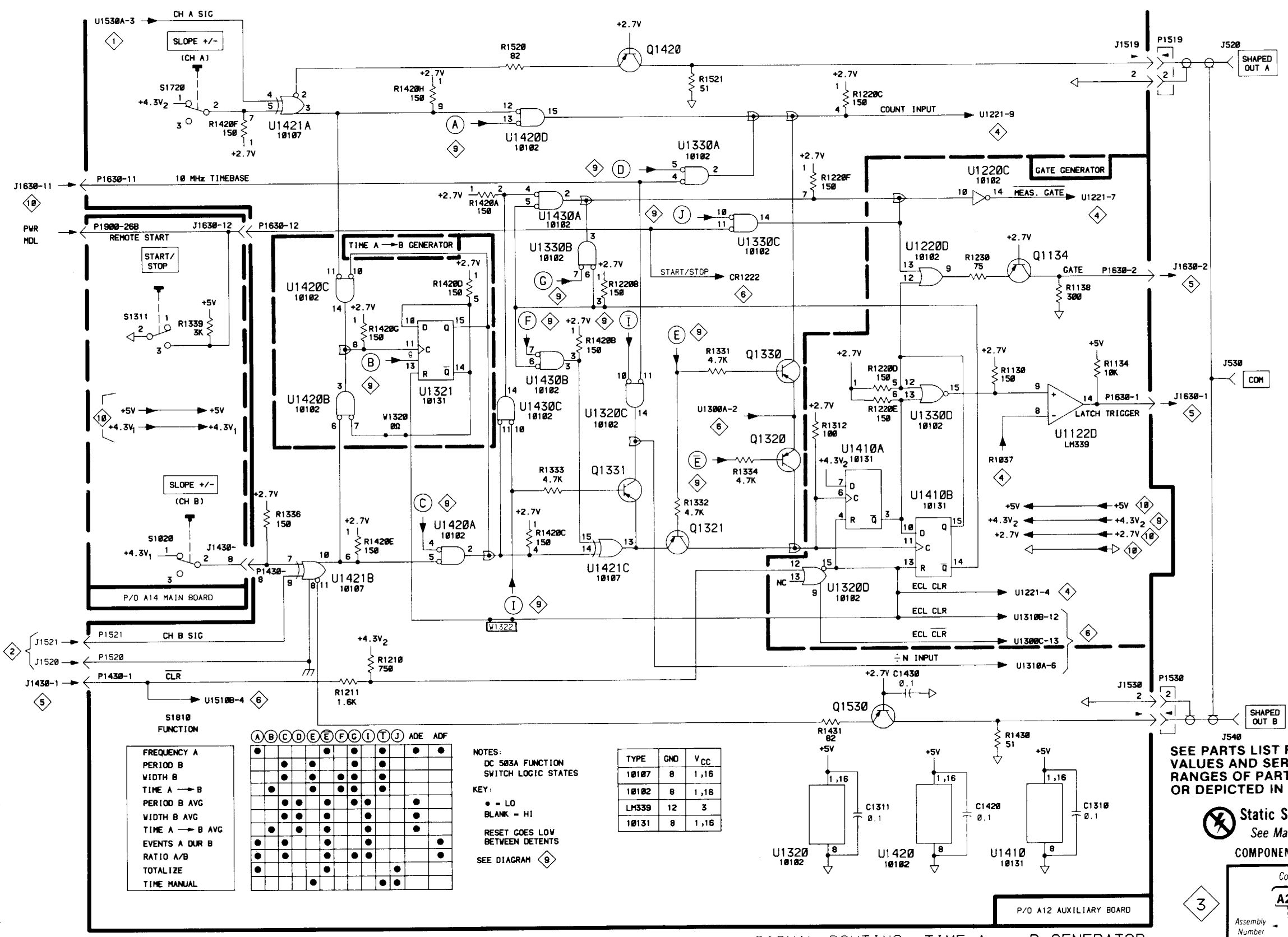
SIGNAL ROUTING, TIME A → B GENERATOR, & GATE GENERATOR
