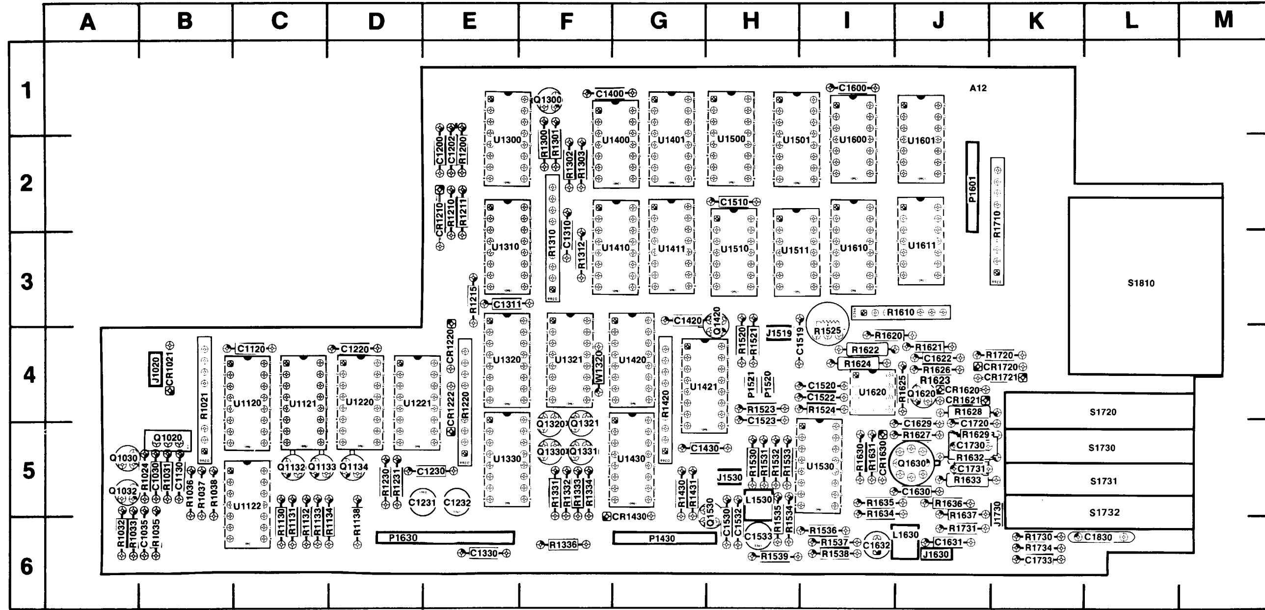
Fig. 8-3. Auxiliary Board (A12 Assy).
