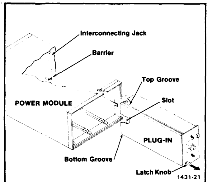
Fig. 2-1. Plug-in installation/removal.
