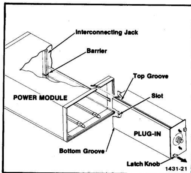
Fig. 2-1. Plug-in Installation/removal.
