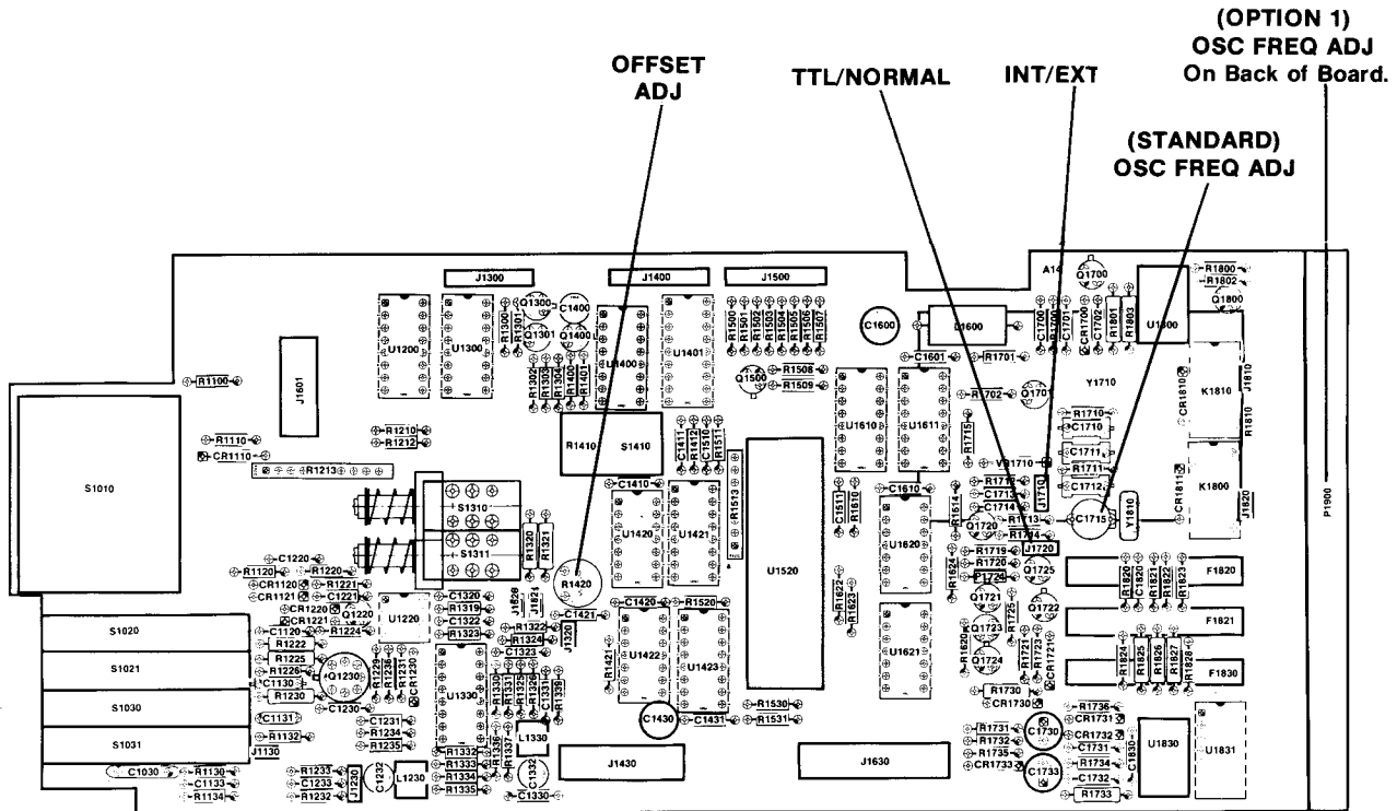
Fig. 8-1. Main Board (A14 Assy).
