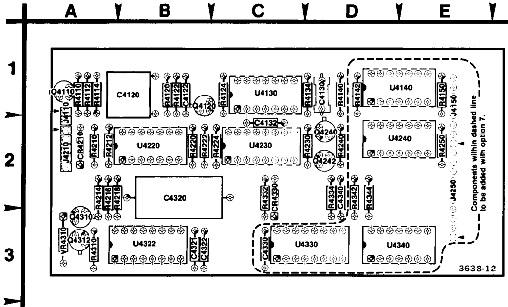
A2 Resolution Multiplier circuit board.
