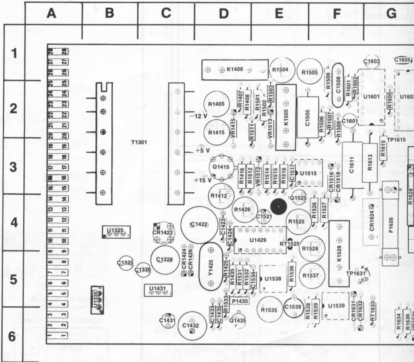
Fig. 8-14. Main Board (A10 Assy)
