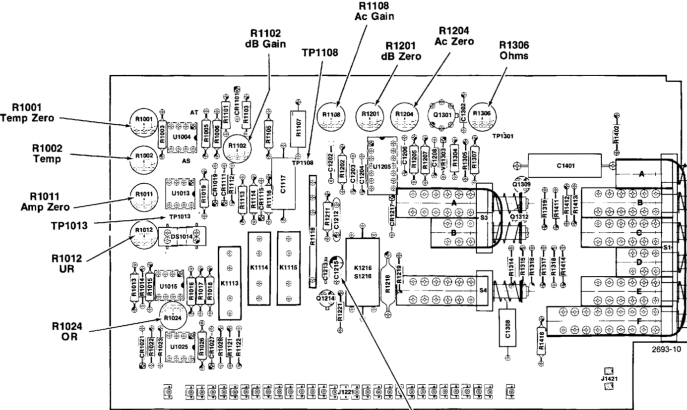
Fig. 8-4. Analog Board
