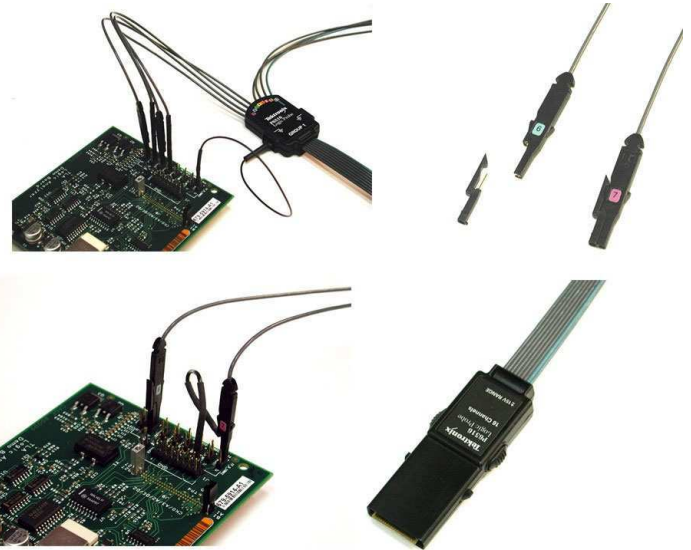
P6516 Mixed-signal Oscilloscope probe.
