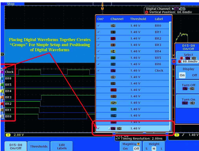
Groups are created by simply placing digital channels together on the screen. You can position and set threshold values for a group in a single step.
