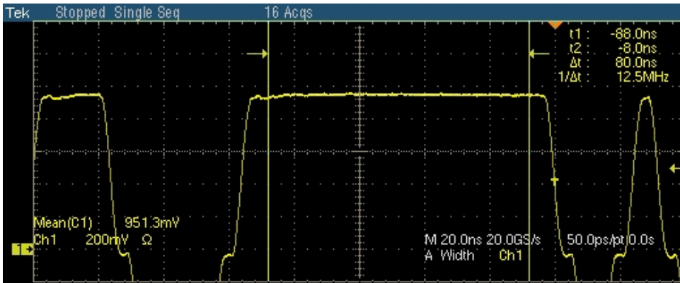
Figure 9-3: Waveform for 100BASE-TX Differential Output Voltage for Positive polarity
