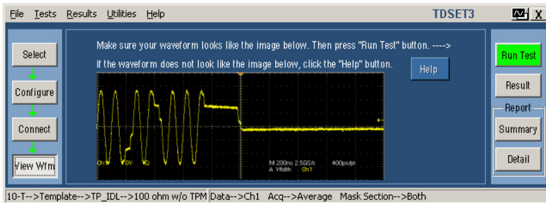
Figure 13-3: 10BASE-T View Waveform for TP_IDL
