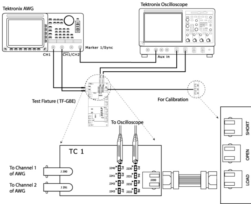
Figure 6-14: 1000BASE-T Connections for Return Loss Calibration
