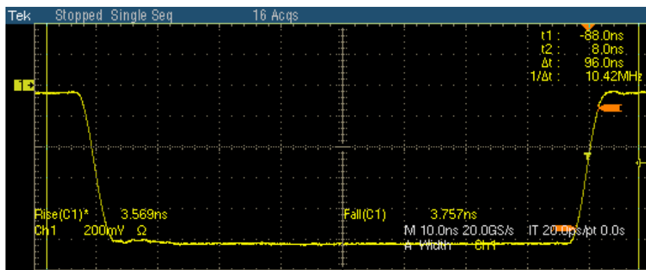
Figure 9-10: Waveform for 100BASE-TX Fall Time for Negative polarity
