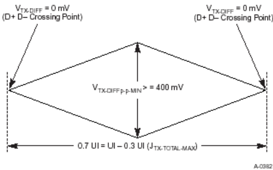
Figure 1b: Transmitter eye mask for low power variant where de-emphasis is not used
