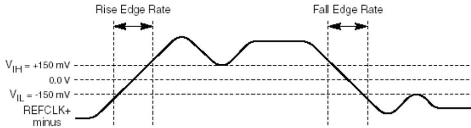
Figure 30: Ref Clock Rise/Fall time calculation
