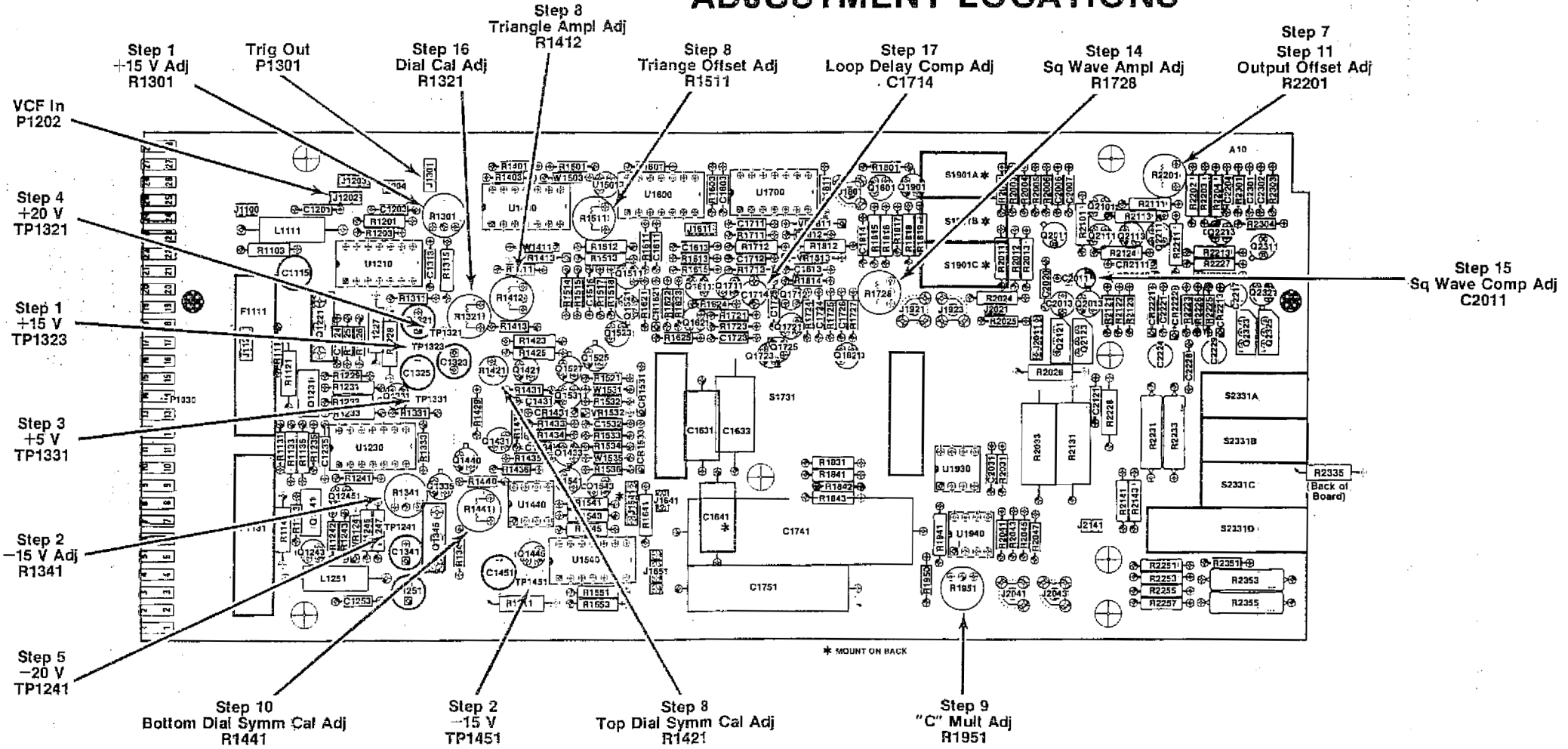
Fig. 8-2. Main Board.
