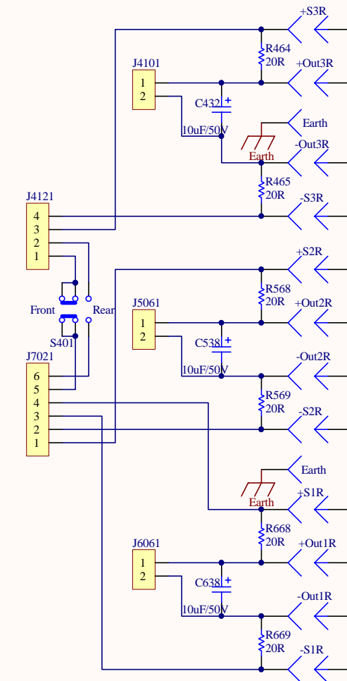
Front Terminal Board Supplies daughter board
