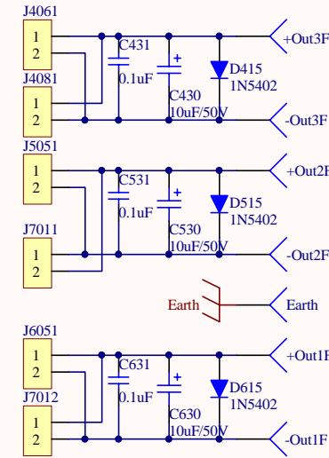
Front Terminal Board Supplies daughter board
