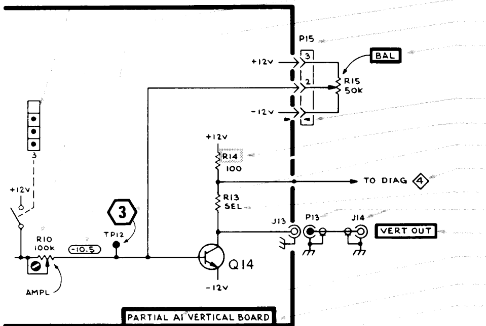
VERTICAL AMPLIFIER 2 CMD 1274
