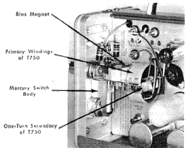
Fig. 4-2. Left front view of the Type 109 showing the pulser section.
