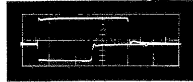
Vertical Deflection Factor: 9.5 v/cm Sweep Rate: 5 nsec/cm (Real-Time) Oscilloscope: Type 519
