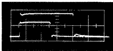
Vertical Deflection Factor: 9.5 v/cm Sweep Rate: 5 nsec/cm (Real-Time) Oscilloscope: Type 519
