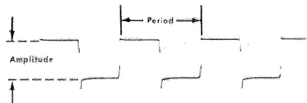
Fig. 6-5. Waveform measuring points.
