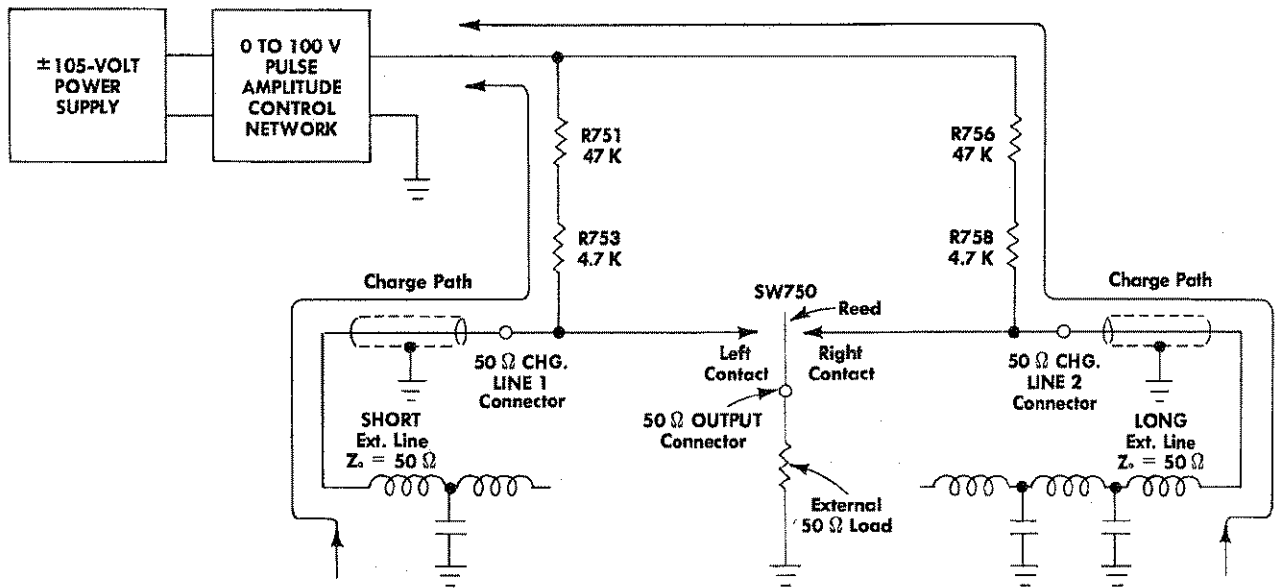
SIMPLIFIED CHARGE CIRCUIT (Using separate charge lines.)
