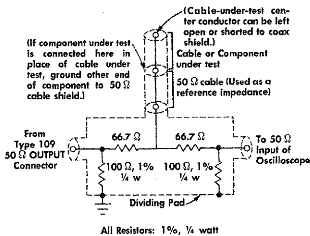
Fig. 3-5. Three-way dividing pad test circuit for measuring impedance by reflection.
