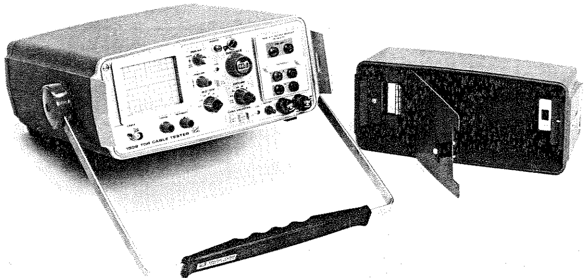
Fig. 2-1. 1502 TDR with Cover.
