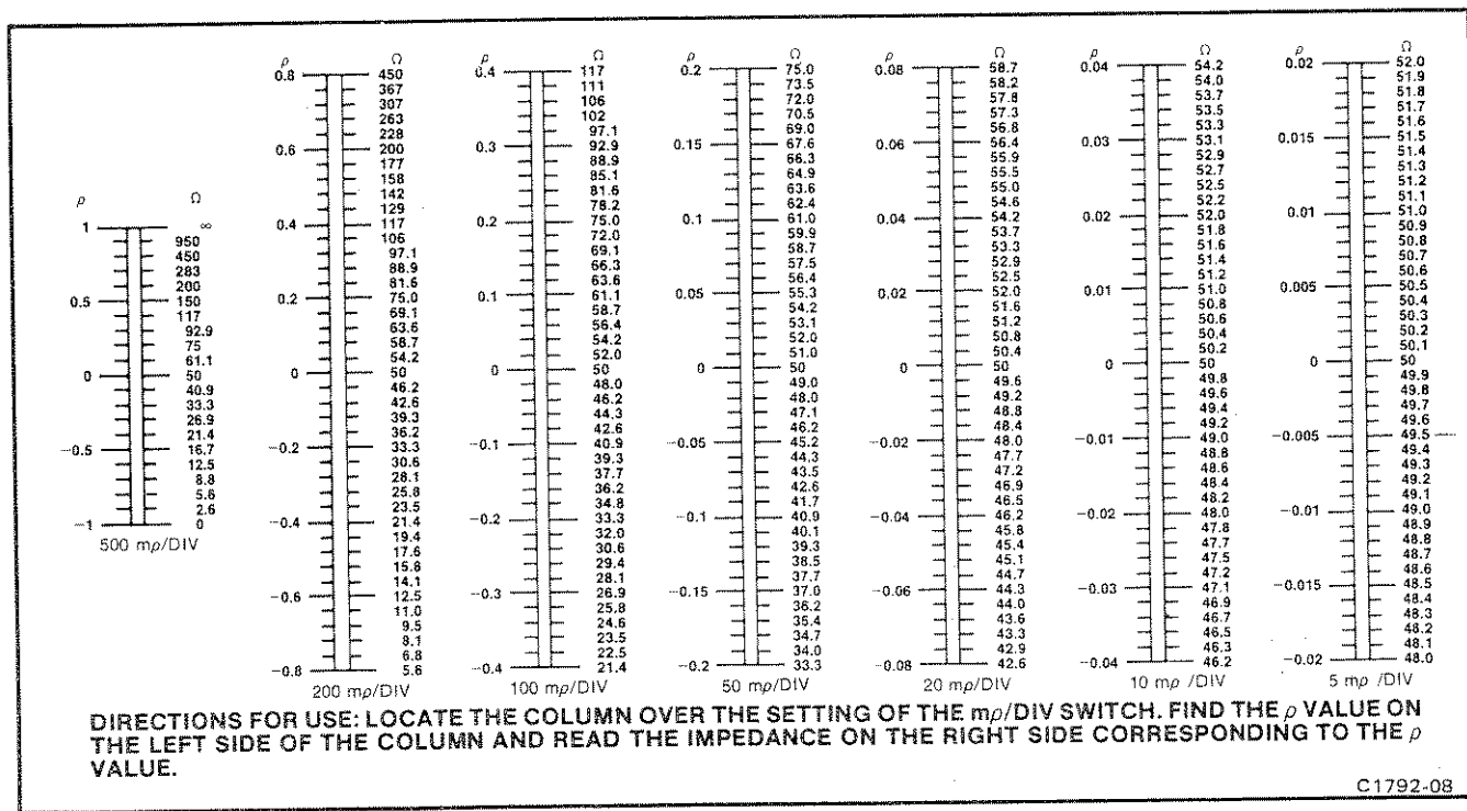
Fig. 2-7. Impedance Nomograph.
