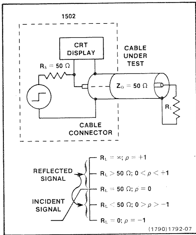
Fig. 2-6. TDR Display of R_L vs Z_0 .
