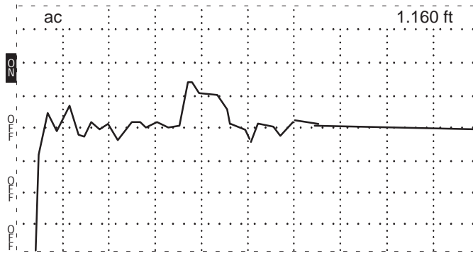
Figure 2-10: Rising Edge of Incident Pulse in Left-most Major Division
