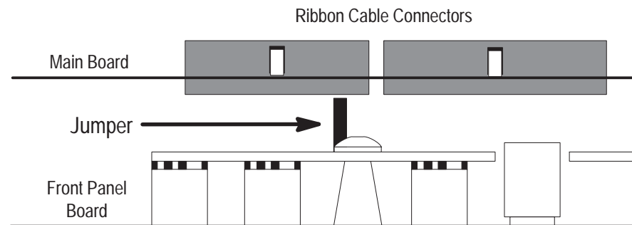
Figure 7-8: Location of Default Jumper on Front Panel Board
