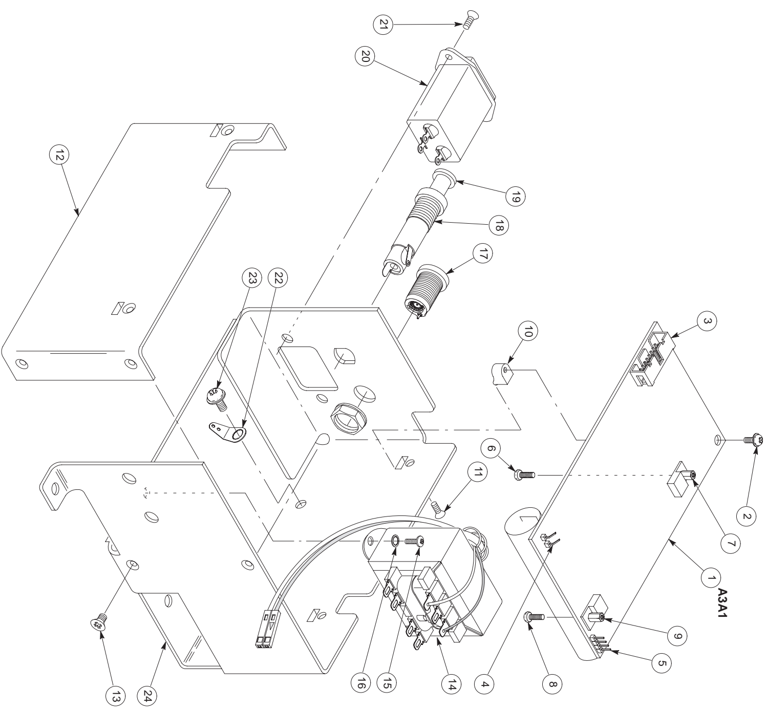
Figure 10-3: Power Supply
