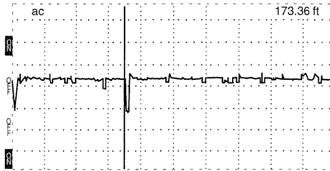
Figure 3-7: System 1 – Tap Quite Visible (128 avg, 50 ft/div, 35 dB)
