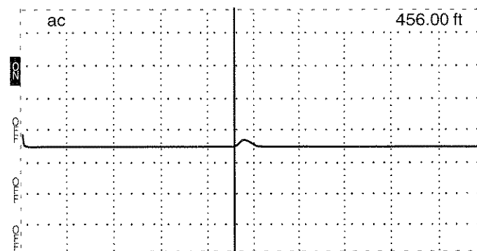
Figure 2-10: Pulse Width at 2 ns
