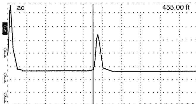
Figure 1-11: 455-ft Cable
