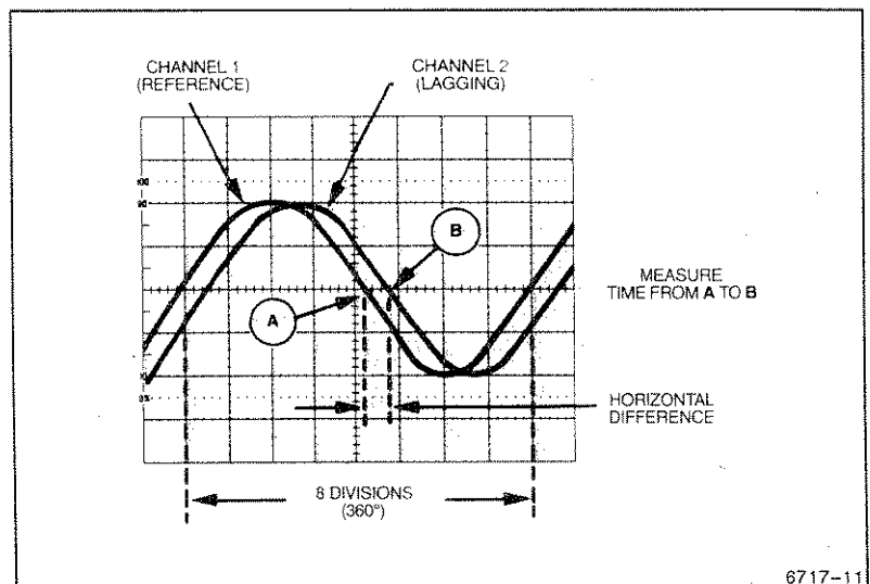
Figure 3-8. Phase difference.
