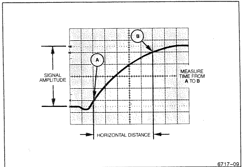
Figure 3-6. Measuring rise time.
