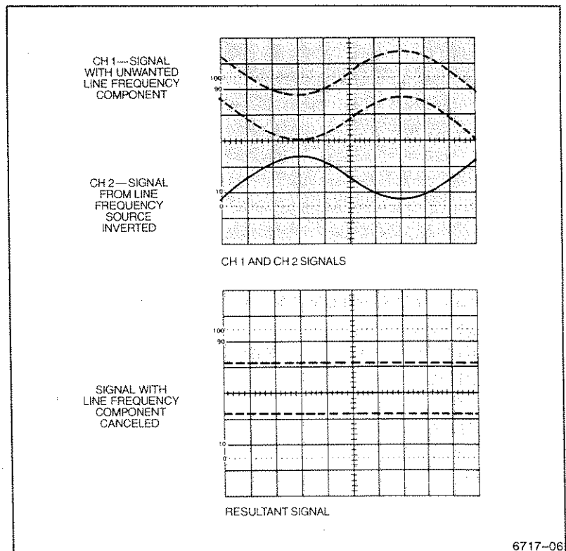
Figure 3-3. Common-mode rejection.
